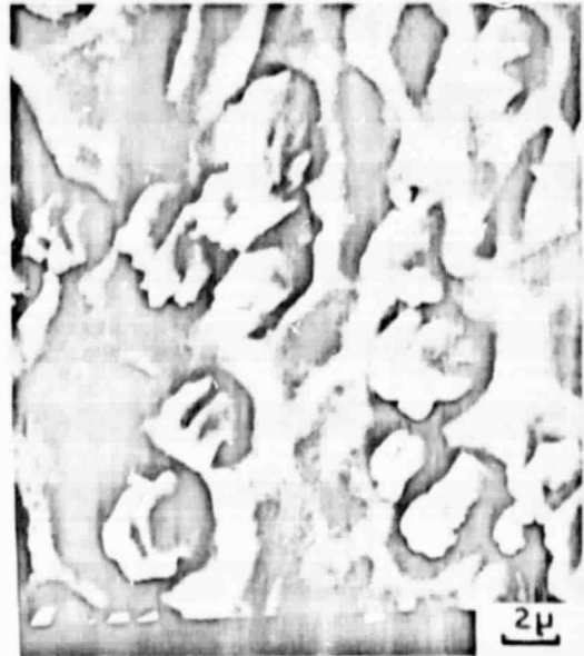
Fig. 12 a. Surface of copper after bombardment by ions with an energy of 1500 eV.
