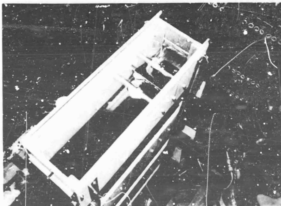
Figure 7. - Top view of the resin tank
