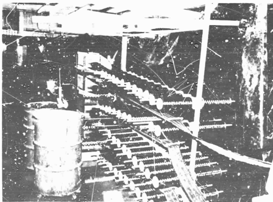
Figure 5. - Overall view of creel holding graphite fiber spools
