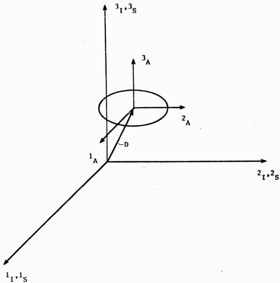
Figure 3.- Initial AMCD-spacecraft coordinate system alinement.
