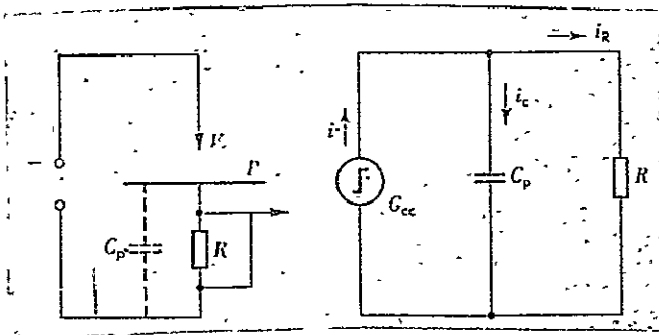
Fig. 2. Diagram of a point-plate system with a constant current generator.
