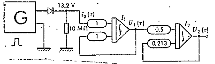
Fig. 6. Analog computer simulation diagram of measurement circuits with rectangular pulses passing through them.
