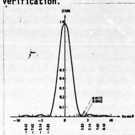
Figure 4. Normalized airy ring diffraction intensity pattern.
