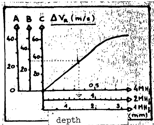
Figure 9: Calibration Curves
