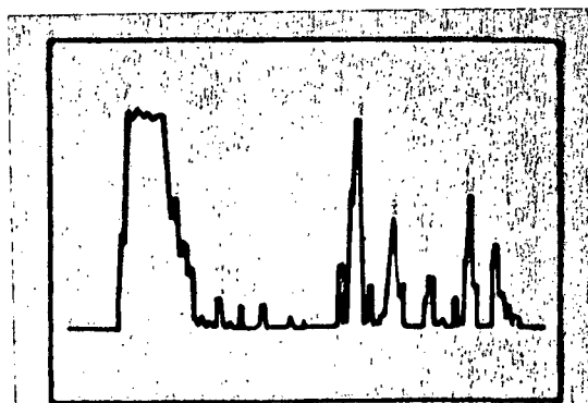
Figure 3: Oscillogram obtained for a piece tempered to a depth of 10 mm.
