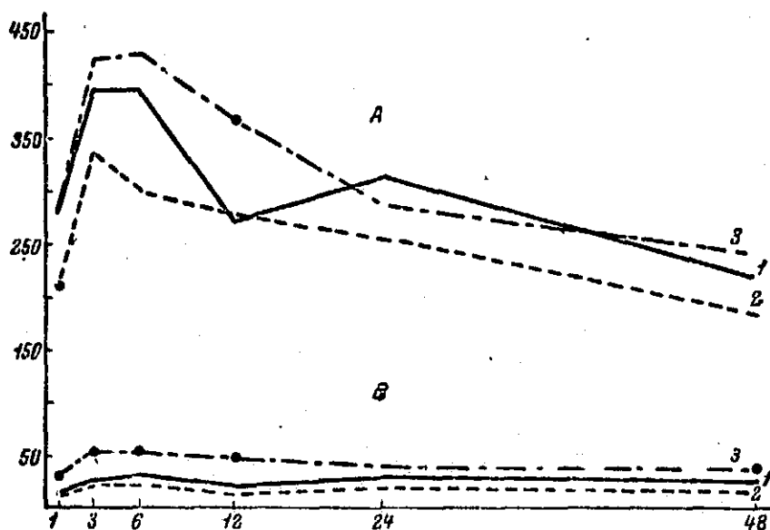
Fig. 2. Rate of incorporation of radioactive ^{14}\text{C} amino acids in tissue proteins of kidneys (A) and skeletal muscles (B) of rats under various motor activity conditions; designations same as in Fig. 1.
