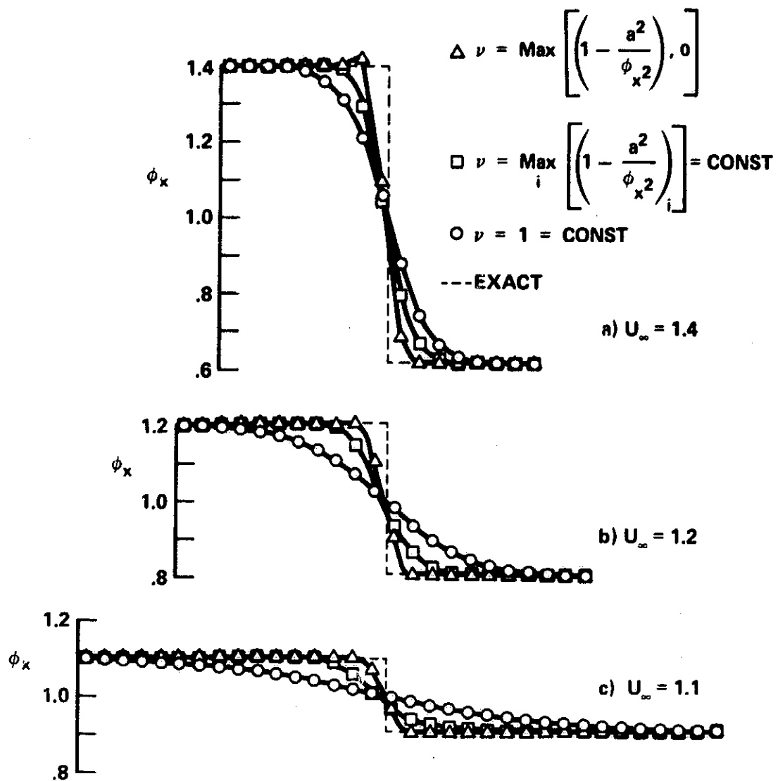
Figure 2.- Shock profiles, \phi_x vs x .
