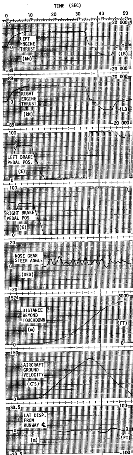
FIGURE 6-10 TYPICAL WET RTO, BRAKES AND REVERSERS, DIGITAL ANTISKID, PILOT - WIEBRACHT, RUN-L17
