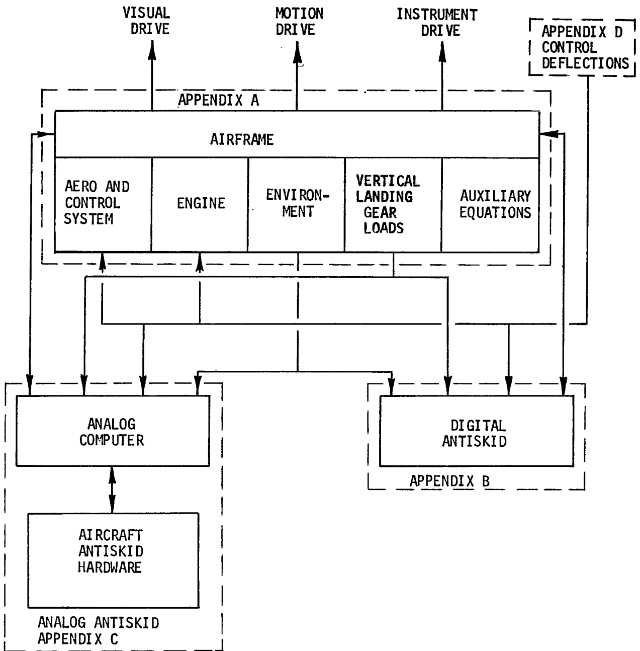
FIGURE 4-2 SIMULATOR DETAILS
