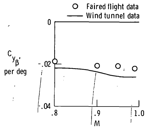
(c) C_{y_{\beta}} .
