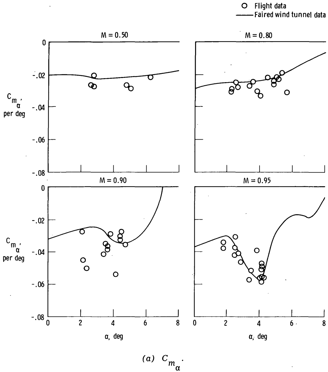
Figure 5. Variation of longitudinal derivatives with angle of attack.
