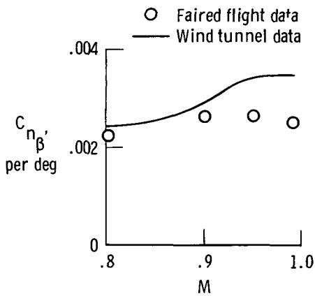
(b) C_{n_{\beta}} .
