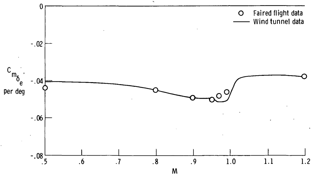
(b) C_{m_{\delta_e}}
