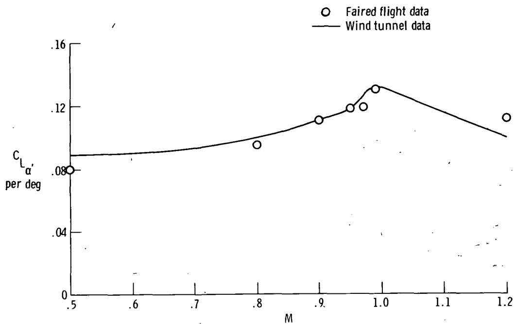
(c) C_{L_{\alpha}}
