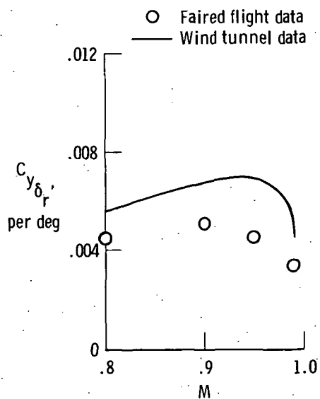
(f) C_{y\delta_r}'
