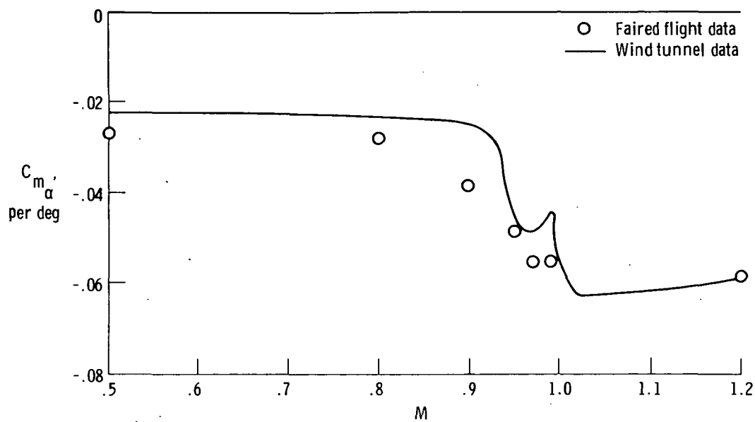
(a) C_{m_{\alpha}}
