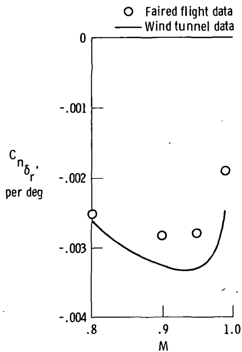
(e) C_{n\delta_r}'
