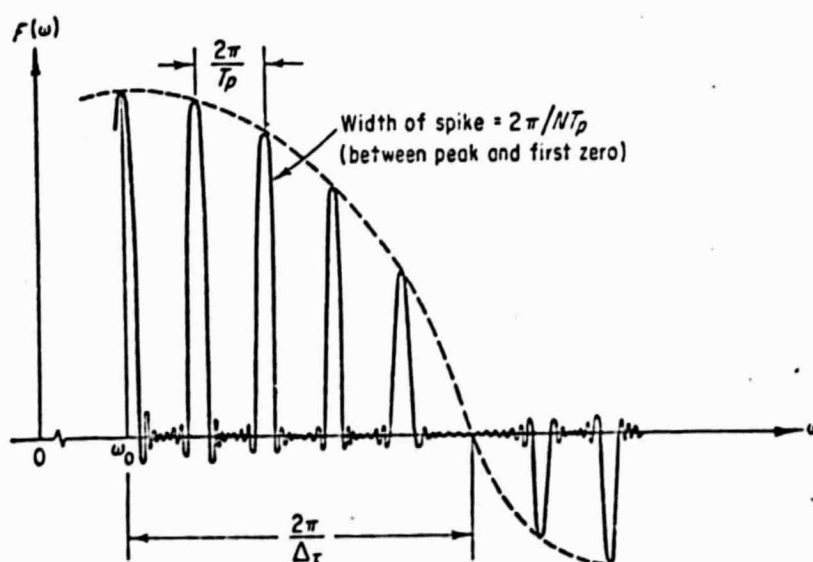
Figure 6. Fourier transform of pulse train.
