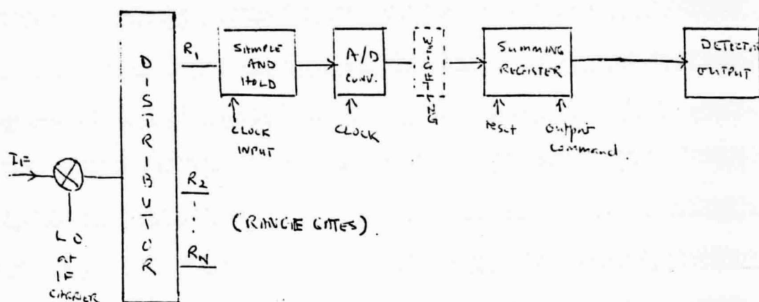
Figure 9. Unfocussed sampling processor.
