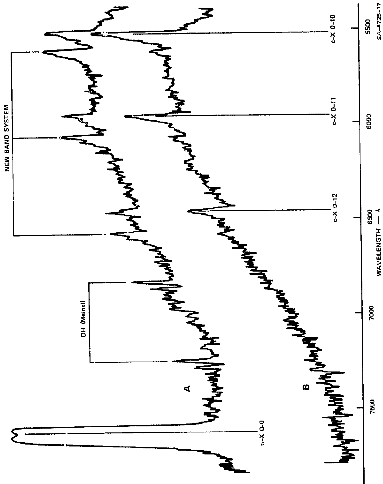
Figure 1 Microdensitometer traces of afterglow spectrum, fast-flow system, 20 torr He, 30 mtorr O 2 , wavelength range 5300-8000 Å. A. No CO 2 . B. 7 torr CO 2 .
