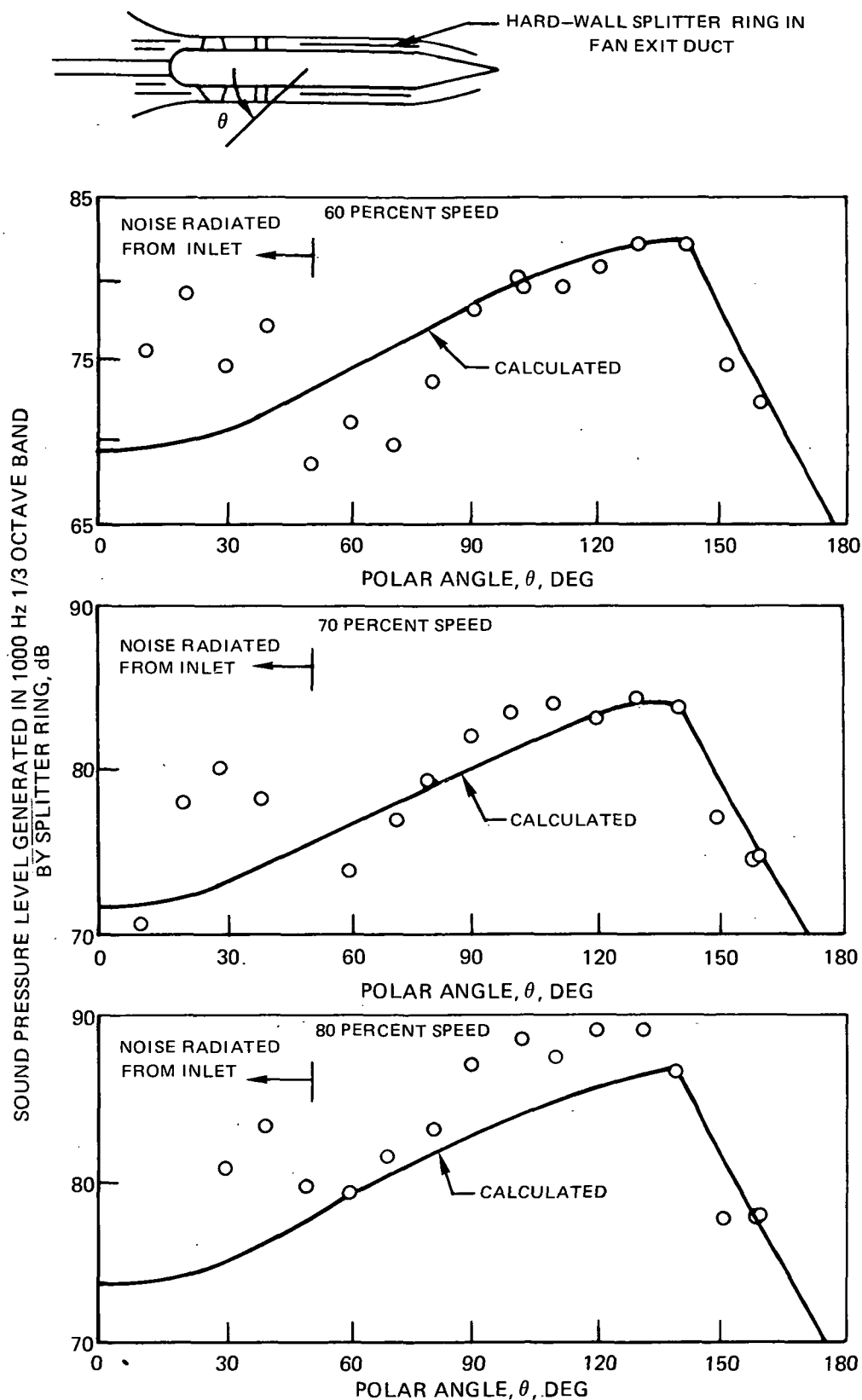
FIGURE 15 – MEASURED AND CALCULATED DIRECTIVITY OF NOISE GENERATED BY HARD-WALL FAN EXIT DUCT SPLITTER RING
