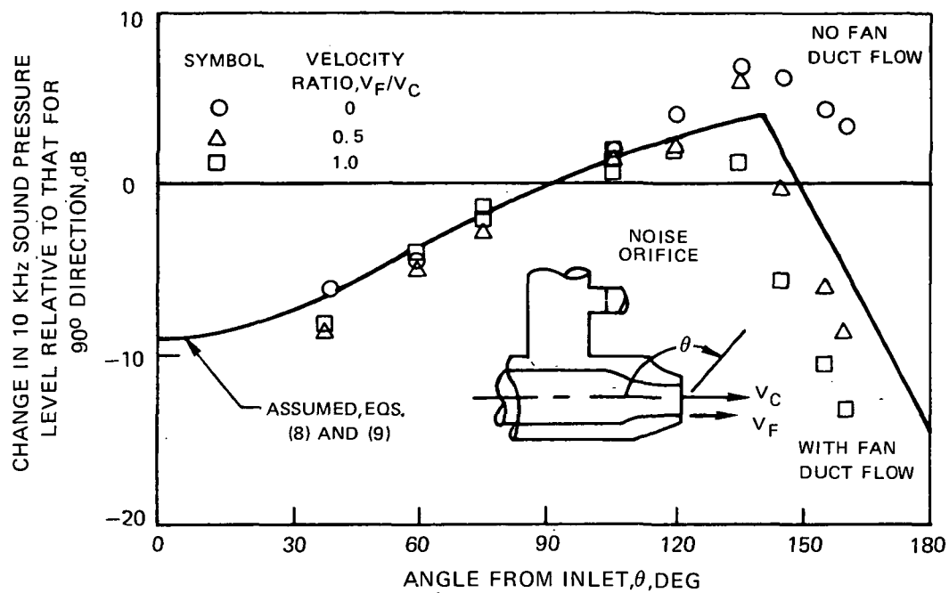
(a.) DIRECTIVITY OF NOISE INTRODUCED INTO FAN DUCT
