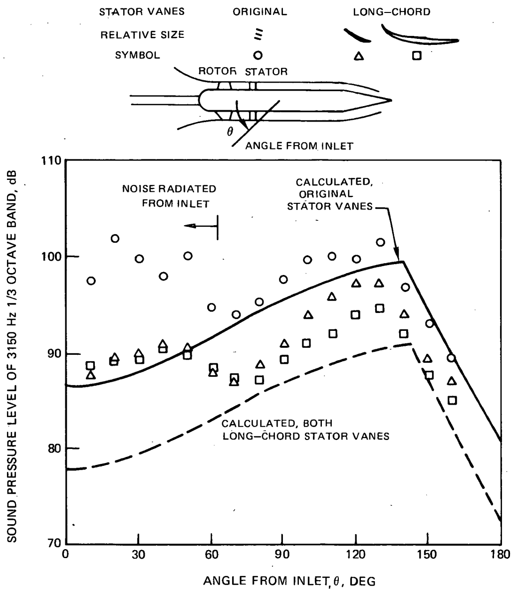
FIGURE 20— EFFECT OF LONG-CHORD STATOR VANES ON FULL-SCALE FAN NOISE DIRECTIVITY IN 3150 Hz 1/3 OCTAVE BAND AT 80 PERCENT SPEED
