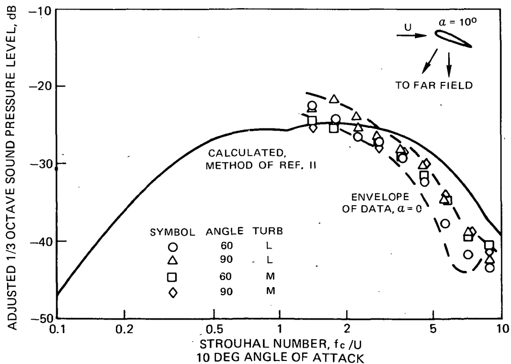
FIGURE 5 —MEASURED AND CALCULATED ADJUSTED SPECTRA FOR SMALL THIN AIRFOIL IN TURBULENT FLOW, (a) 31.5 M/SEC VELOCITY
