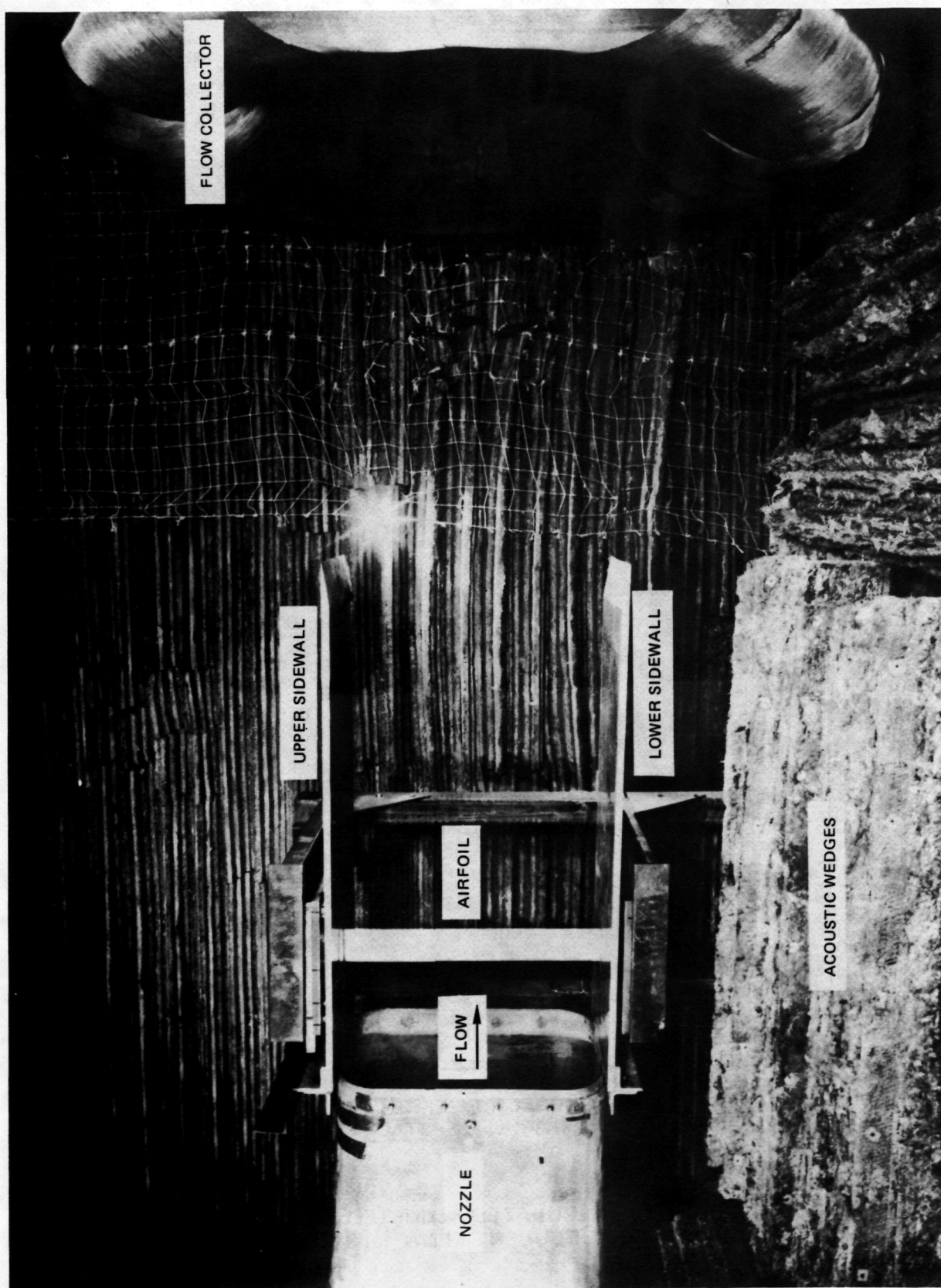
FIGURE 4 – ACOUSTIC TUNNEL TEST SECTION WITH 11.4 CM (4.5 IN.) CHORD AIRFOIL
