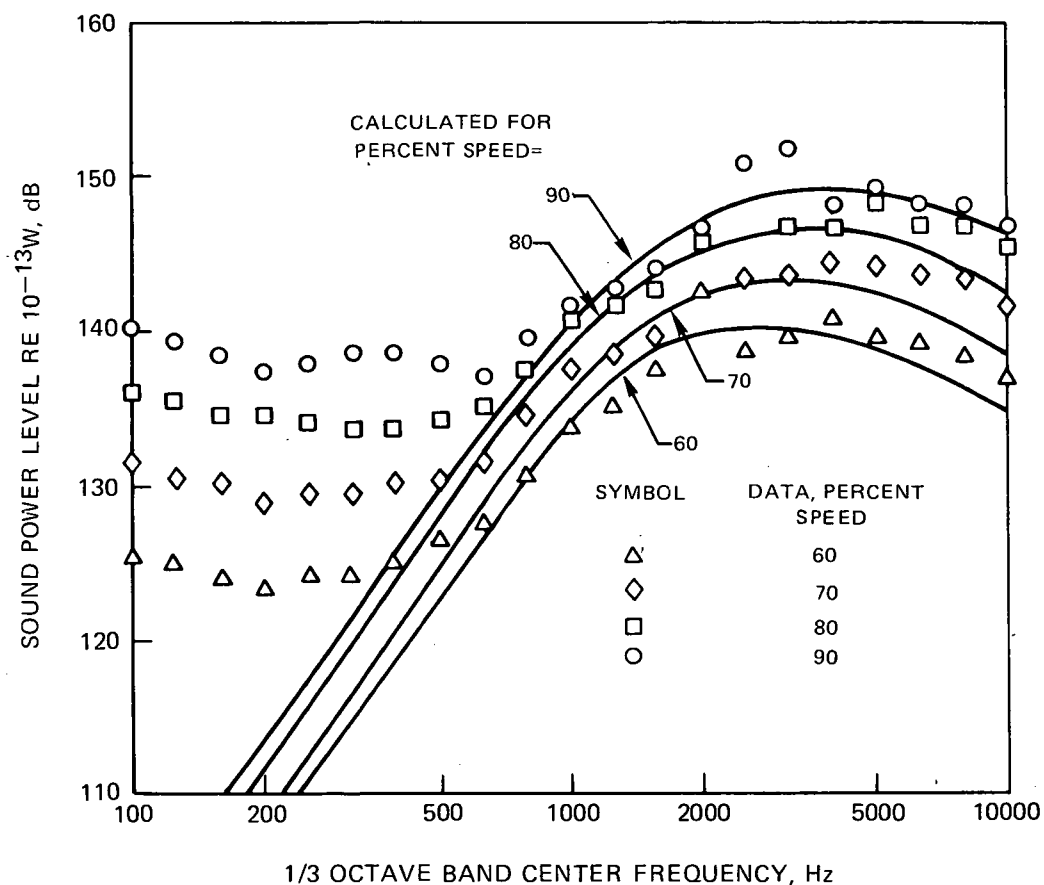
FIGURE 17— CALCULATED AND MEASURED 1/3 OCTAVE SOUND POWER SPECTRA OF FULL SCALE FAN NOISE FOR ORIGINAL STATOR VANES. ASSUMED TURBULENCE PROPERTIES VARIED TO ACHIEVE GOOD MATCH WITH DATA
