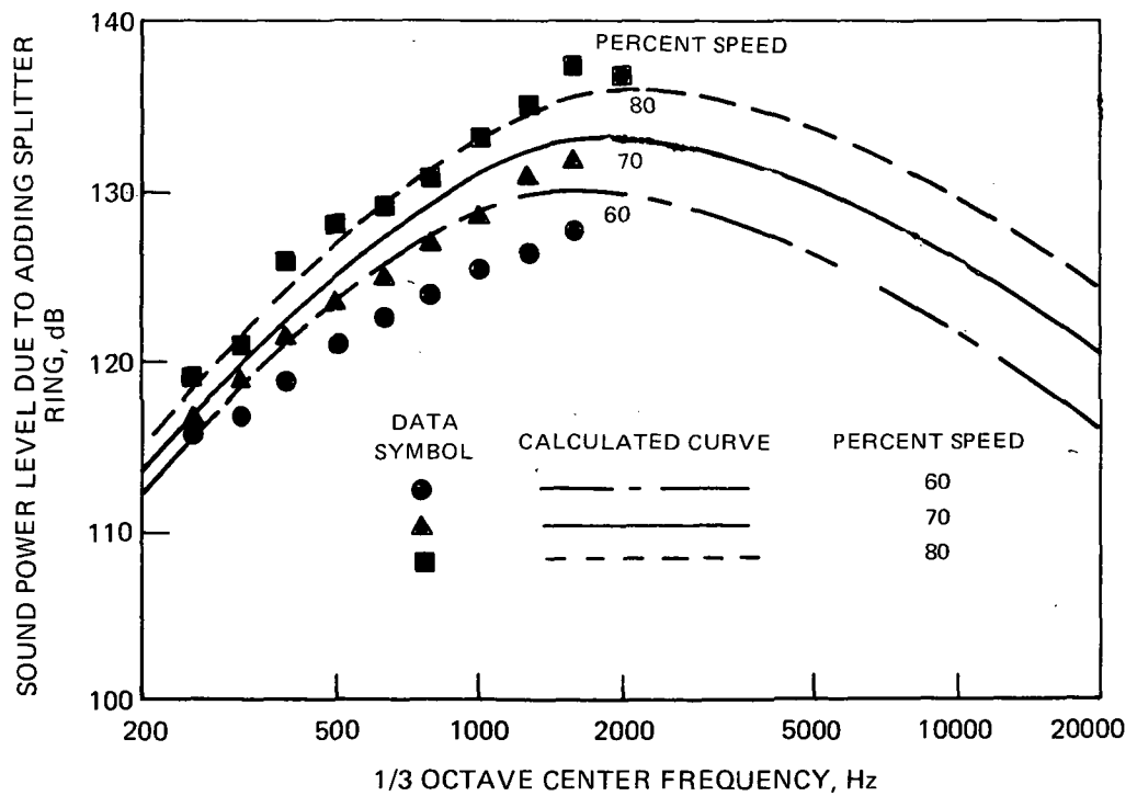
FIGURE 16— MEASURED AND CALCULATED SOUND POWER LEVEL DUE TO ADDITION OF HARD-WALL AFT SPLITTER RING
