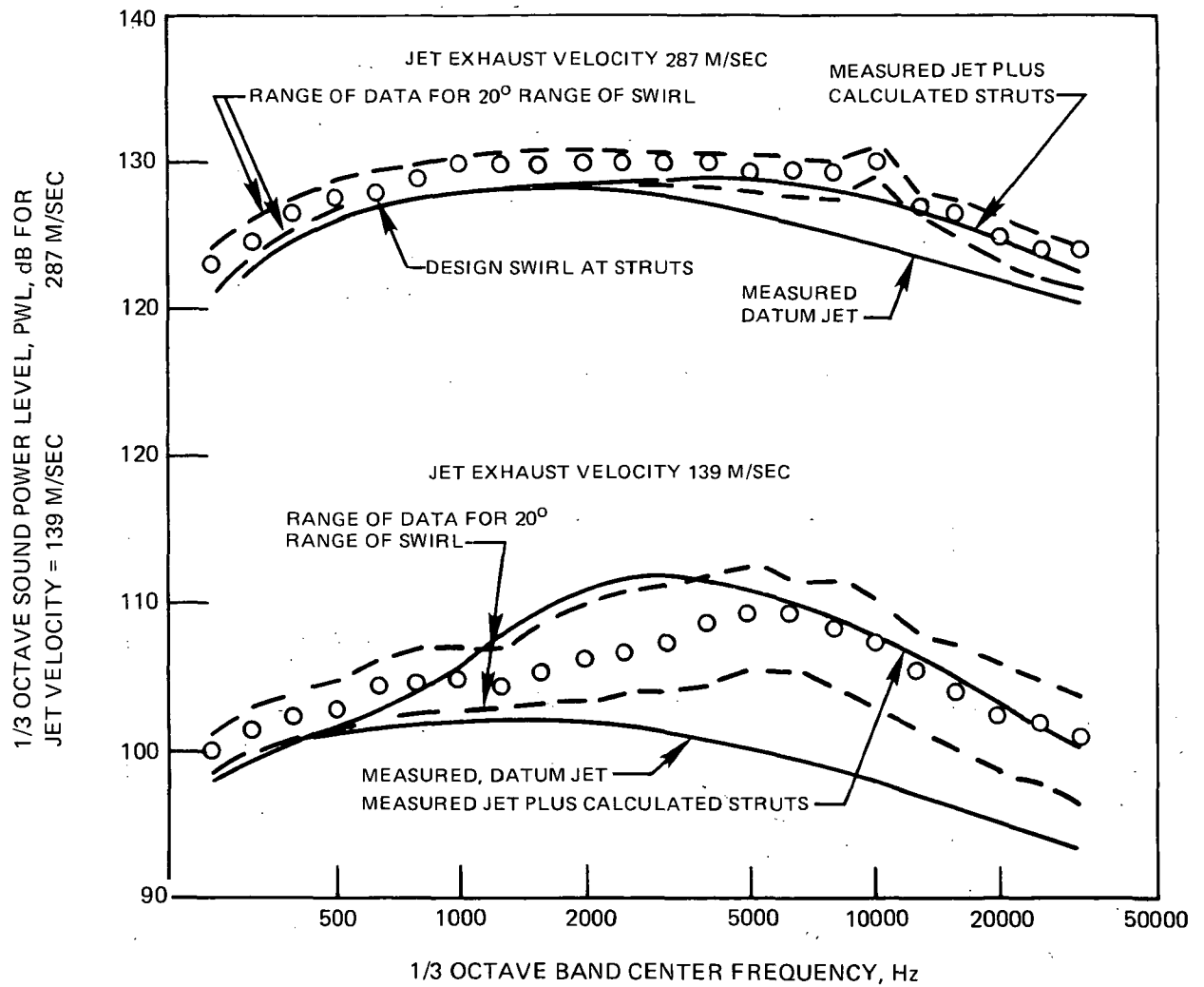
FIGURE 13—CALCULATED AND MEASURED NOISE OF TURBINE EXIT STRUTS IN 1/8 SCALE MODEL TURBOJET ENGINE
