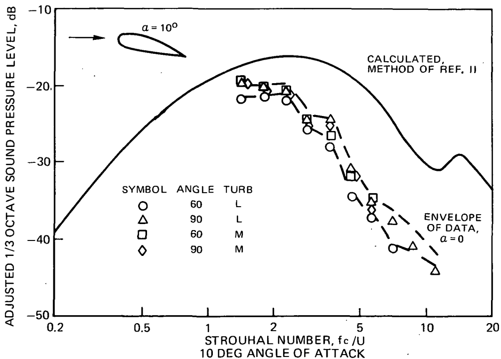
FIGURE 6 —MEASURED AND CALCULATED ADJUSTED SPECTRA FOR THICK AIRFOIL IN TURBULENT FLOW. (a) 31.5 M/SEC VELOCITY
