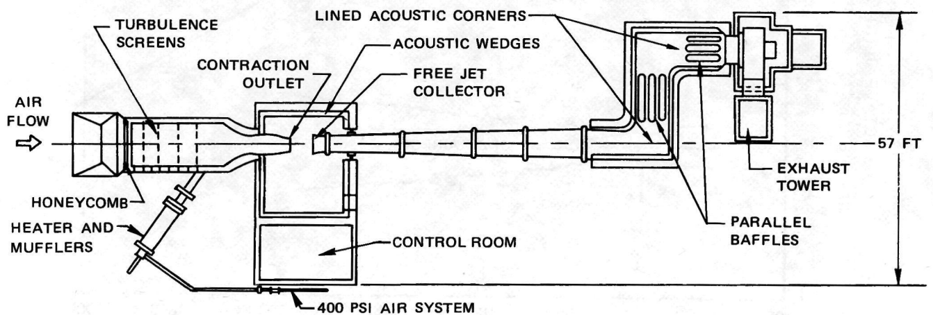
TOP VIEW
