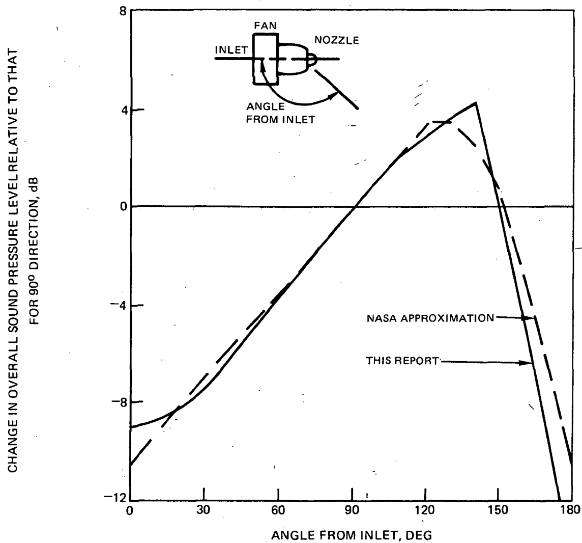
FIGURE 11 — COMPARISON OF ASSUMED DIRECTIVITY SHAPES FOR AFT-RADIATED INTERNALLY GENERATED NOISE
