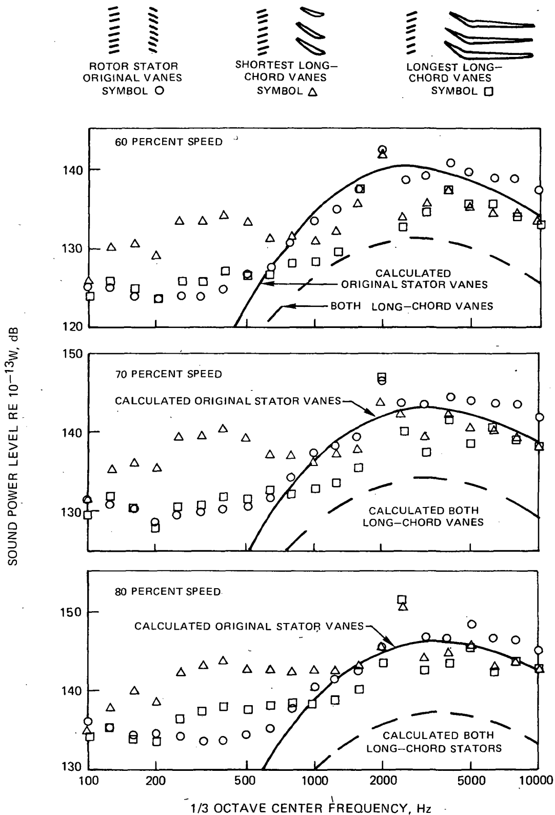
FIGURE 18 — COMPARISON OF CALCULATED AND MEASURED 1/3 OCTAVE SOUND POWER SPECTRA OF FULL SCALE FAN WITH ORIGINAL AND LONG-CHORD STATOR VANES AT 60, 70, AND 80 PERCENT SPEED
