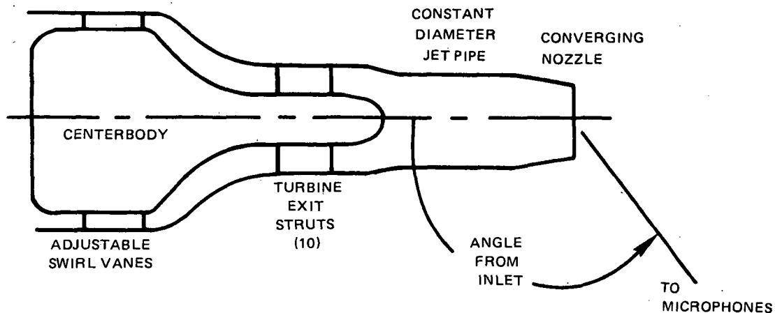
(a) SKETCH OF ENGINE EXHAUST SYSTEM MODEL
