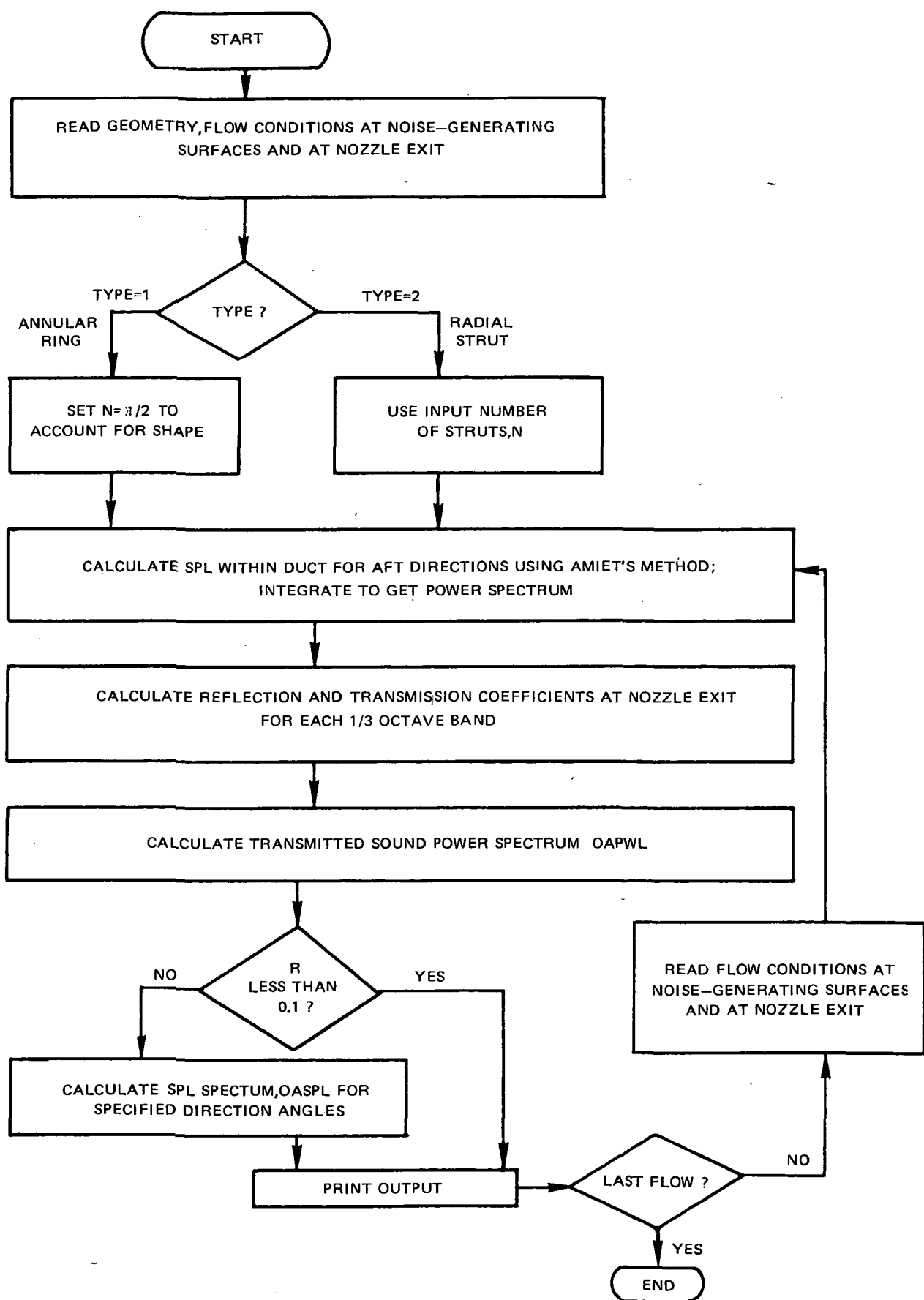
FIGURE 21—FLOW CHART FOR CALCULATION OF STRUT NOISE RADIATED FROM EXIT DUCT
