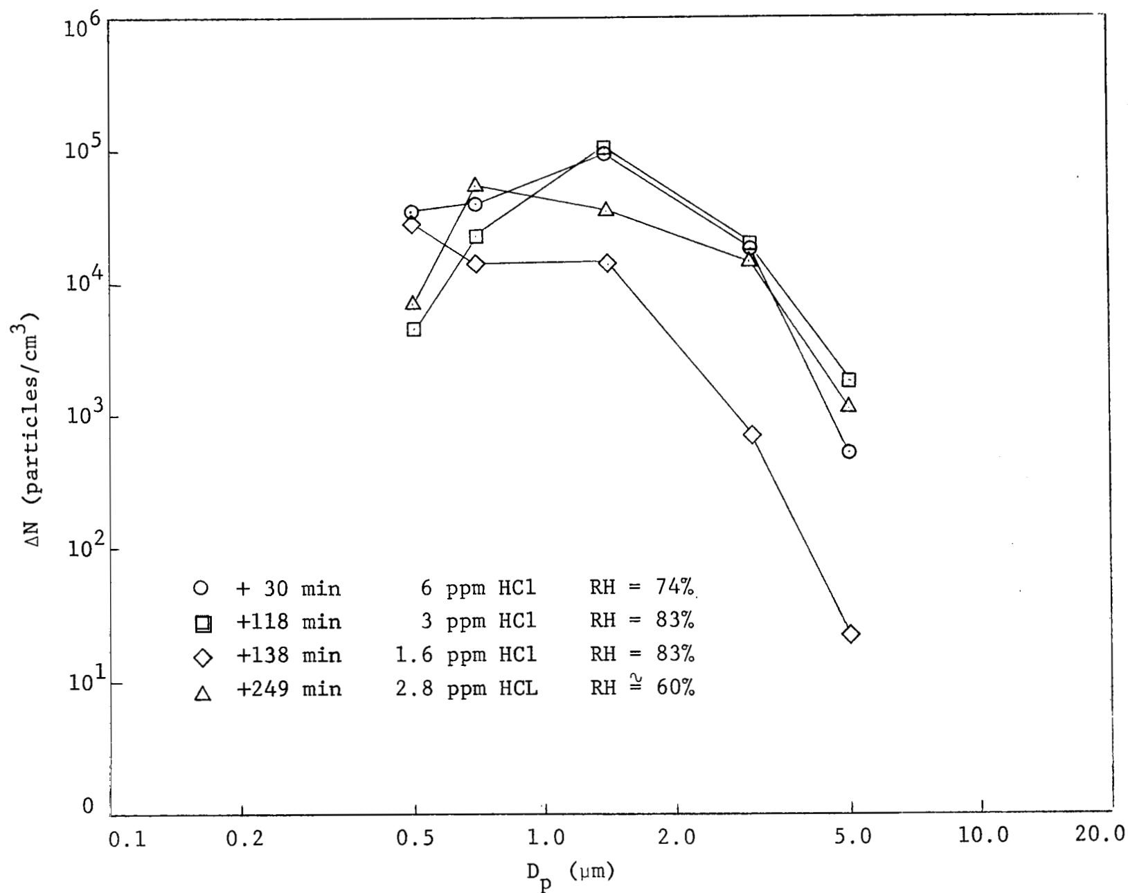
Figure 24 Al 2 O 3 PARTICLE SIZE DATA FOR THIRD SCAVENGING TEST
