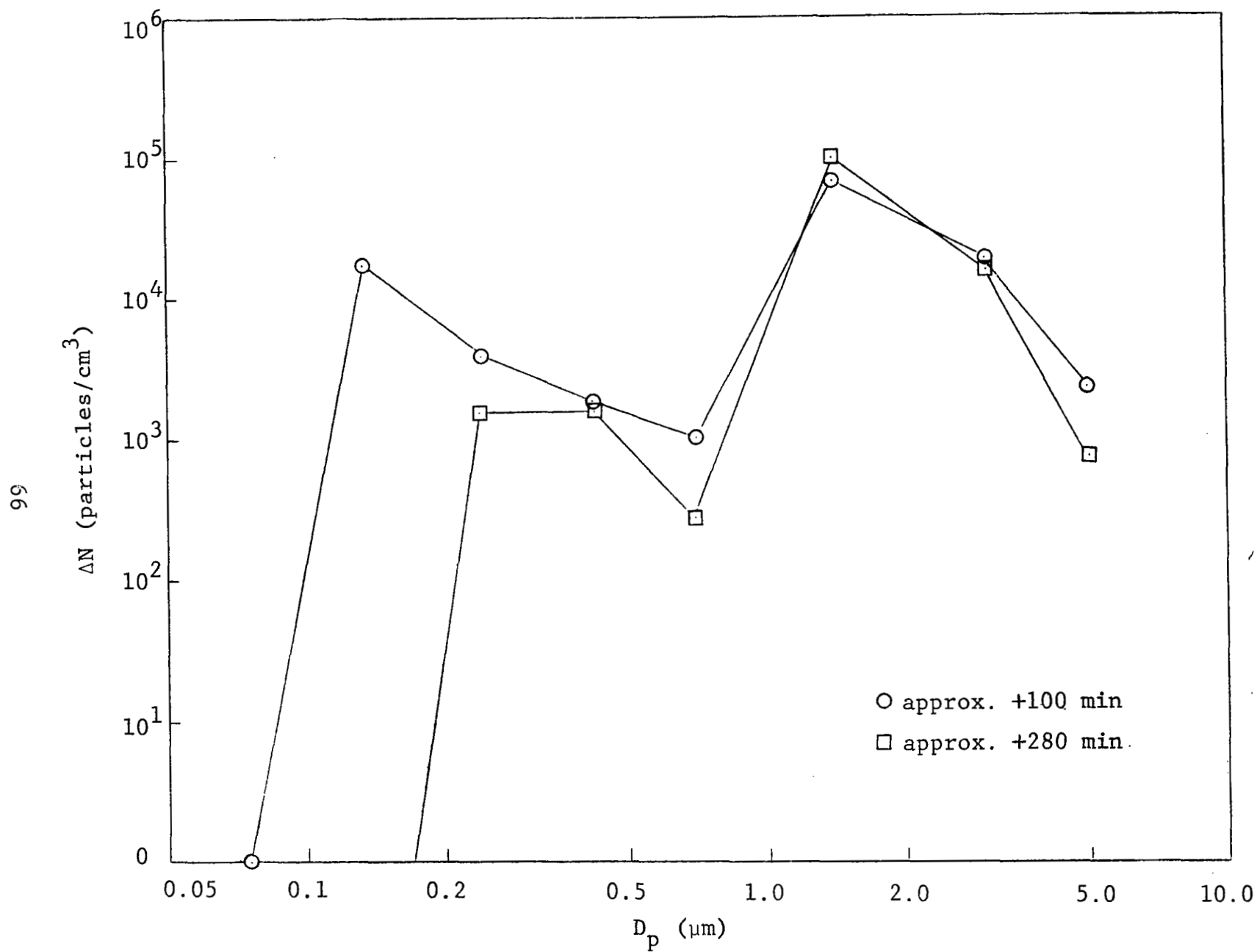
Figure 23 \text{Al}_2\text{O}_3 PARTICLE SIZE DATA FOR SECOND SCAVENGING TEST
