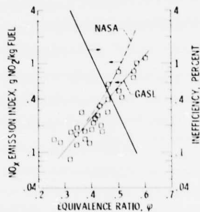
Figure 8. - Effect of equivalence ratio on \text{NO}_x in a prevaporized-premixed combustion scheme. Jet A fuel; residence time, 2 milliseconds; inlet temperature, 830 K; inlet pressure, 40 N/cm 2 .
