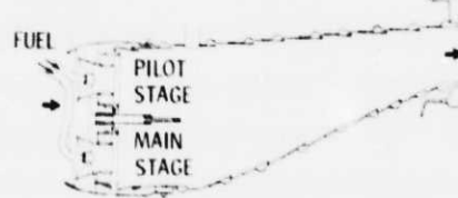
(b) DOUBLE ANNULAR CONCEPT.
