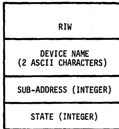
Figure 5.5-22 Declare DPA End-Item OP/NOP Record
