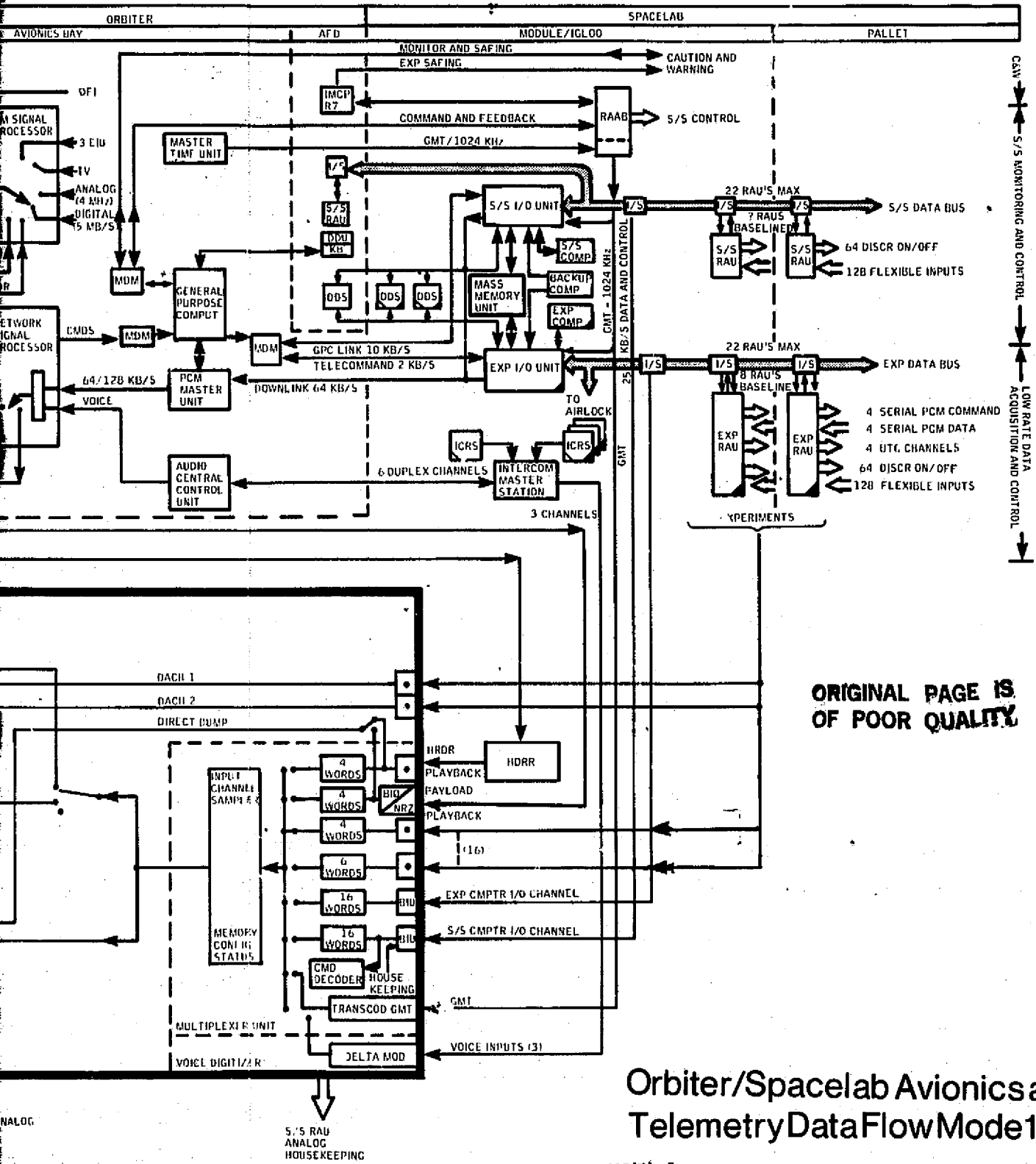
Figure 4-1 Mode 1 Telemetry Data Flow Paths from Orbiter to Ground (Spacelab Configuration)
