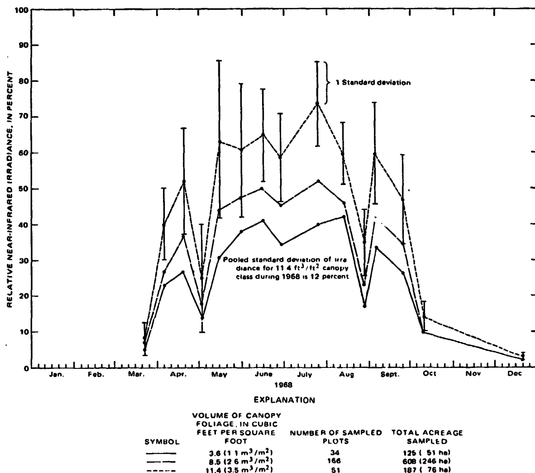
FIGURE 27.—Relative near-infrared irradiance versus time for three saltcedar volumes of canopy foliage classes, reach 2, Gila River Phreatophyte Project.
