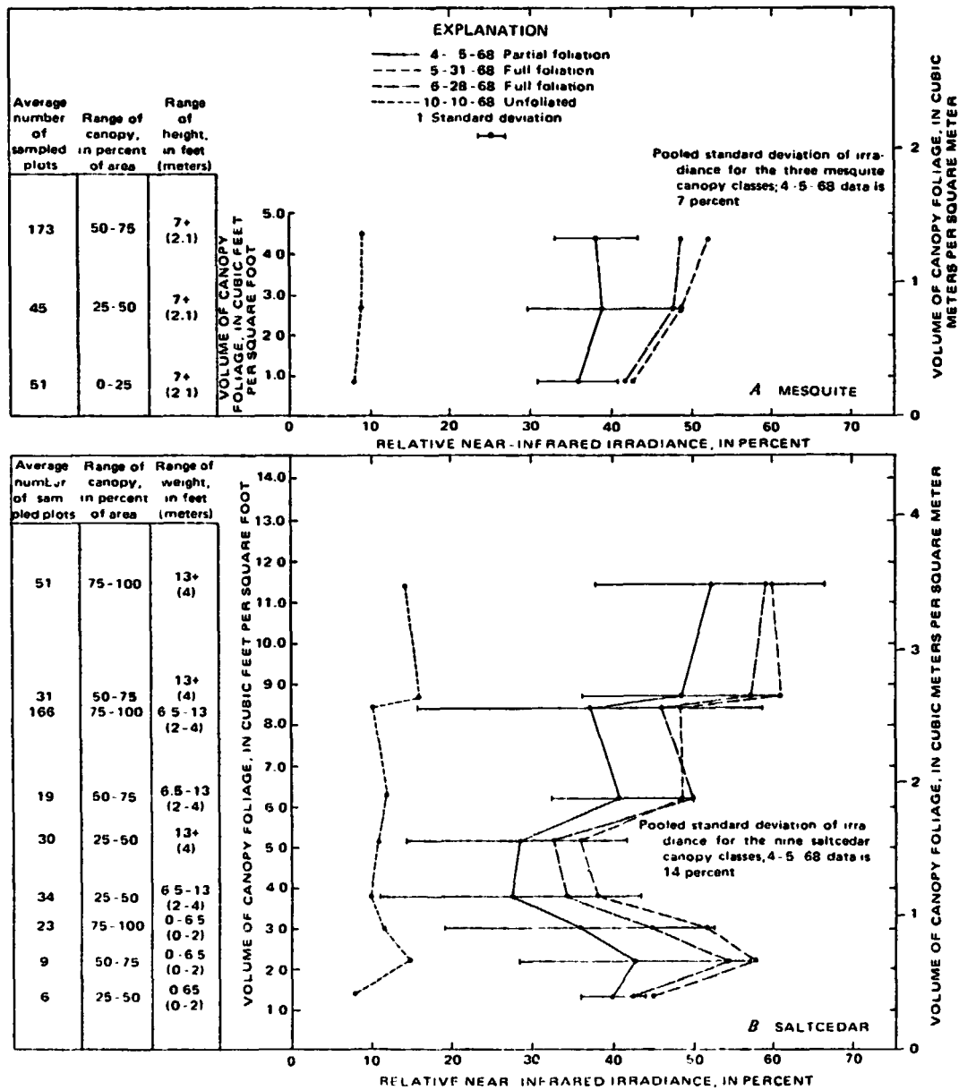
FIGURE 26 -- Volume of canopy foliage versus relative near-infrared irradiance for photographic flights during 1968, reach 2, Gila River Phreatophyte Project.
