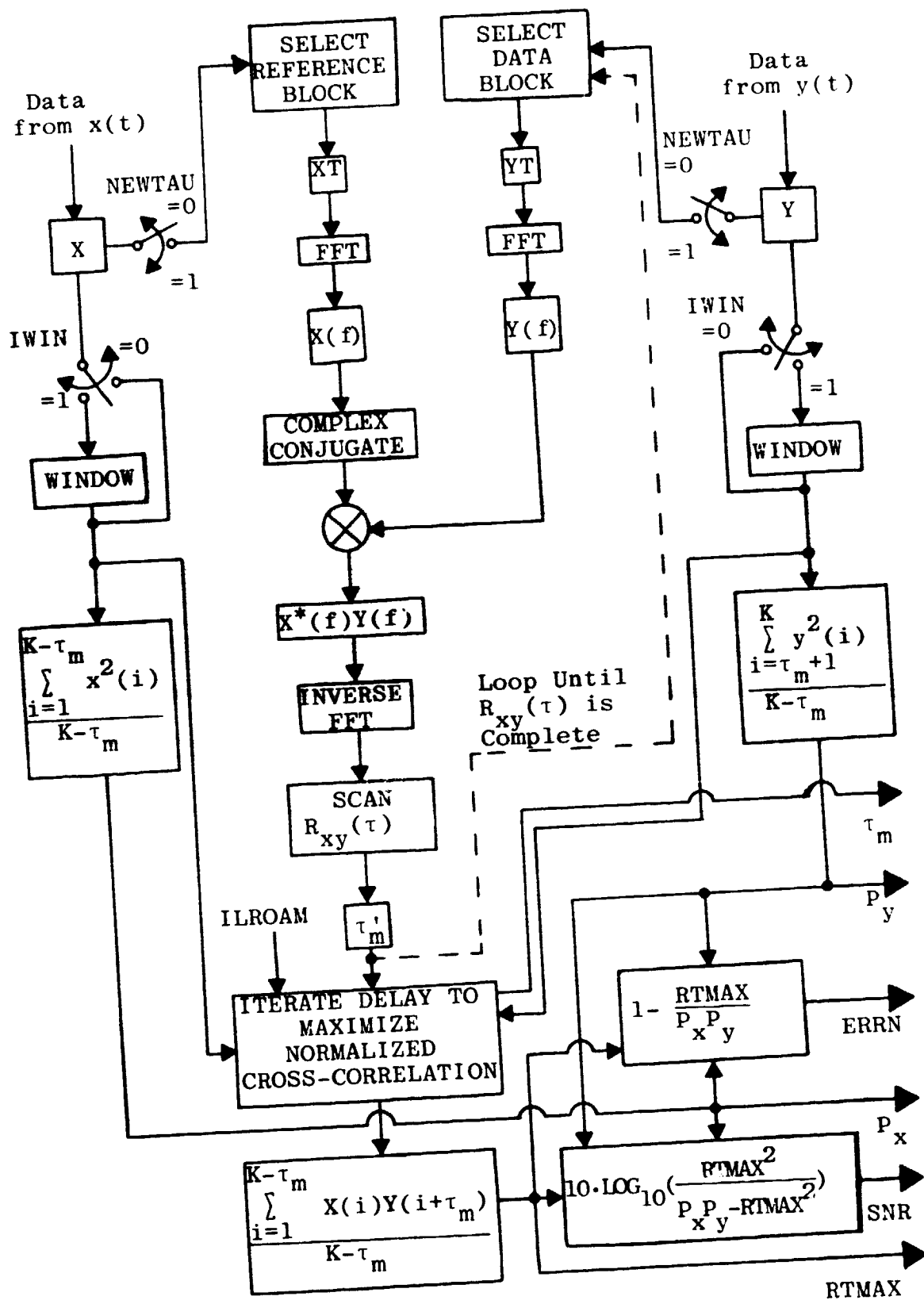
Figure 7. Block Diagram of SNRMSE
