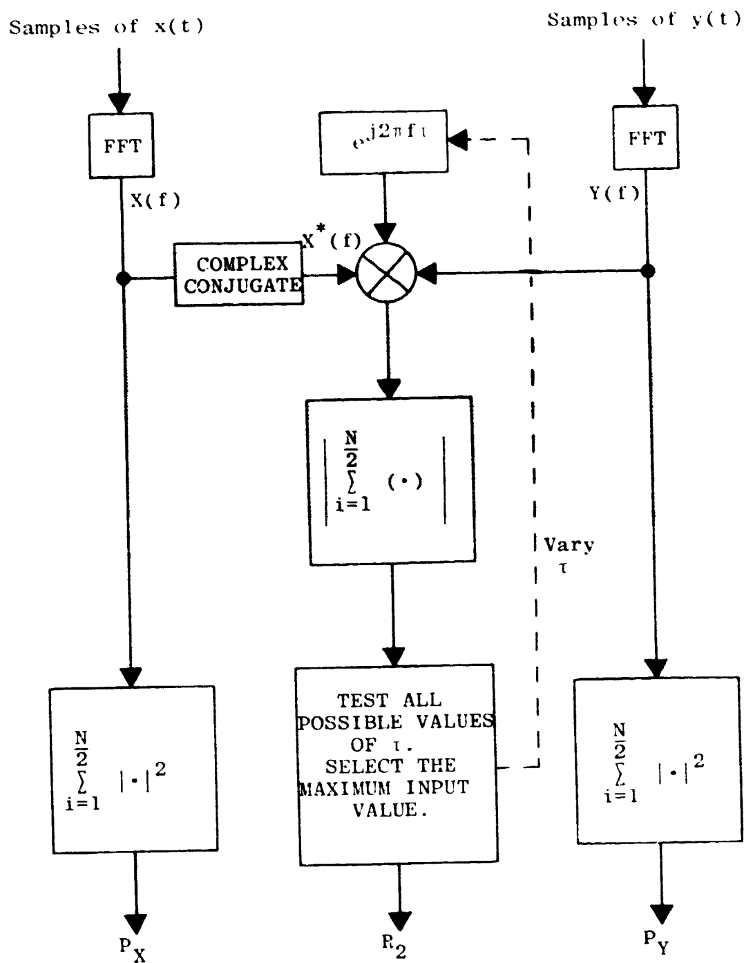
Figure 9. Direct Computation of P_X , P_Y , and R_2
