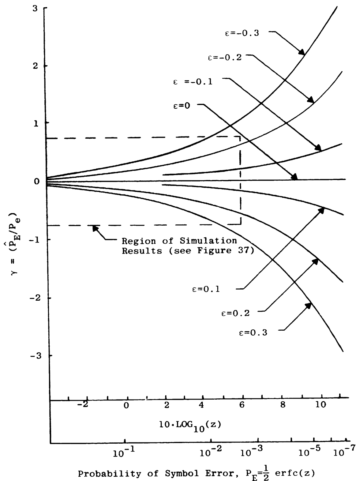
Figure 36. \gamma Versus P_E and 10 \cdot \text{LOG}_{10}(z)
