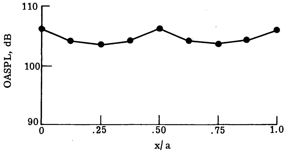
(b) Variation parallel to plate.
