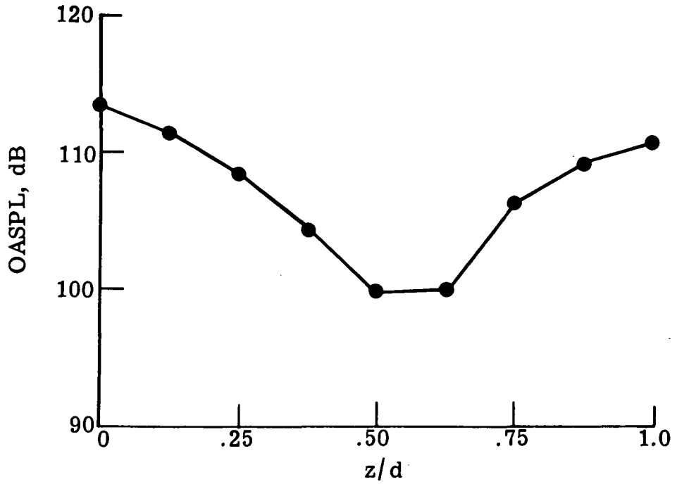
(a) Variation with distance below plate.
