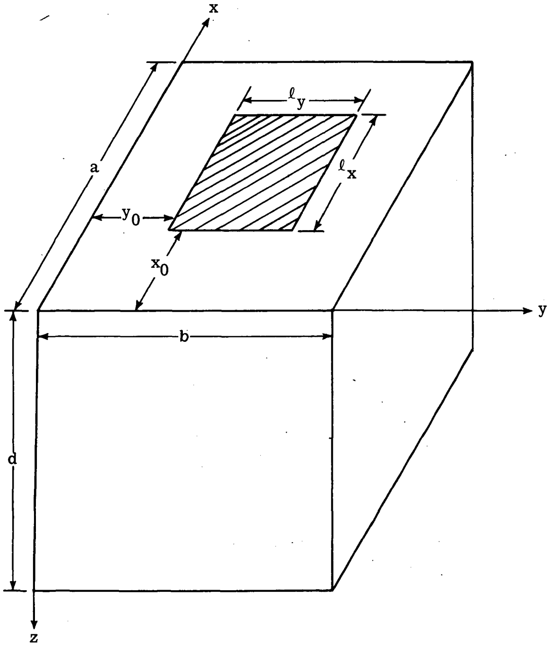
Figure 1.- Cavity and panel geometry.
