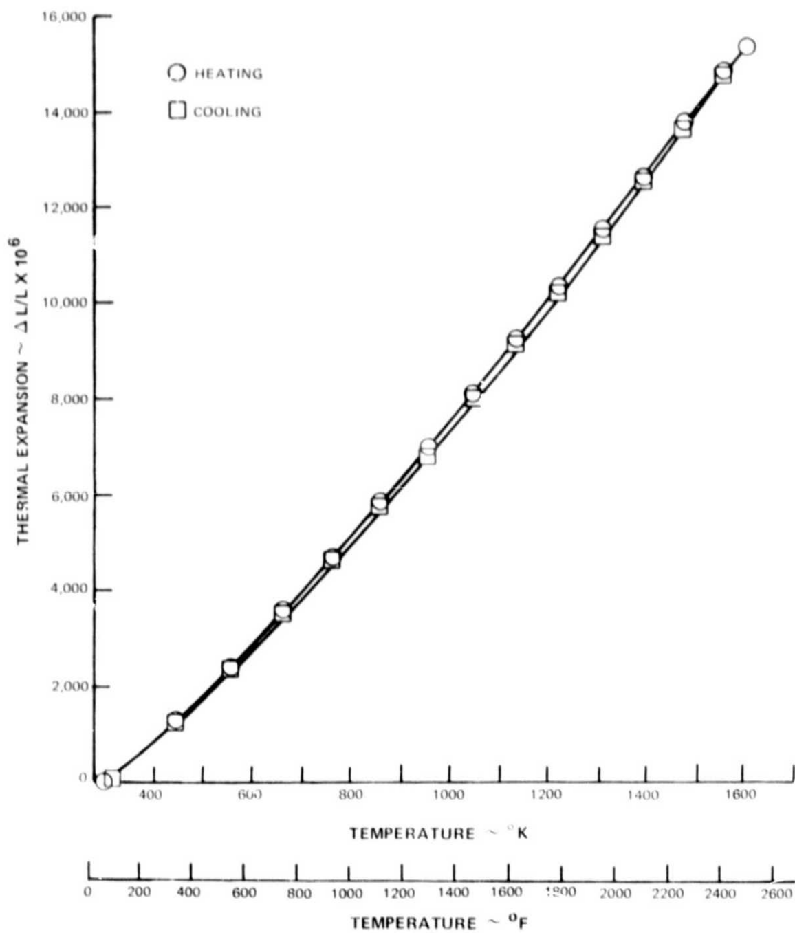
Figure 22 Thermal Expansivity, Plasma Sprayed ZrO_2 on 922°K (1200°F) Metal Substrate - Second Cycle
