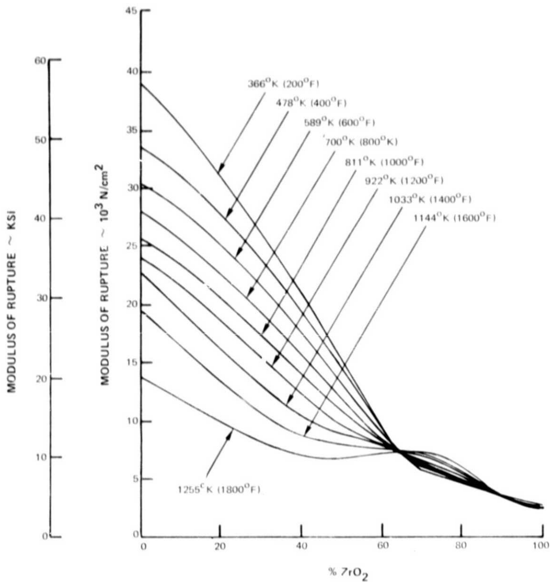
Figure 6 Estimated Modulus of Rupture Variation Versus Spray Powder ZrO 2 Weight Fraction for Plasma Sprayed ZrO 2 /CoCrAlY Materials
