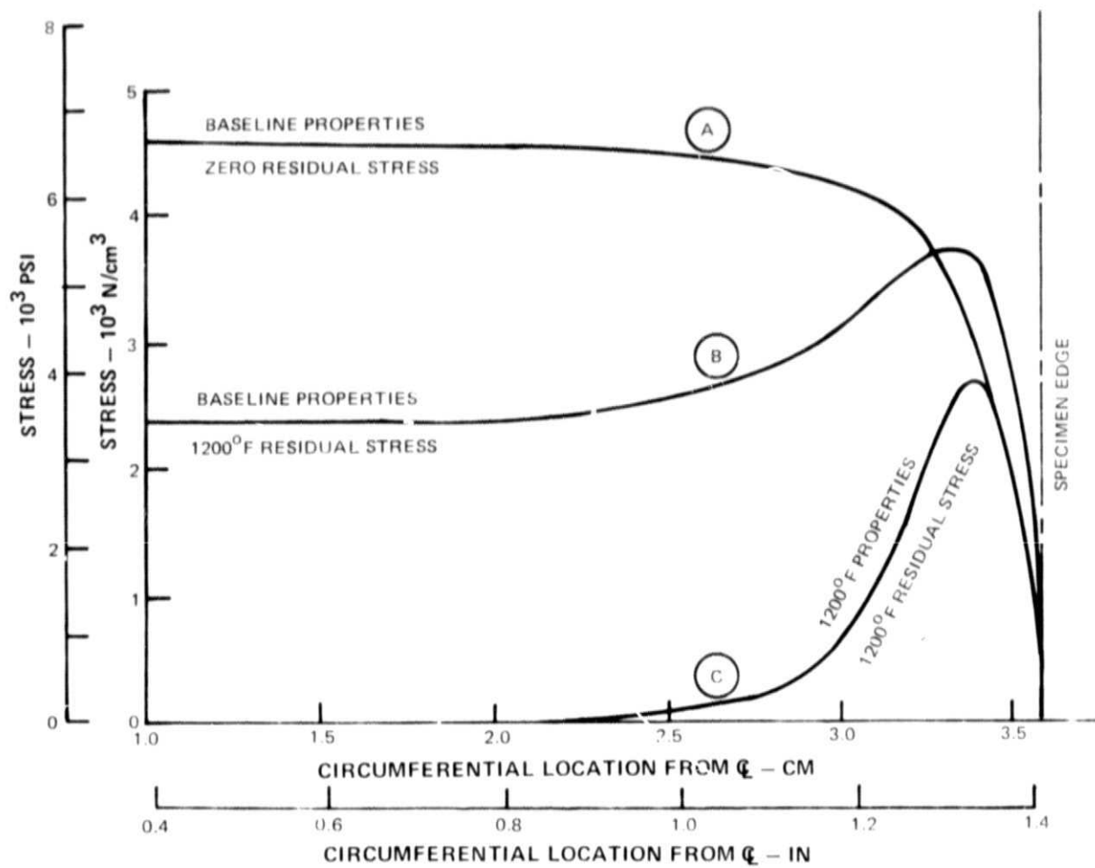
Figure 36 Calculated Maximum Principal Stress Near \text{ZrO}_2 Layer Interface for SLTO Conditions
