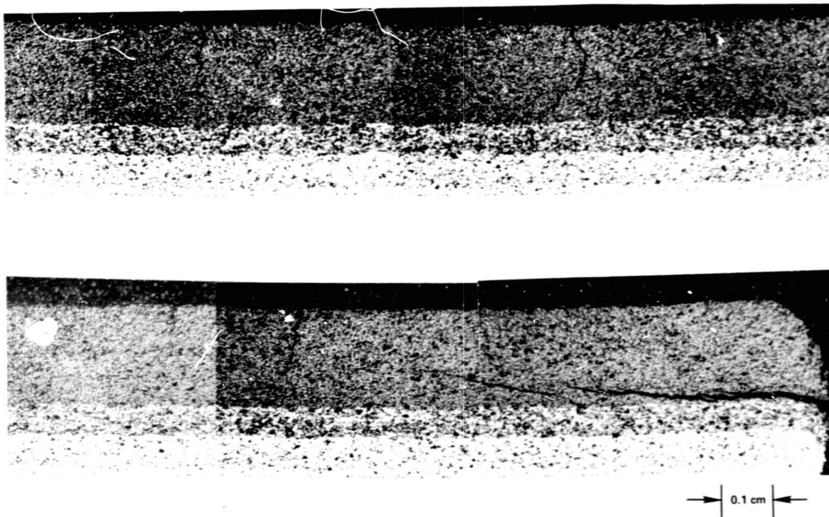
Figure 34 Circumferential Section Through Thermal Fatigue Specimen No. 1 (78-441-8415)
