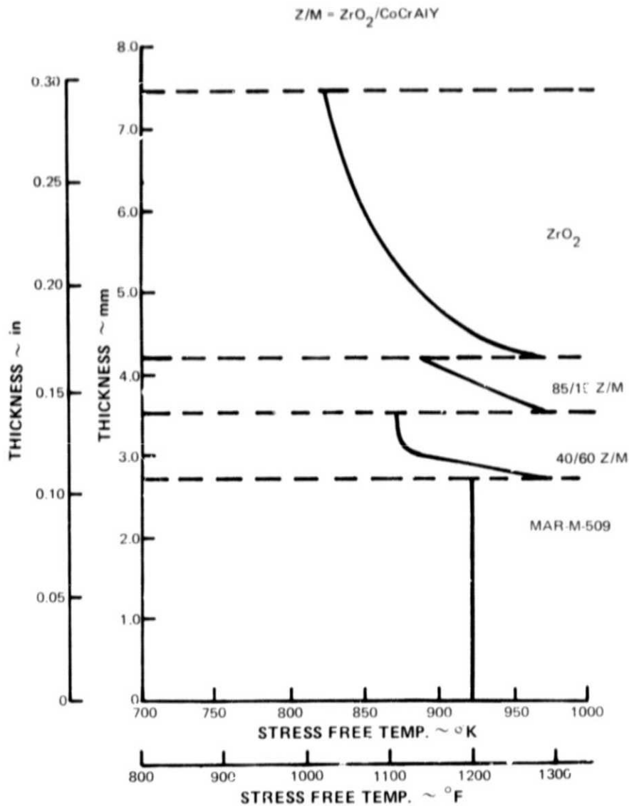
Figure 18 Stress Free Temperature Distribution, 922°K (1200°F) Seal System – 922°K (1200°F) Material Properties
