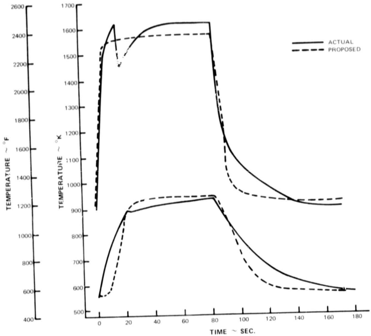
Figure 29 Thermal Fatigue Test Cycle
