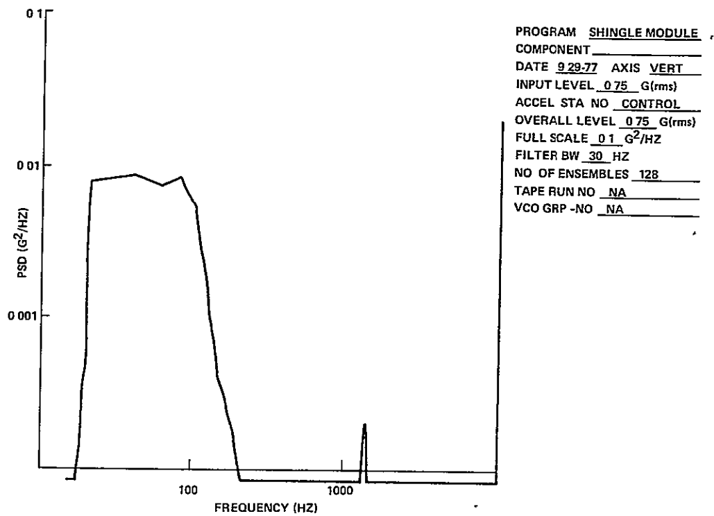
Figure 3-24. Power Spectra Density Plot of Random Vibration Input
