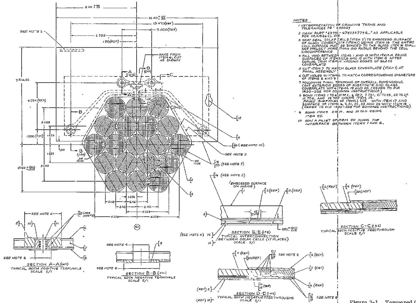
Figure 3-1. Tempered Glass Covered Module Design
