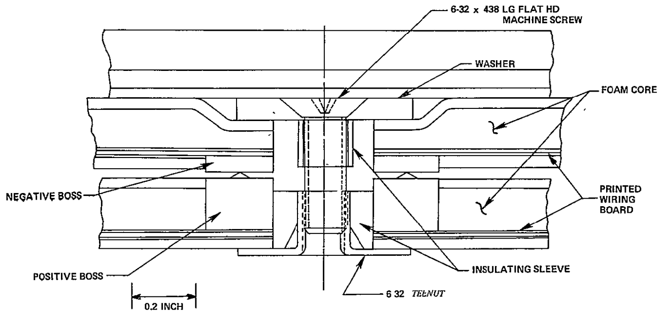
Figure 3-12. Module-to-Module Interconnection
