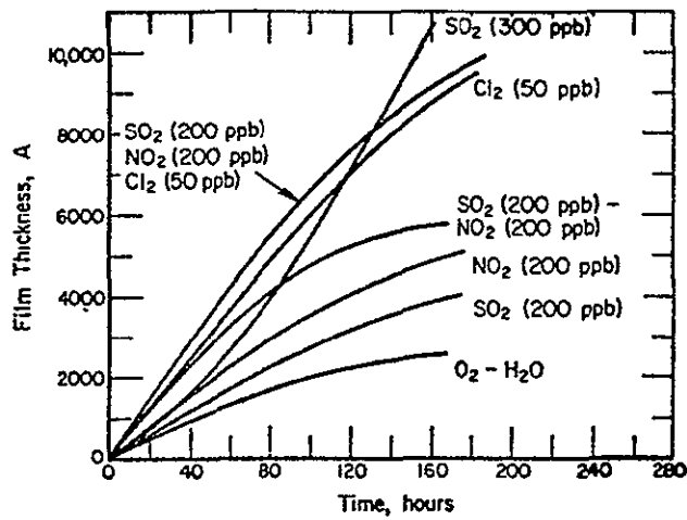
Figure 3-26. Tarnish Kinetics of Copper in \text{N}_2 - \text{O}_2 - \text{H}_2\text{S} (200 ppb) Mixtures with \text{SO}_2 , \text{NO}_2 , \text{Cl}_2 at 30 C
