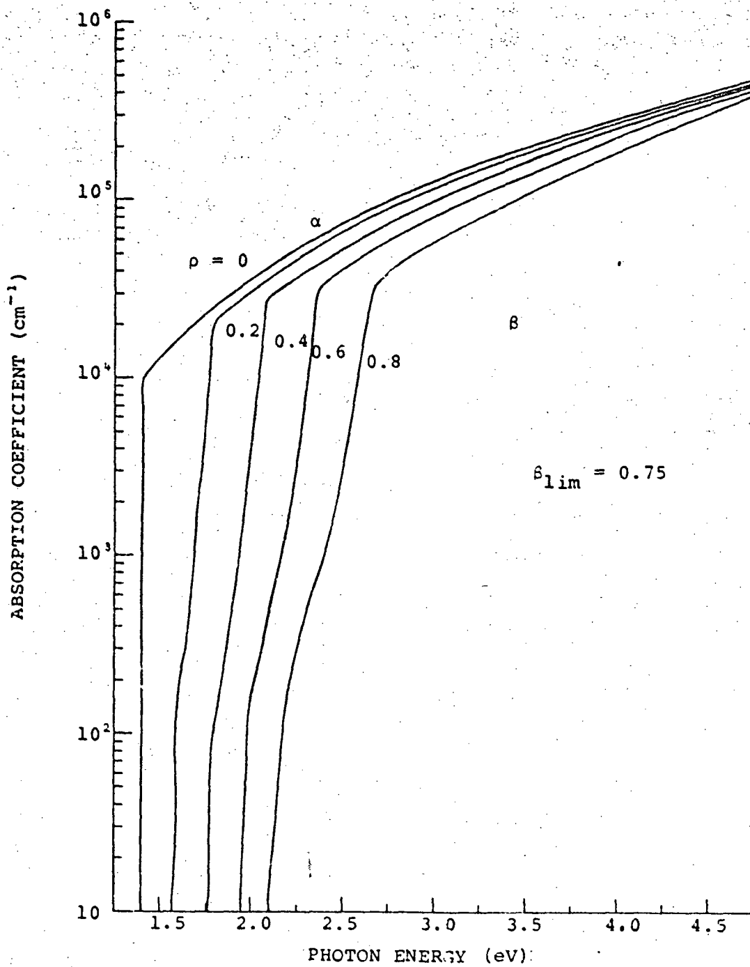
Figure 9. Absorption coefficient curves for Ga 1-p Al p As for p = 0, 0.2, 0.4, 0.6 and 0.8 .
