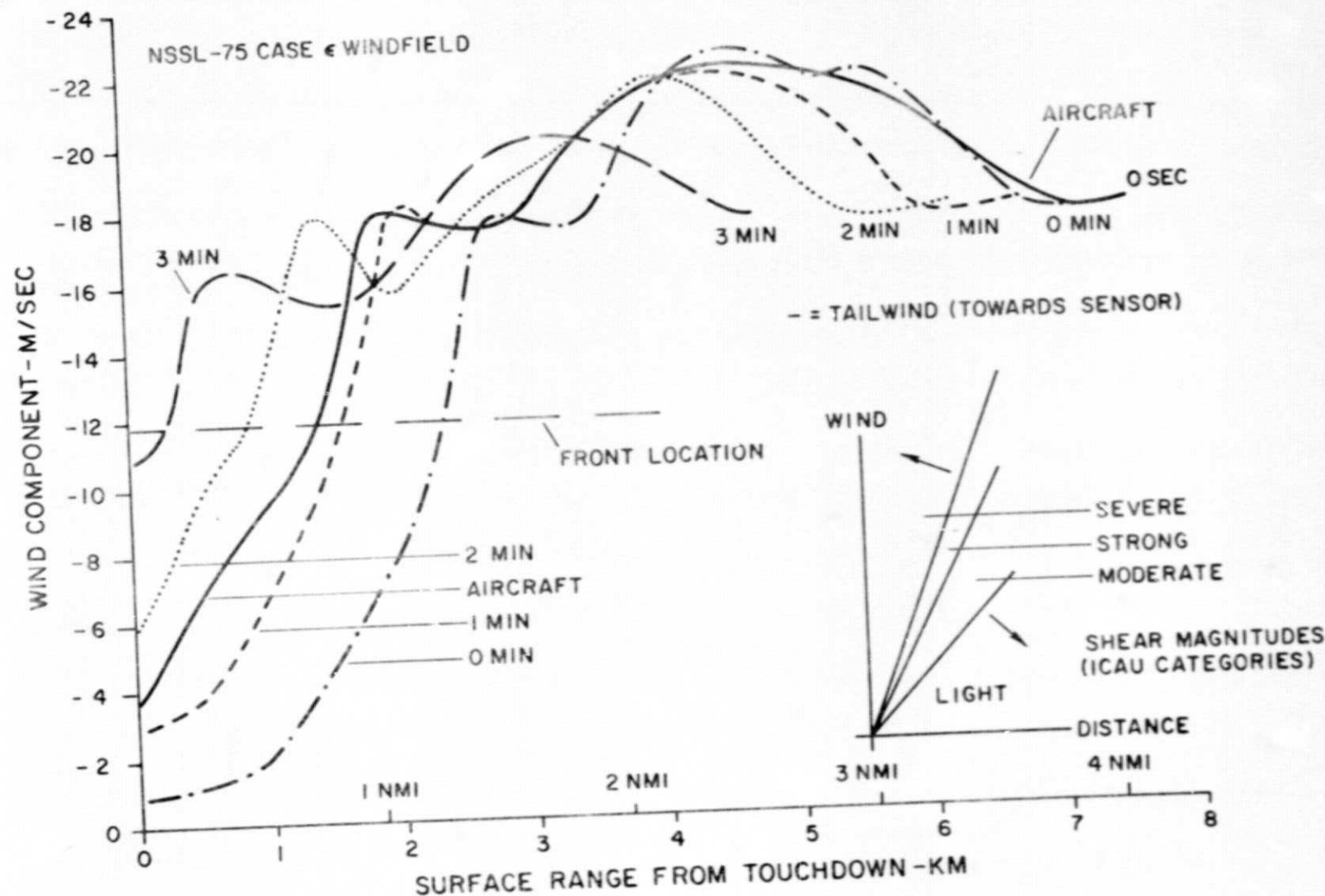
Figure 10. Comparison of Aircraft Experienced Wind and Glide Slope Sensor Measurements
