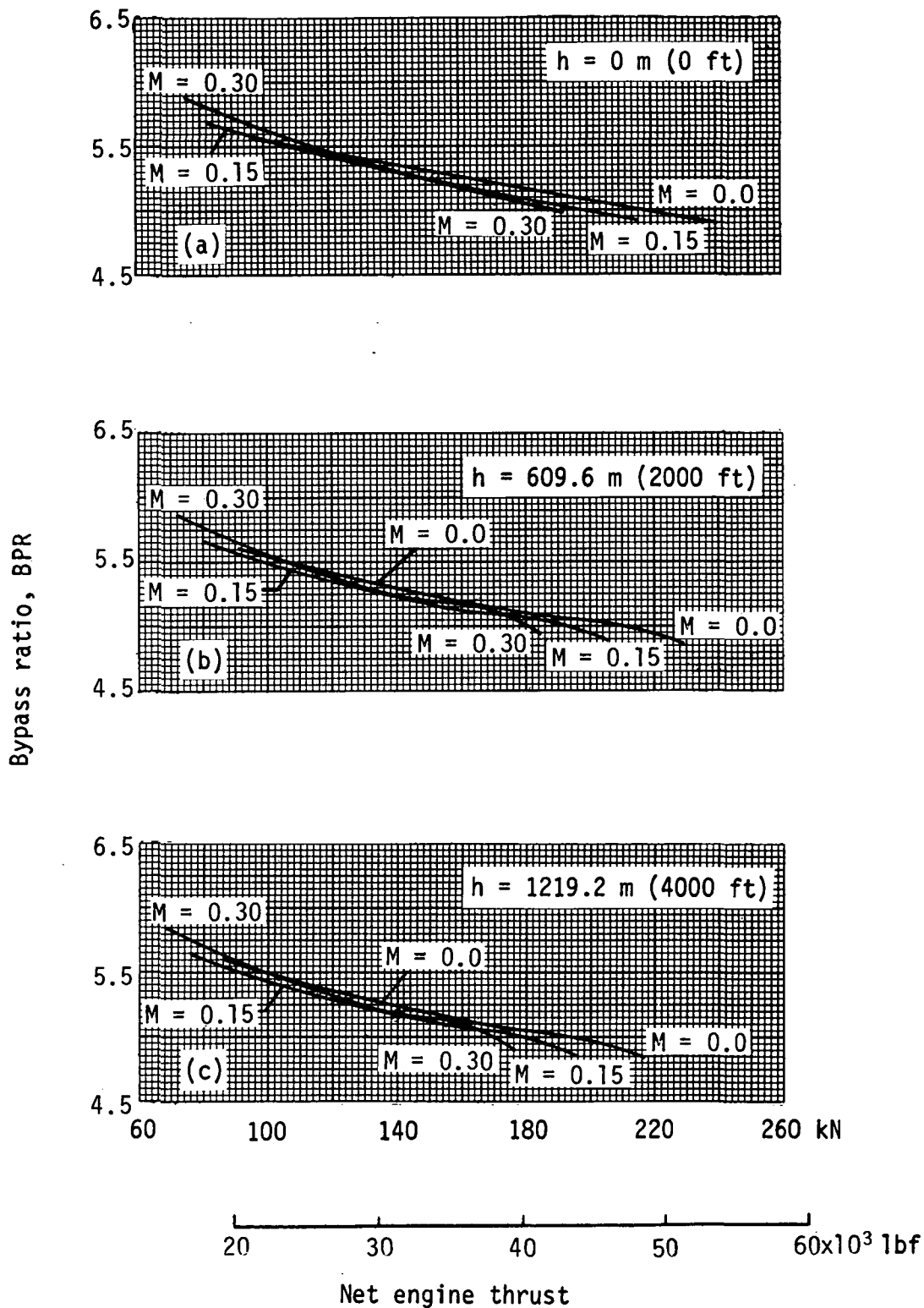
Figure 43.- Installed engine bypass ratio at take-off and part-power cruise thrust. Standard day + 10° C.
