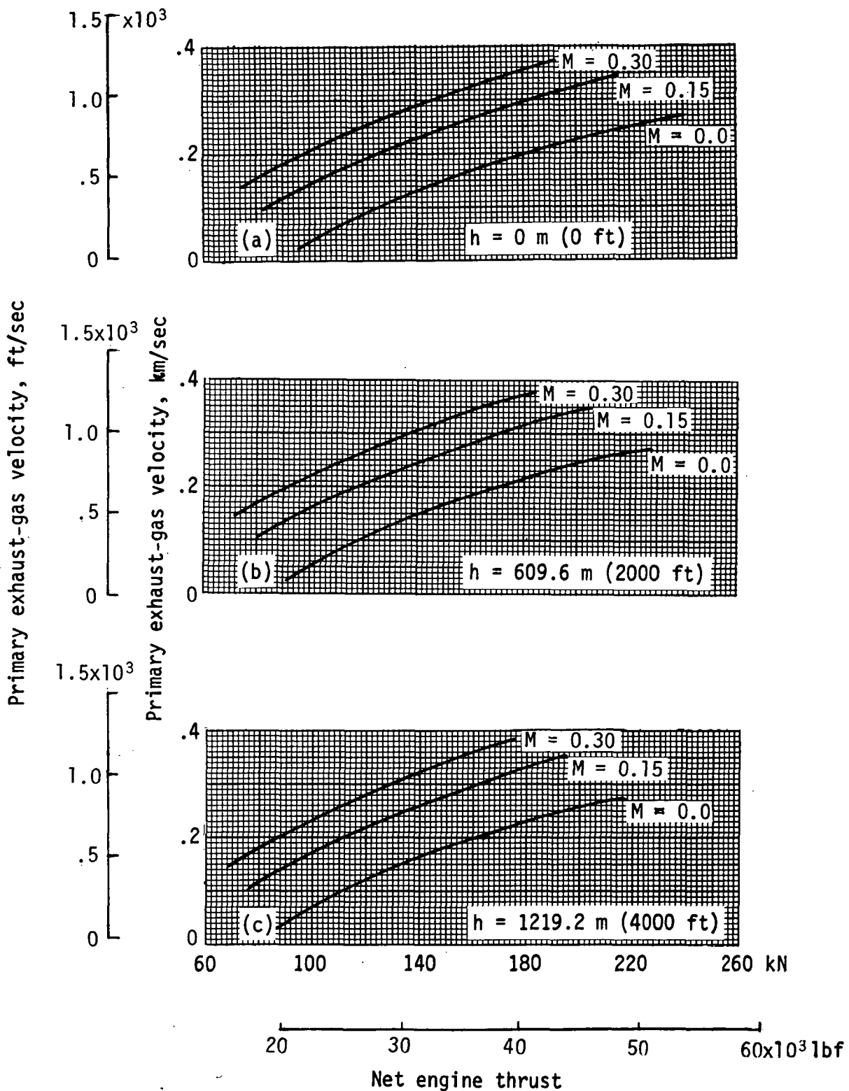
Figure 45.- Installed primary exhaust-gas velocity at take-off and part-power cruise thrust. Standard day + 10° C.
