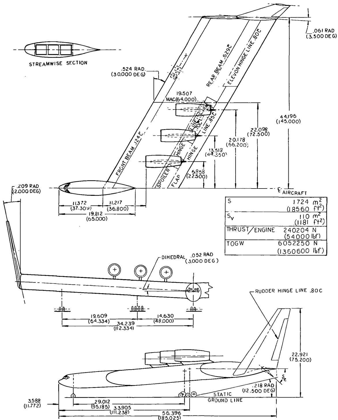
Figure 1.- Span-distributed-load cargo airplane configuration. Dimensions are shown in meters with feet in parentheses except as noted.
