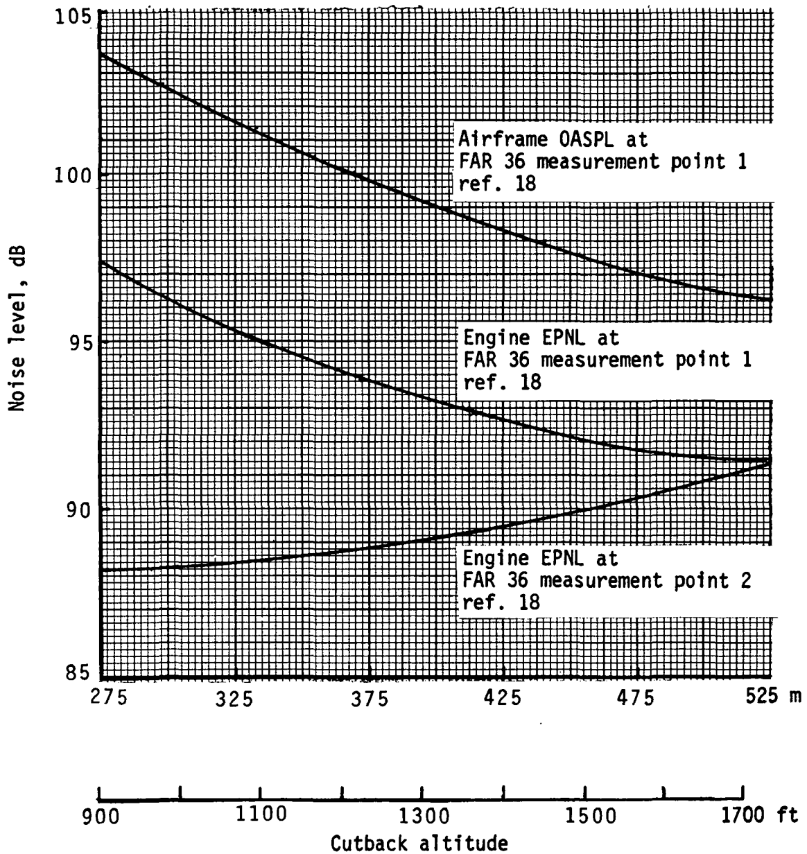
Figure 59.- Effect of cutback altitude on span-loader take-off noise levels.
