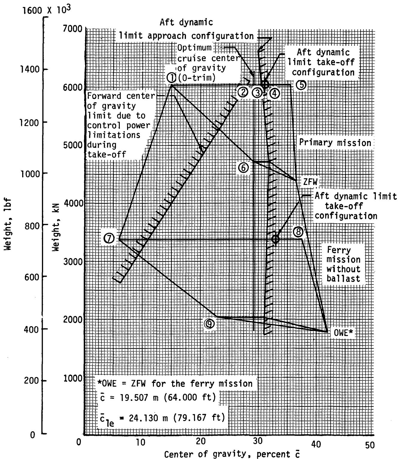
Figure 17.- Loadability envelope with flight limitations. (See table III for correlation of point number.)
