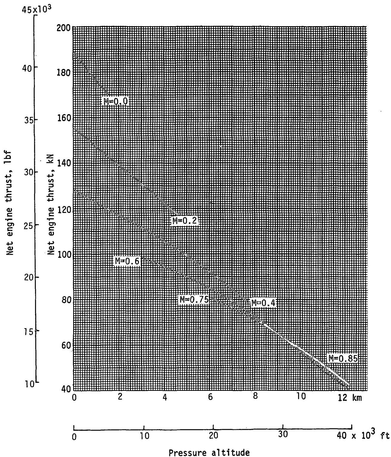
Figure 39.- Installed maximum-cruise net engine thrust. Standard day to (standard day + 15° C).
