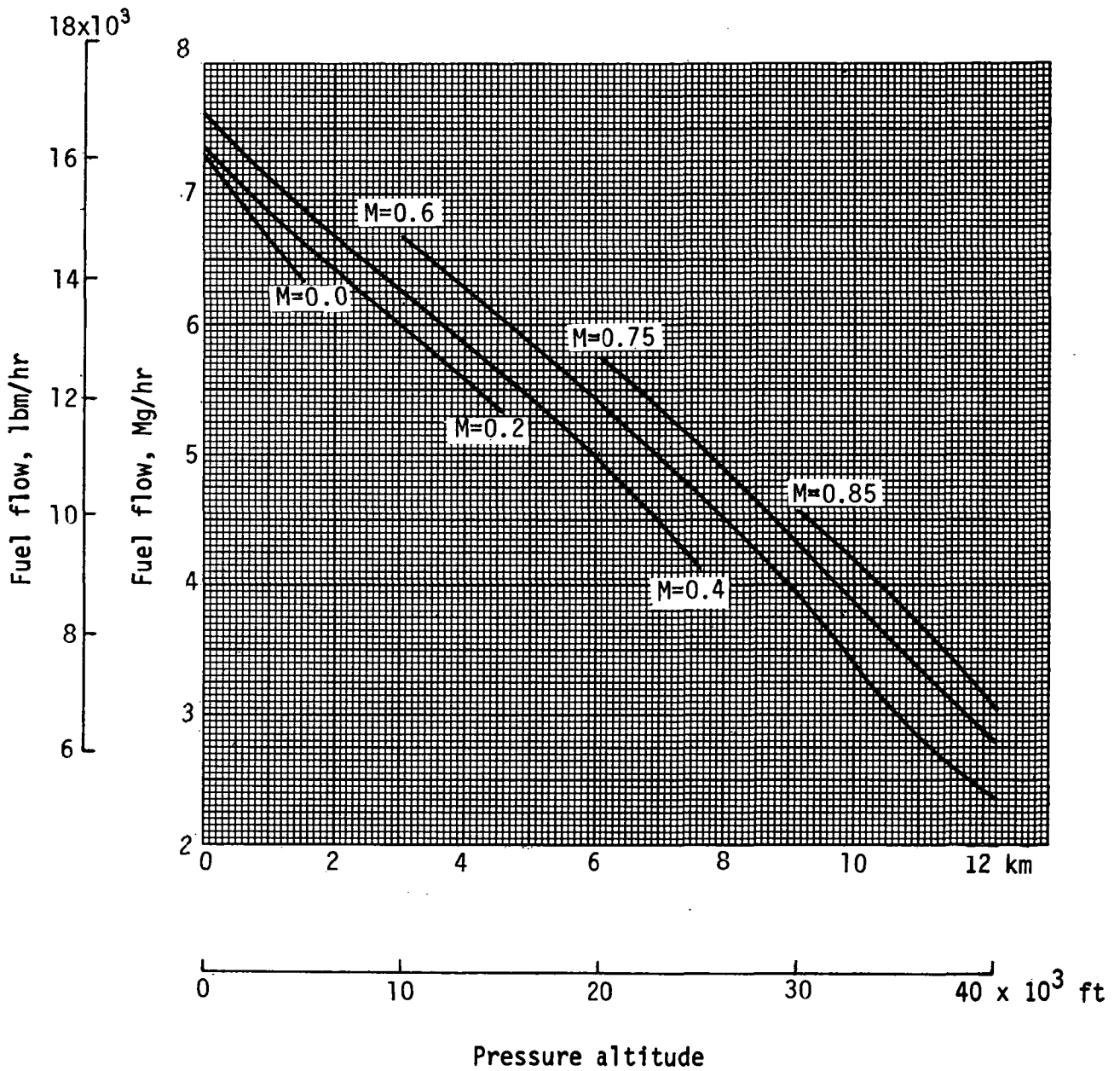
Figure 38.- Installed maximum-climb fuel flow. Standard day.
