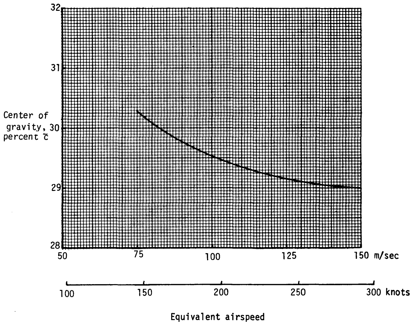
Figure 30.- Rearward dynamic center-of-gravity limit for climb-acceleration mode. \delta_f = 0^\circ .
