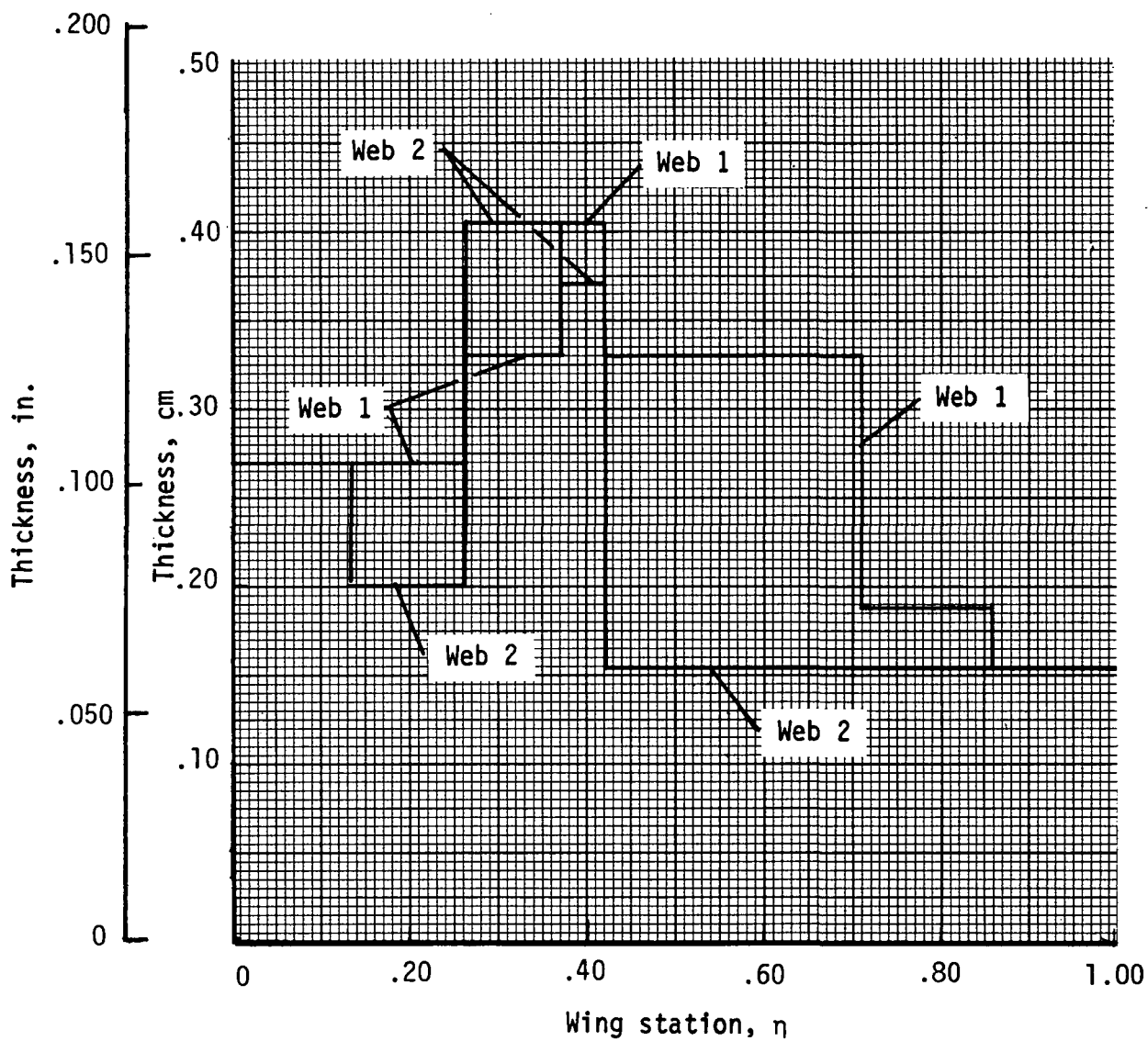
Figure 10.- Web thicknesses of beams 1 (forward) and 2 (rearward).
