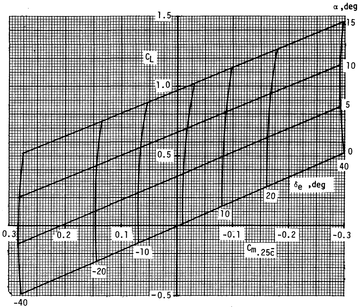
Figure 23.- Effect of elevon deflection on lift and pitching moment. \delta_f = 0^\circ ; cruise.
