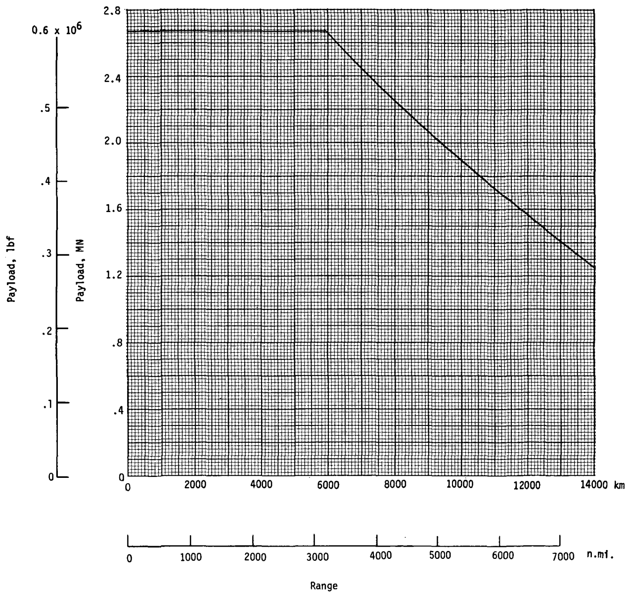
Figure 55.- Variation of payload with range.
