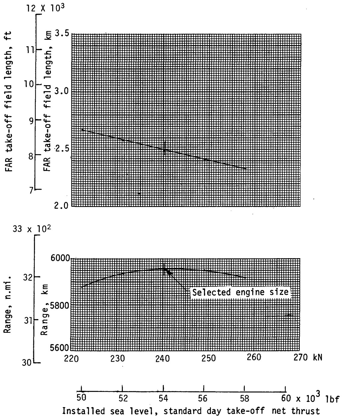
Figure 50.- Effect of engine size on range and FAR take-off field length. Standard day, sea level, 20° flaps.
