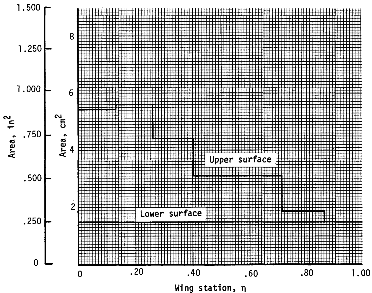
Figure 14.- Wing box stringer sectional areas, upper and lower surfaces.
