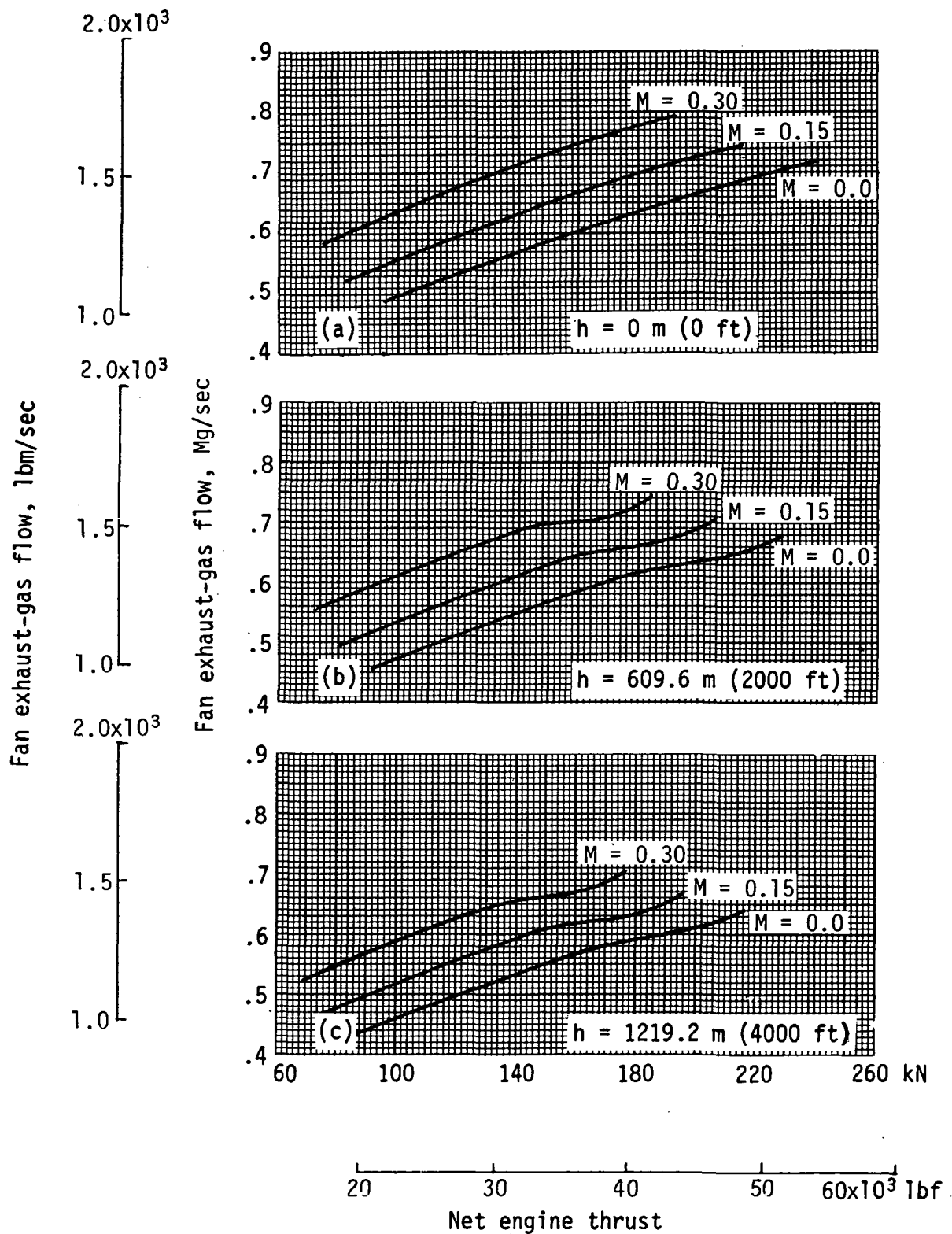
Figure 48.- Installed fan exhaust-gas flow at take-off and part-power cruise thrust. Standard day + 10° C.
