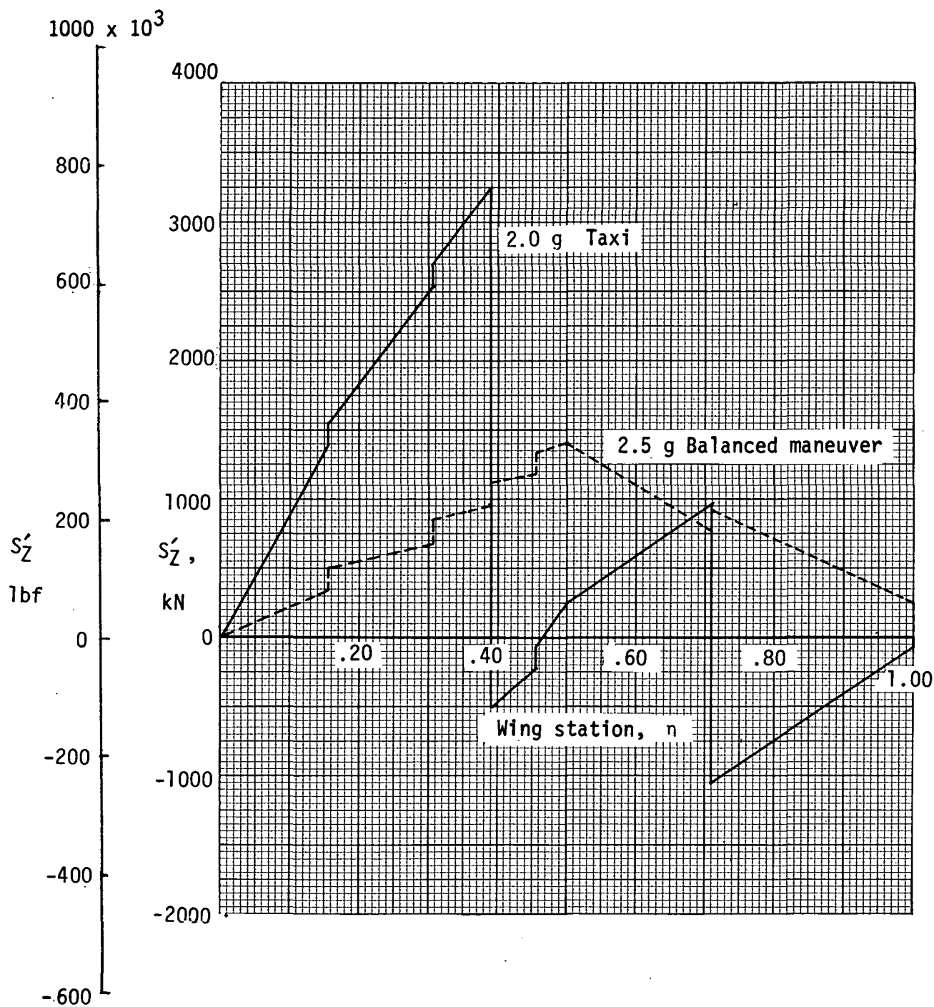
Figure 5.- Net limit swept axis shears.
