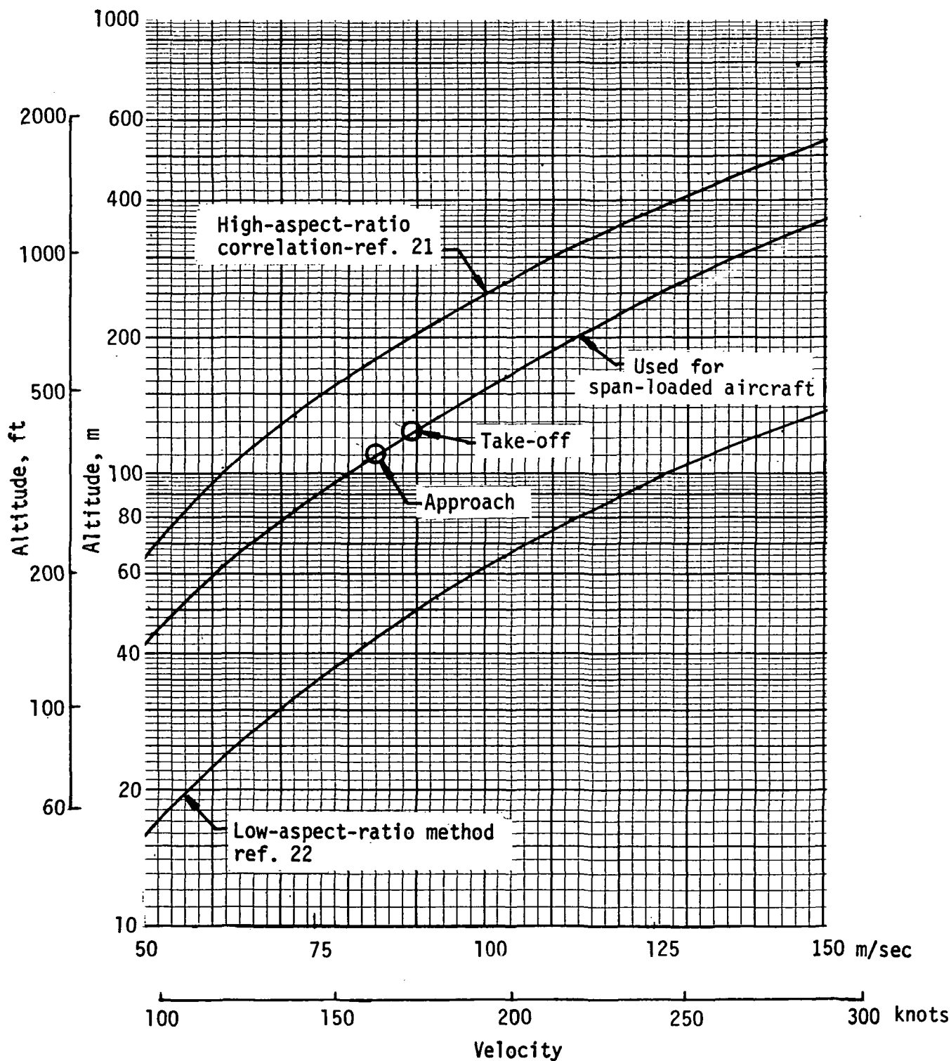
Figure 58.- Variation of altitude with velocity for span-loader airframe noise level of 108 dB. (Airplane is directly over measurement point.)
