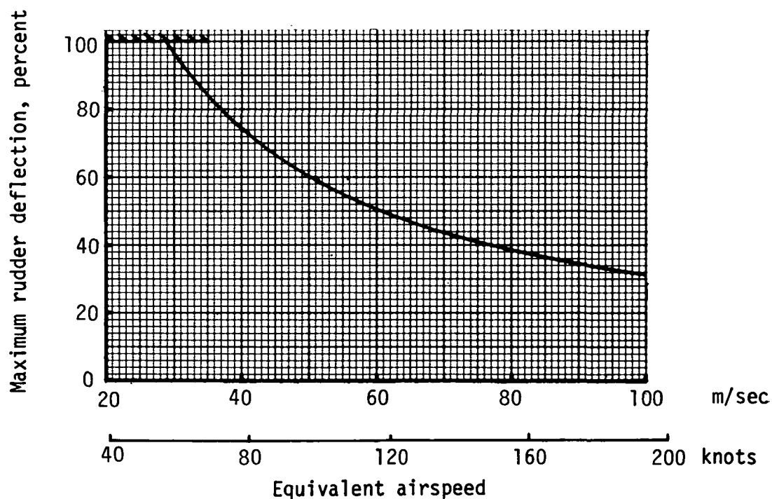
Figure 33.- Estimated aircraft directional trim requirements in a 90°, 15.4 m/sec (30 knots) cross wind.
