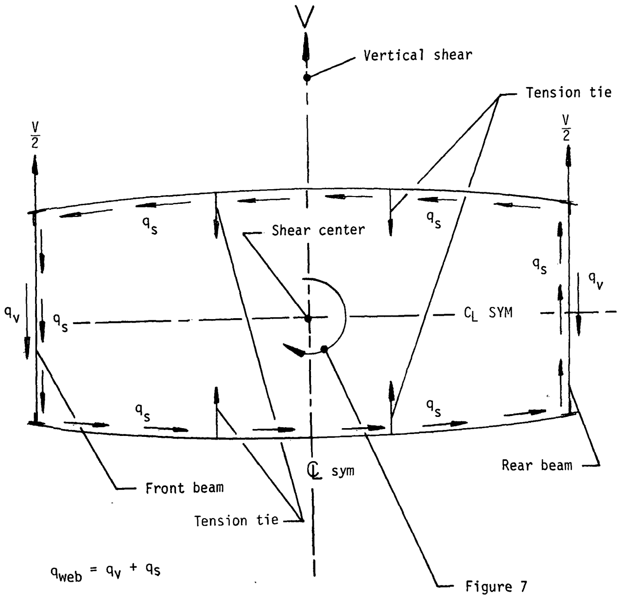
Figure 9.- Shear flow schematic.
