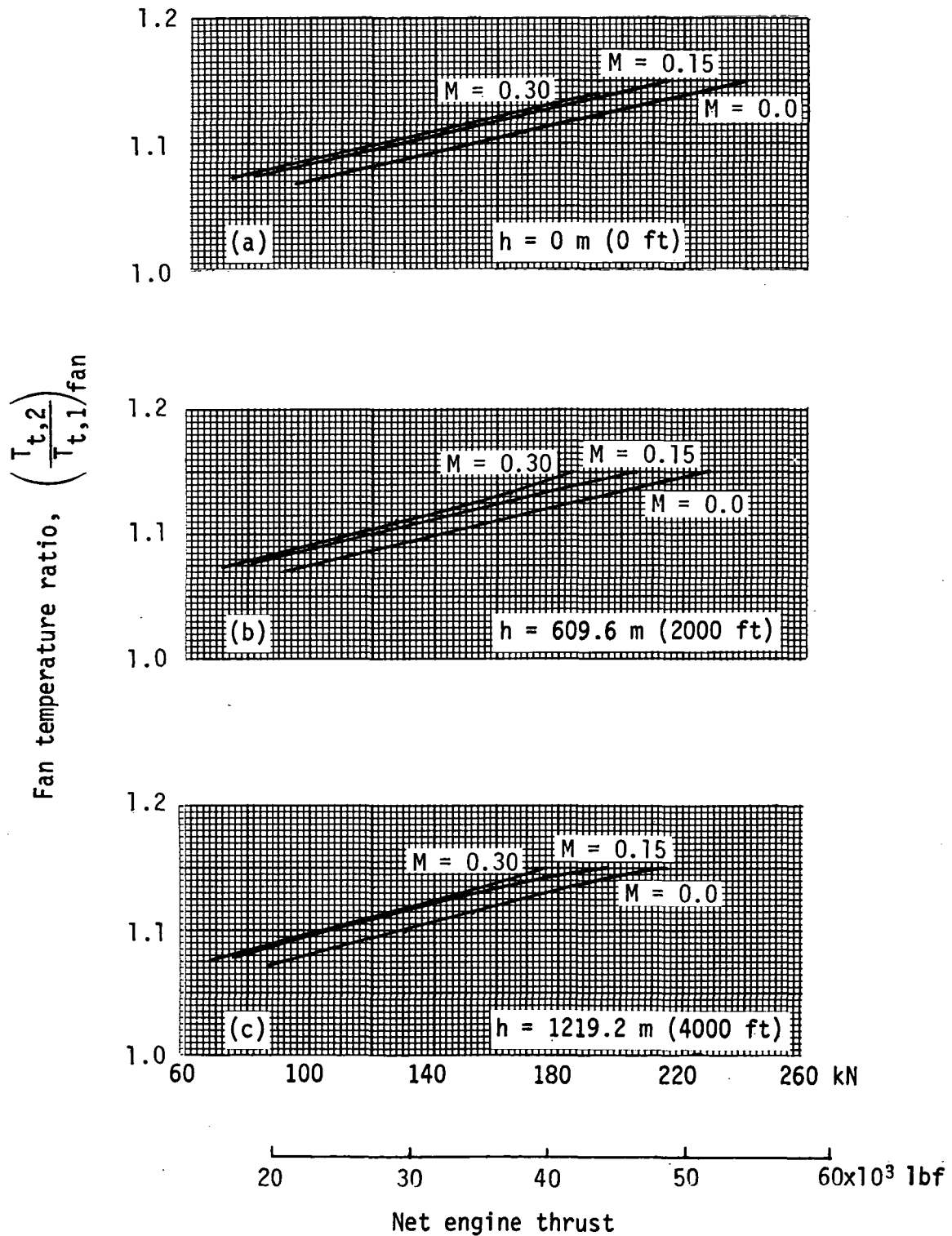
Figure 46.- Installed fan temperature ratio at take-off and part-power cruise thrust. Standard day + 10° C.
