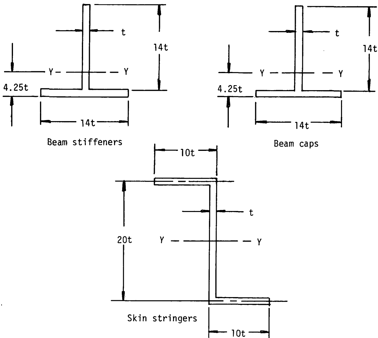
Figure 11.- Cross sections of mean stiffeners, beam caps, and skin stringers.
