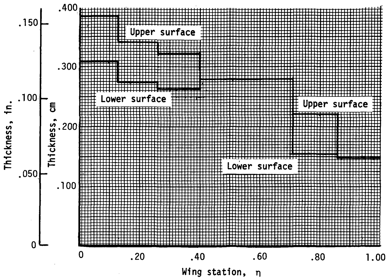
Figure 15.- Wing box skin thickness, upper and lower surfaces.
