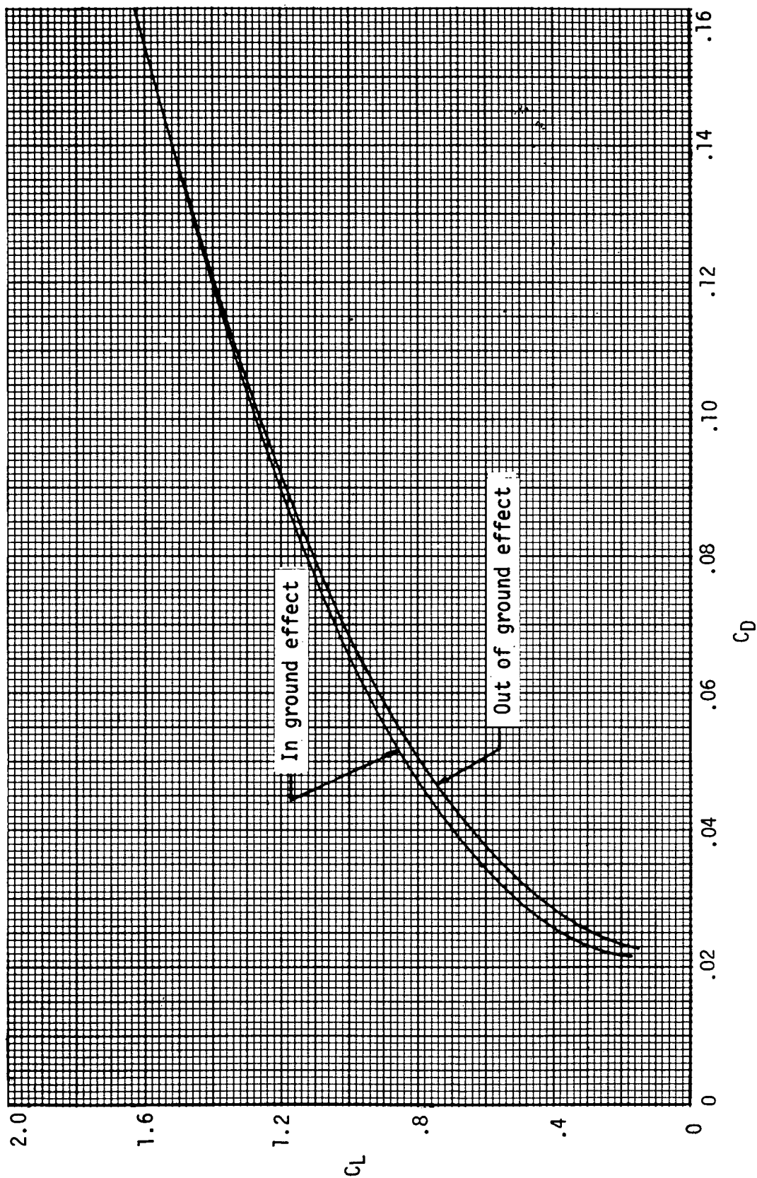
Figure 18.- Landing lift-drag polar. S = 1724 \text{ m}^2 (18 560 \text{ft}^2 ); \delta_f = 20^\circ ; center of gravity, 0.34\bar{c} ; landing gear extended.
