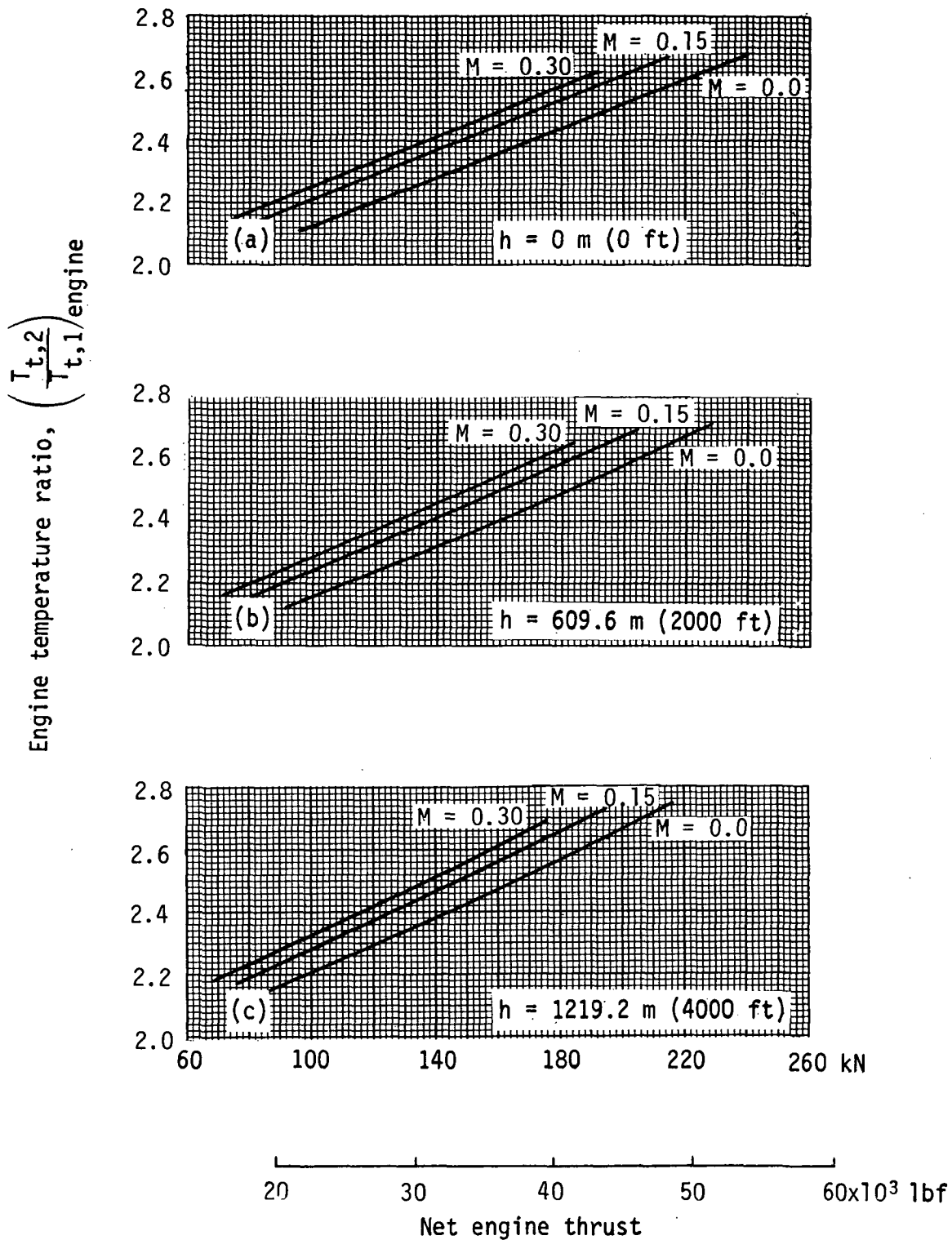
Figure 47.- Installed engine temperature ratio at take-off and part-power cruise thrust. Standard day + 10° C.
