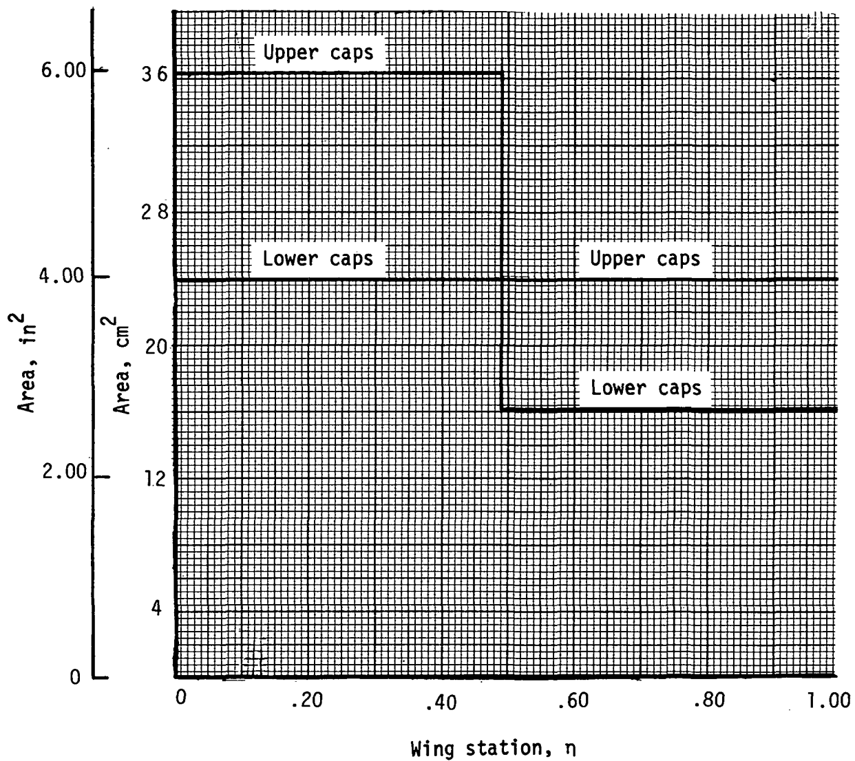
Figure 13.- Upper and lower beam cap sectional areas of beams 1 (forward) and 2 (rearward).
