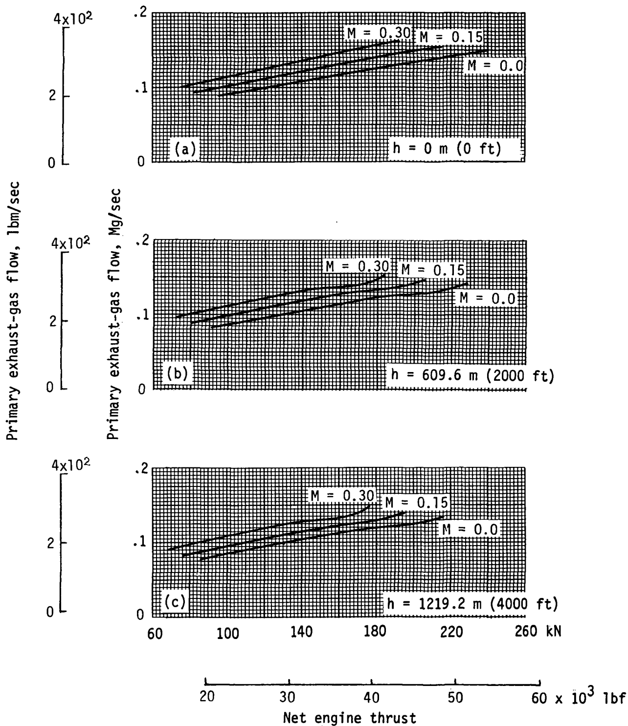
Figure 49.- Installed primary exhaust-gas flow at take-off and part-power cruise thrust. Standard day + 10^\circ \text{ C} .
