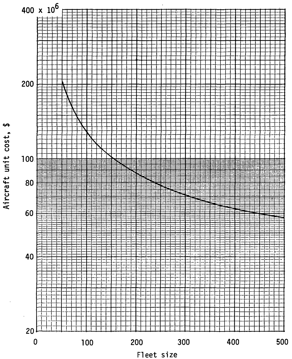
Figure 64.- Variation of aircraft unit cost with number of units produced, 1977 dollars.
