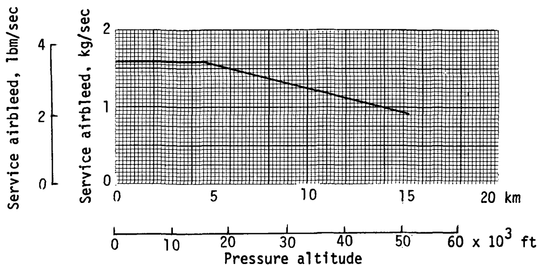
Figure 35.- Service airbleed schedule per engine.
