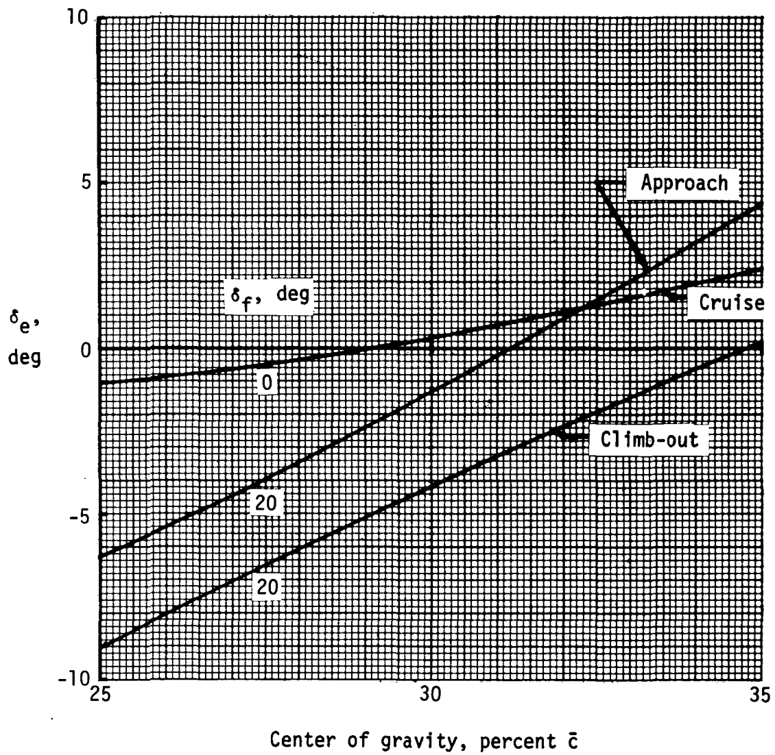
Figure 26.- Elevon required to trim.
