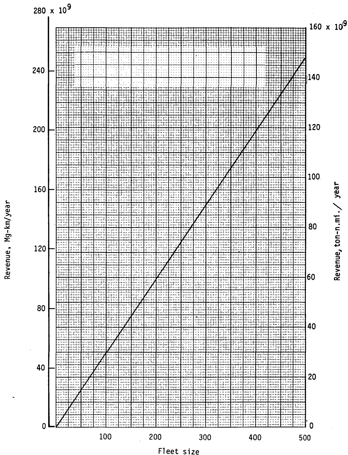
Figure 65.- Variation of productivity with fleet size. Utilization, 3500 hr/yr; load factor, 0.65; range, 5926 km (3200 n. mi.).
