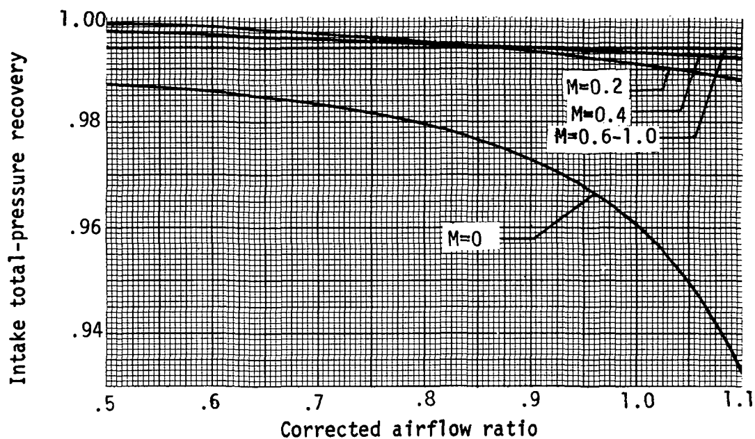
Figure 34.- Air-inlet total pressure recovery.
