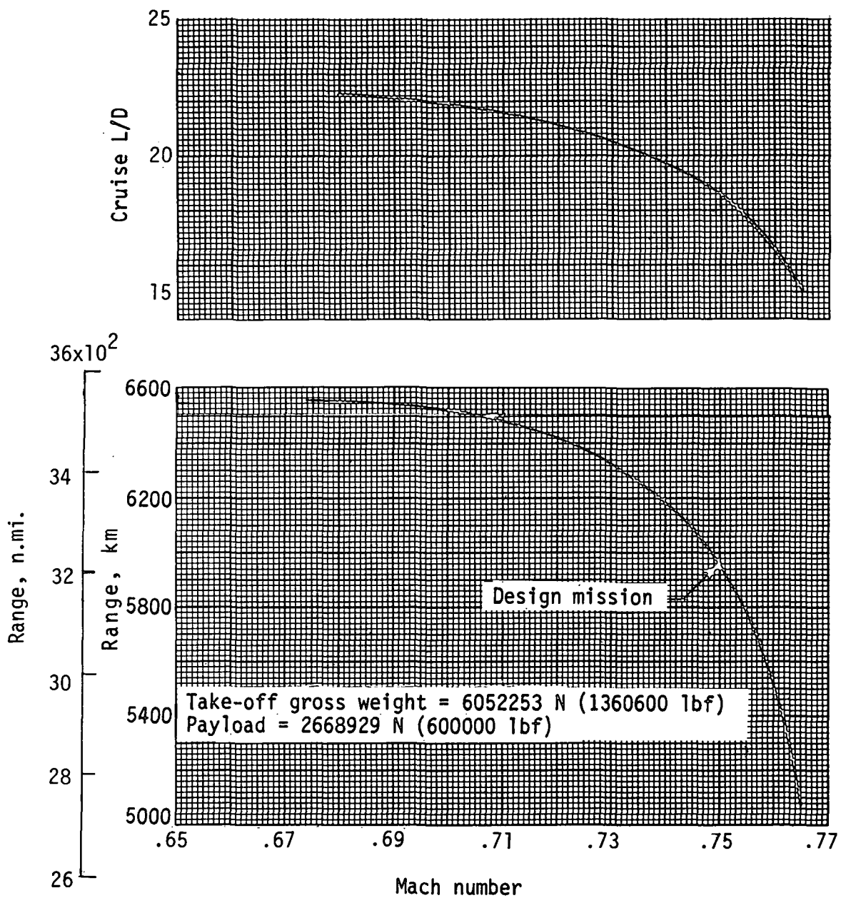
Figure 53.- Effect of Mach number on range and L/D.
