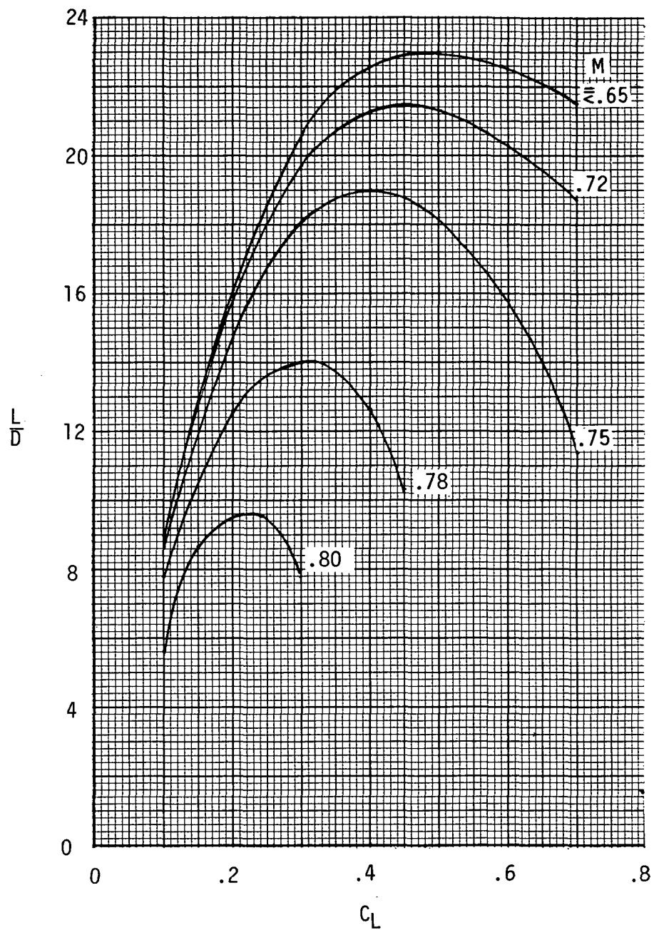
Figure 22.- Lift-drag variation with lift coefficient for several cruise Mach numbers. S = 1724 \text{ m}^2 (18 560 \text{ft}^2 ).
