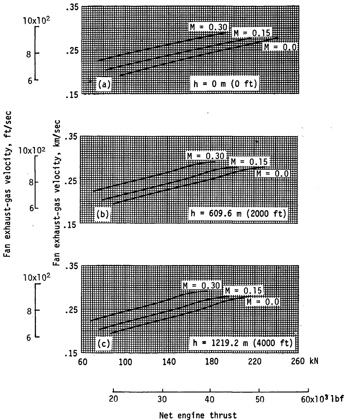
Figure 44.- Installed fan exhaust-gas velocity at take-off and part-power cruise thrust. Standard day + 10° C.
