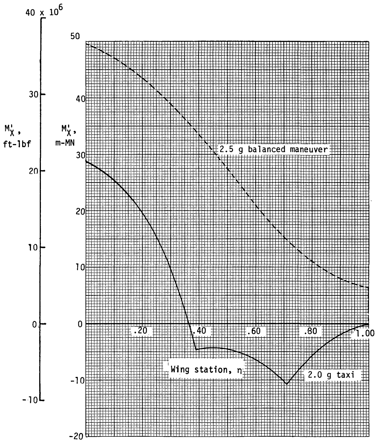
Figure 6.- Net limit swept axis bending moments.
