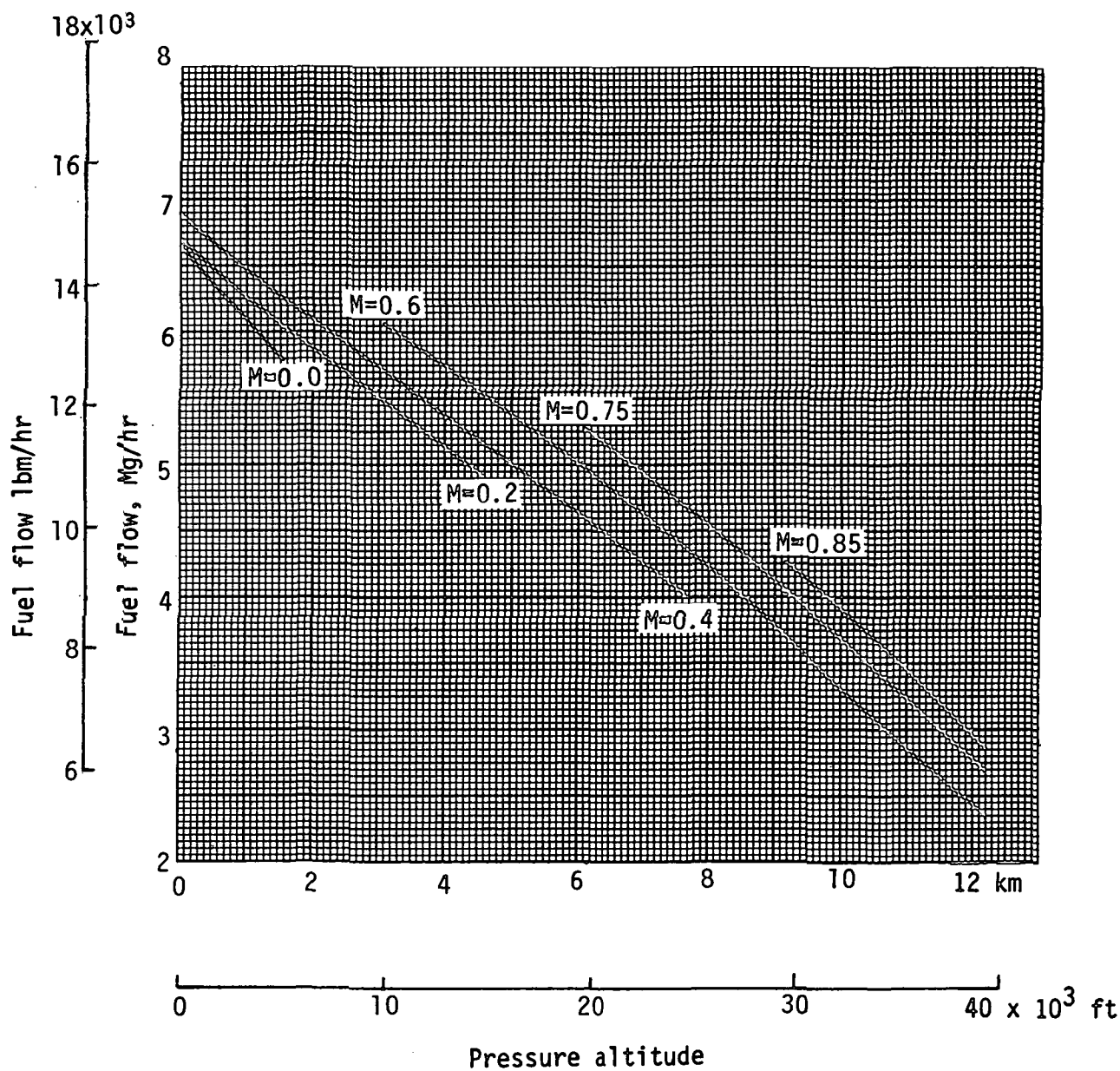
Figure 40.- Installed maximum-cruise fuel flow. Standard day.
