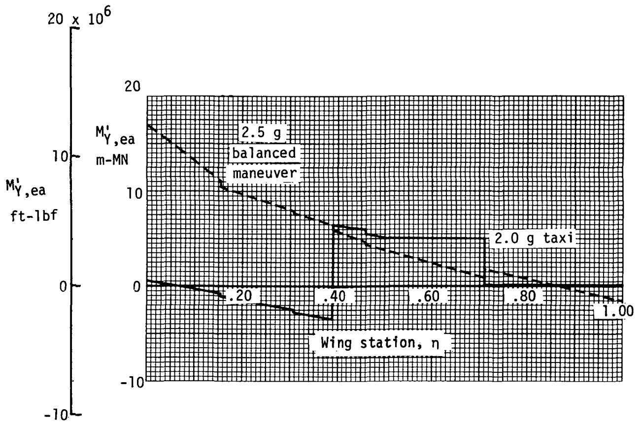
Figure 7.- Net limit swept axis torsions.
