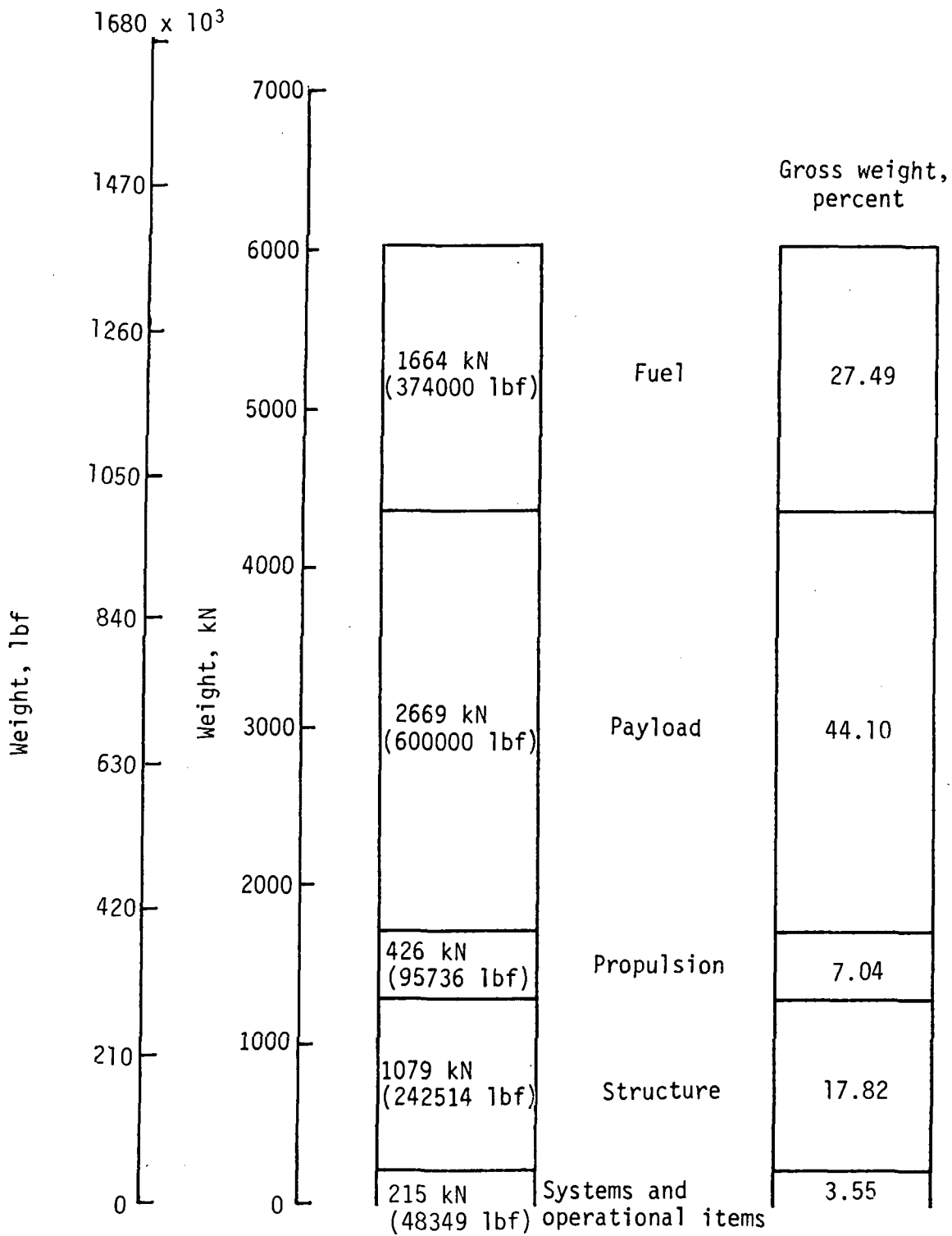
Figure 16.- Gross weight breakdown.
