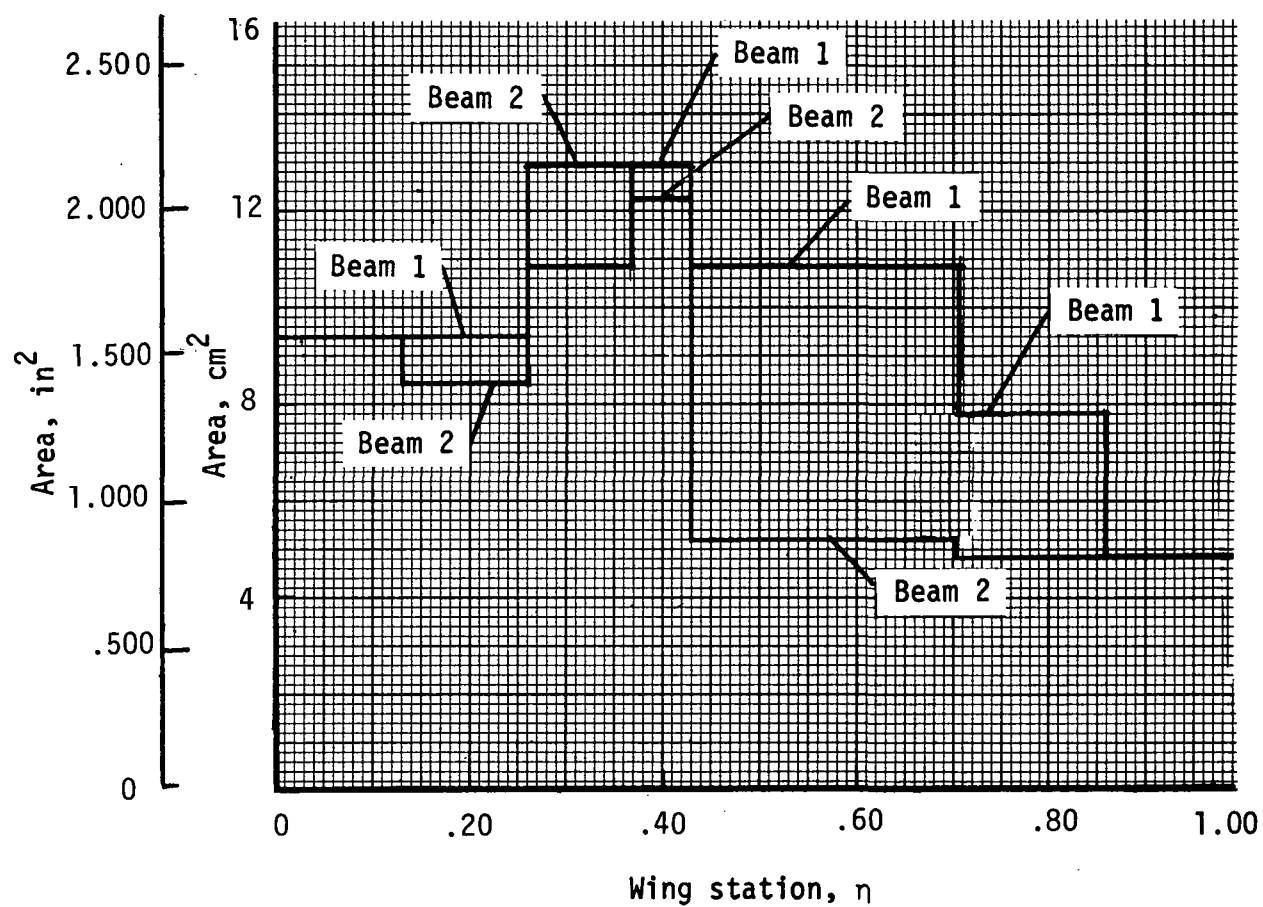
Figure 12.- Stiffener sectional areas of beams 1 (forward) and 2 (rearward).
