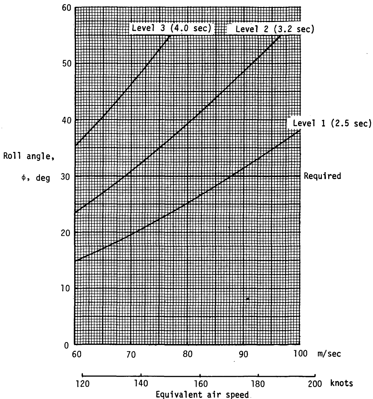
Figure 32.- Estimated aircraft roll response to a lateral step input. Landing approach. Approach configuration; C_{n,elastic}/C_{n,rigid} assumed equal to 0.90; class III; category C, reference 14.
