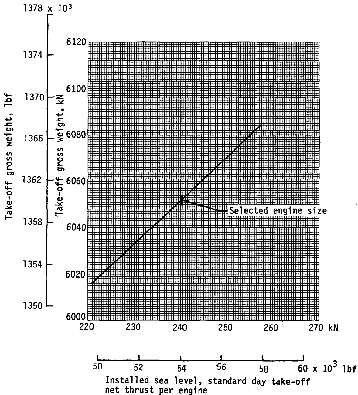
Figure 52.- Effect of engine size on gross weight.
