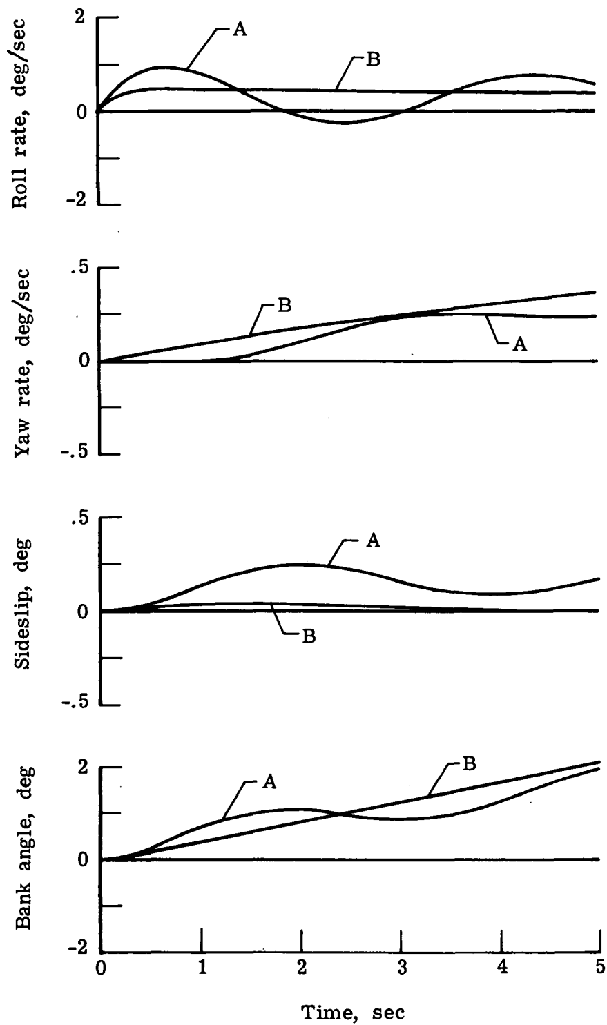
(b) Flight condition 17 (landing approach).
