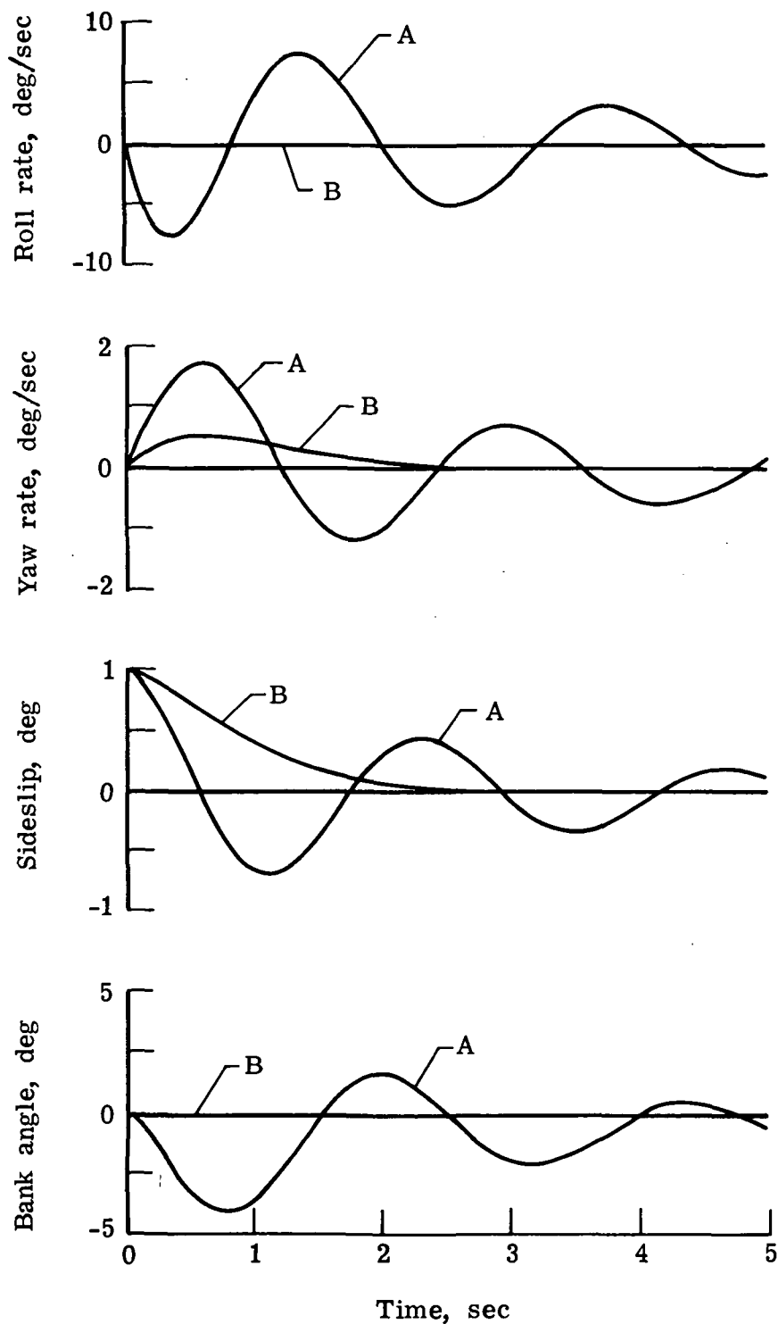
(a) Flight condition 1 (nominal cruise).
