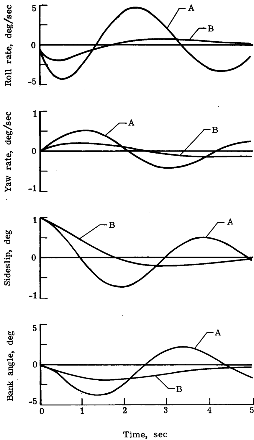
(b) Flight condition 17 (landing approach).
