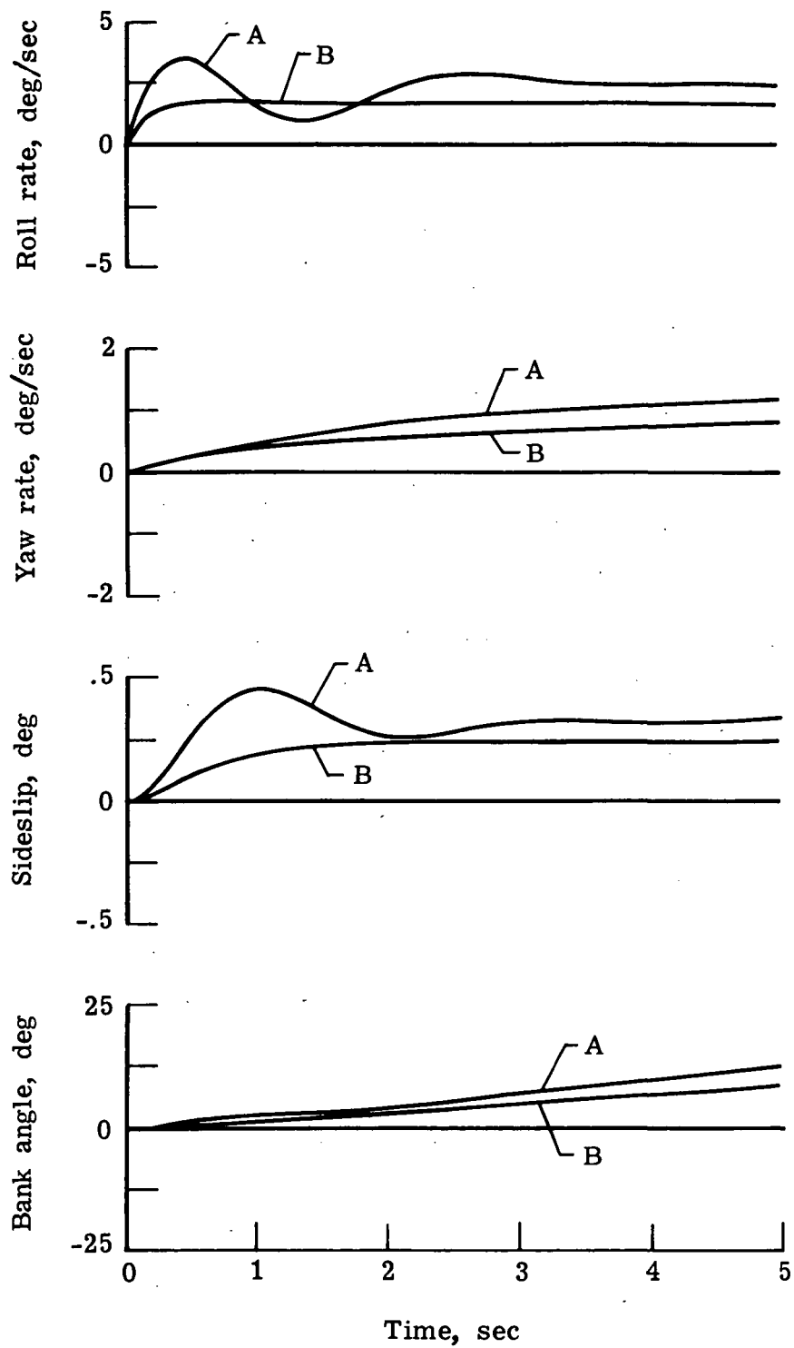
(c) Flight condition 20 (high angle of attack).
