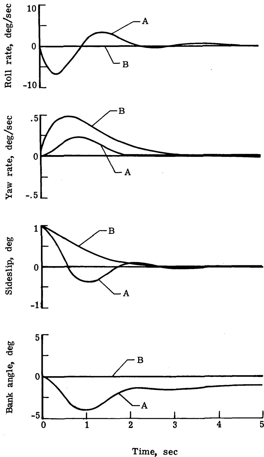
(c) Flight condition 20 (high angle of attack).
