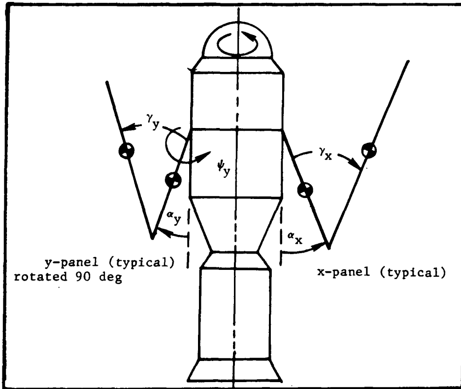
Figure 1. Spacecraft Schematic
