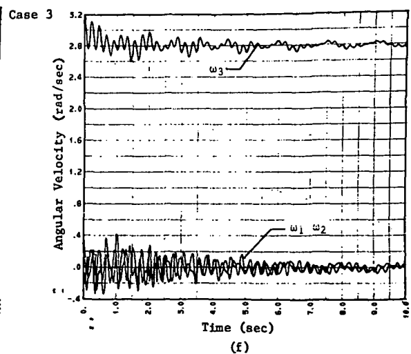
Figure 5. Principal Inertias and Principal Axes Angular Velocity Components
