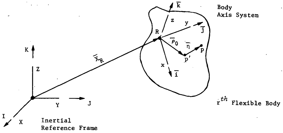
Figure 3. The r^{th} flexible body.
