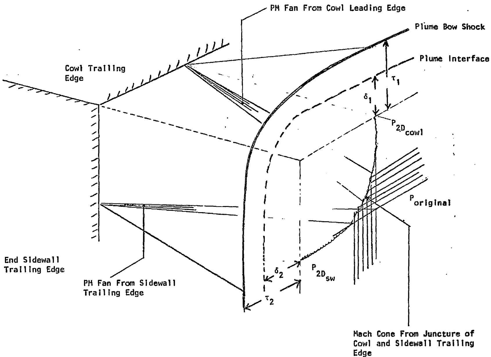
FIGURE 28. UNDEREXPANDED EXHAUST CORNER INTERACTION FLOWFIELD
