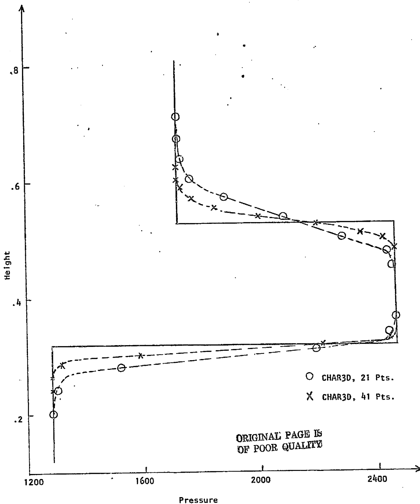
FIGURE 35. DOUBLE WEDGE INLET, PRESSURE PROFILES AT x = 1.16
