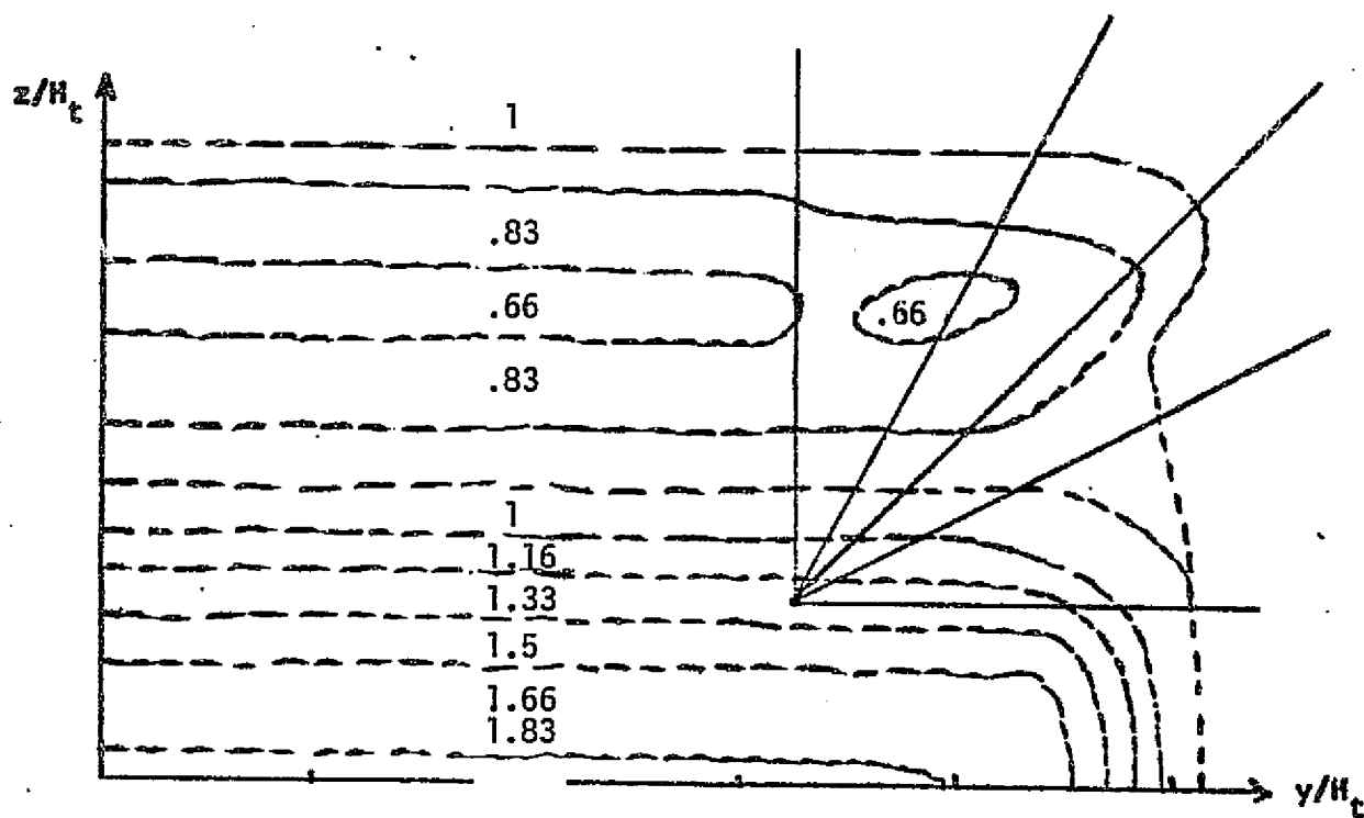
FIGURE 61. SINGLE MODULE ISOBARS AT x/H_t = 3.75
