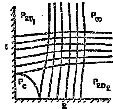
Figure 48. Results for 5° expansion corner. P_c is corner pressure; P_{2D} is two-dimensional wall pressure.
