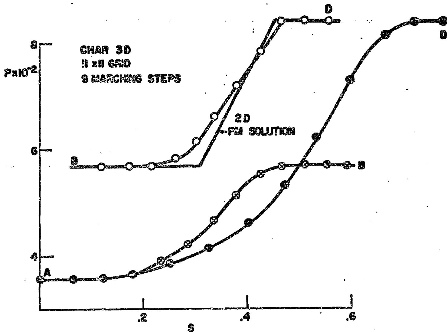
Figure 49.- Pressure distribution for 5^\circ expansion corner. PM means Prandtl-Meyer.
