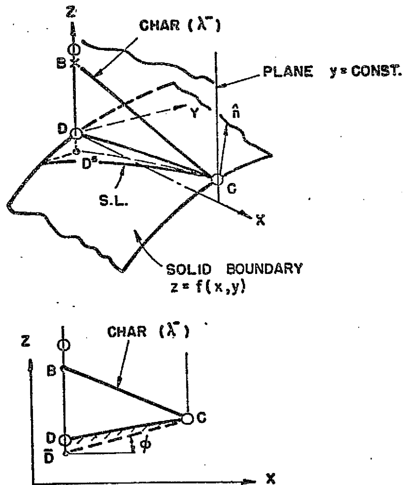
Figure 16. Solid boundary calculation.
