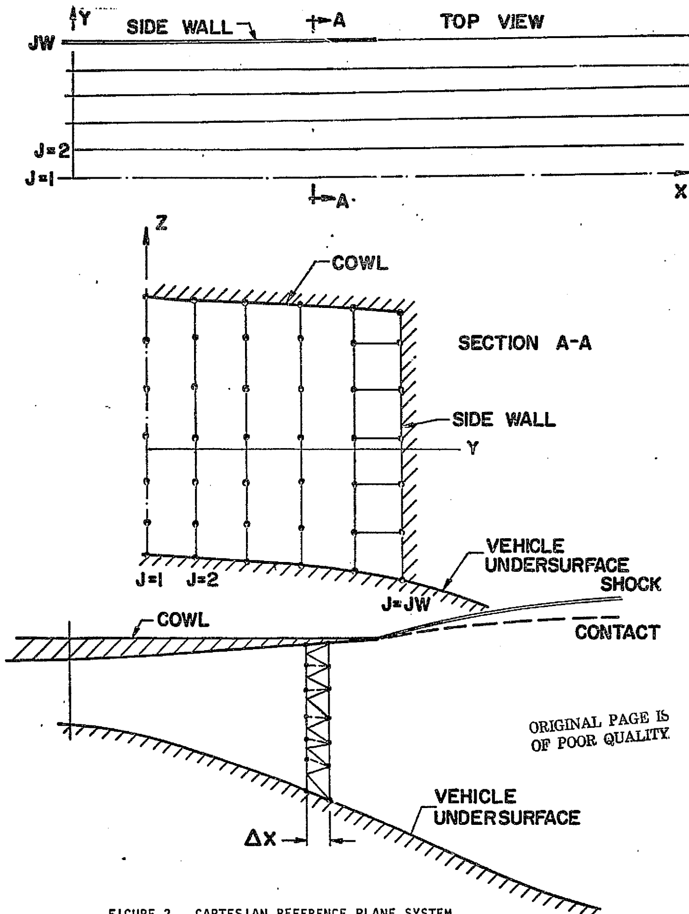
FIGURE 2. CARTESIAN REFERENCE PLANE SYSTEM
