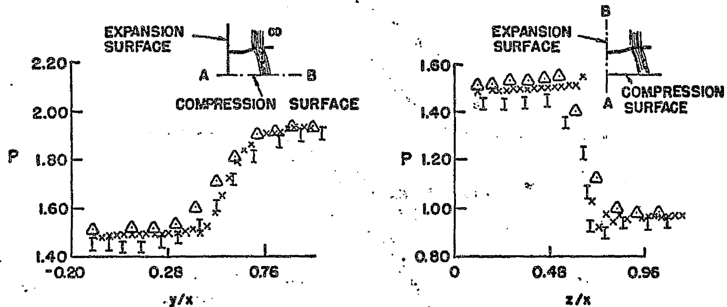
Figure 50. Results for an expansion-compression corner.
