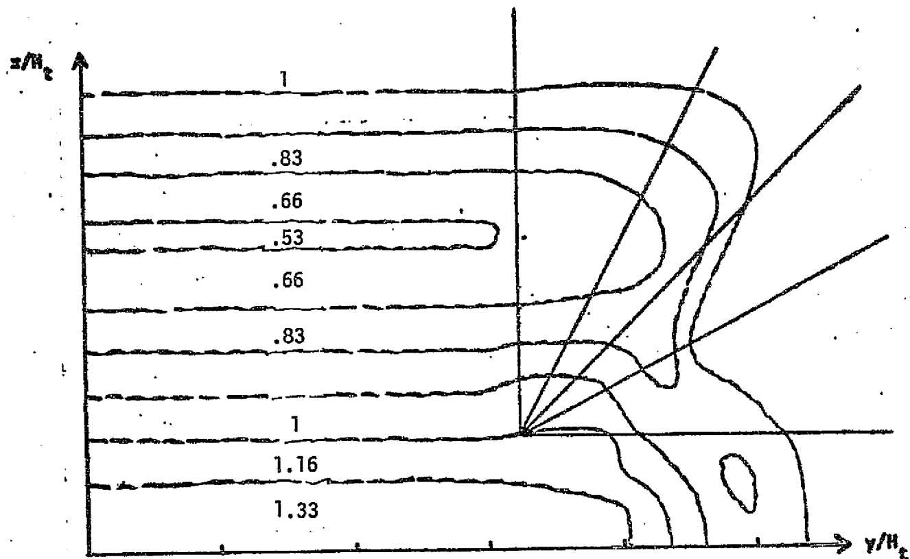
FIGURE 62. SINGLE MODULE ISOBARS AT x/H_t = 4.99
