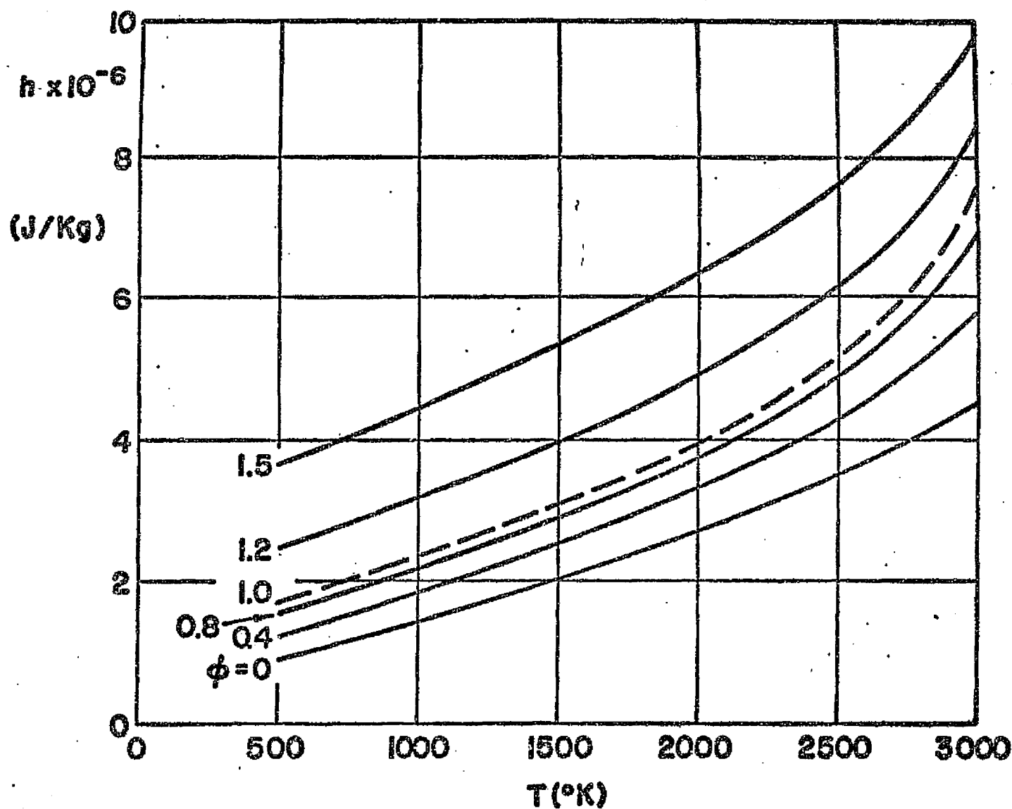
FIGURE A4. ENTHALPY AS A FUNCTION OF TEMPERATURE ( p=10^5 \text{ pa.} )
