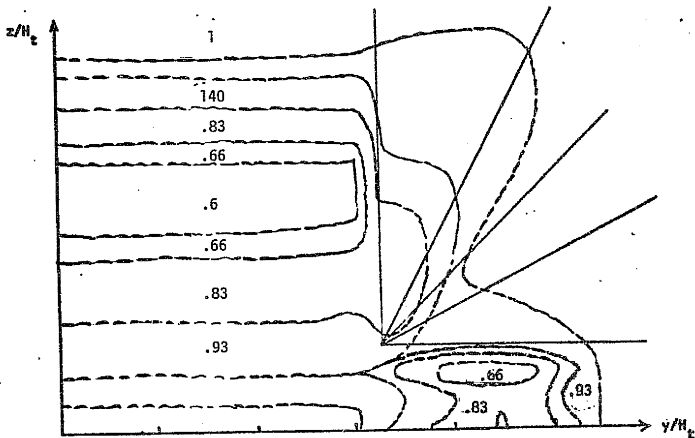
FIGURE 63. SINGLE MODULE ISOBARS AT x/H_t = 6.43
