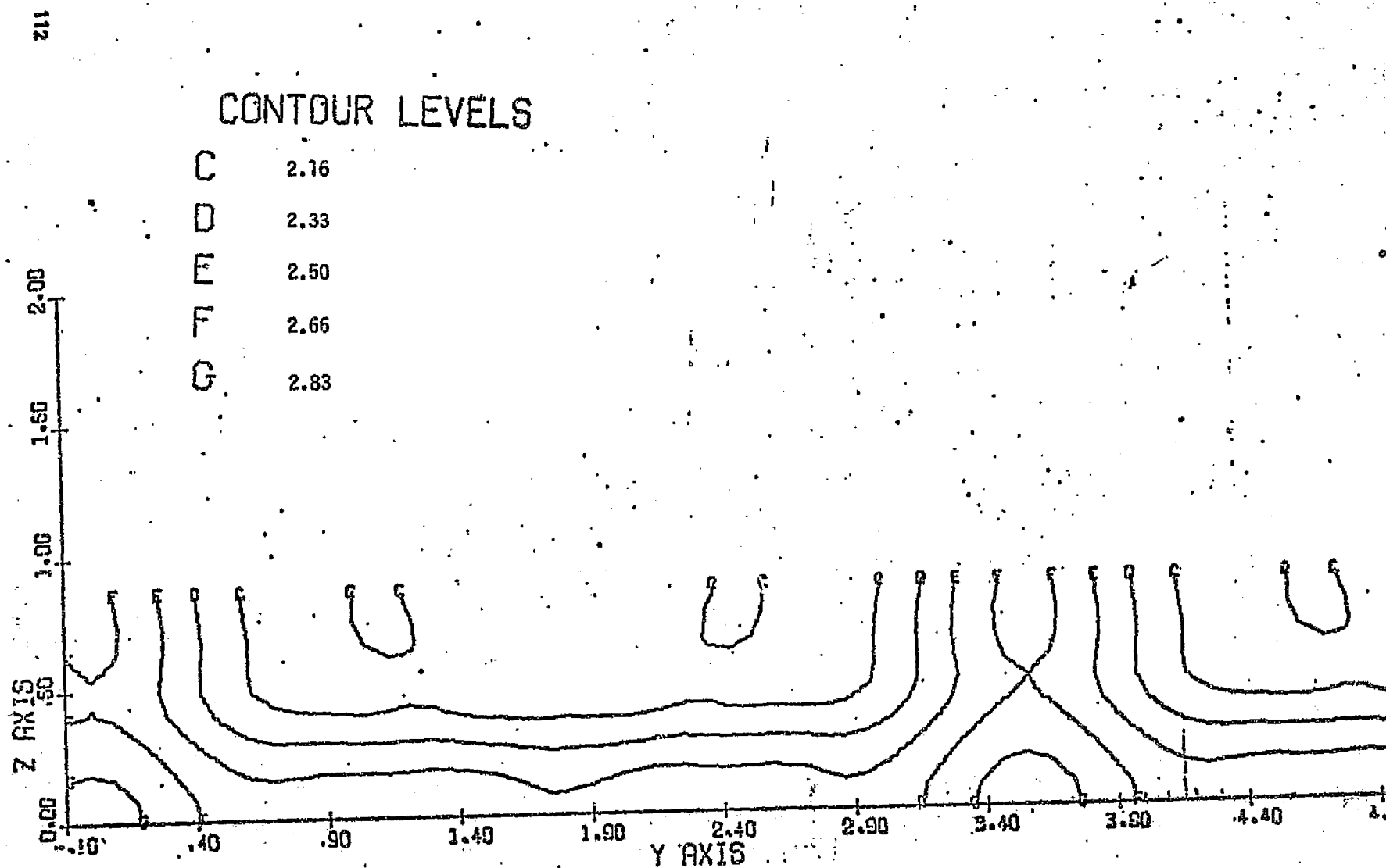
FIGURE 67. PRESSURE CONTOURS AT COWL EXIT PLANE ( x/z_c = 3.7 ), DOUBLE MODULE CASE
