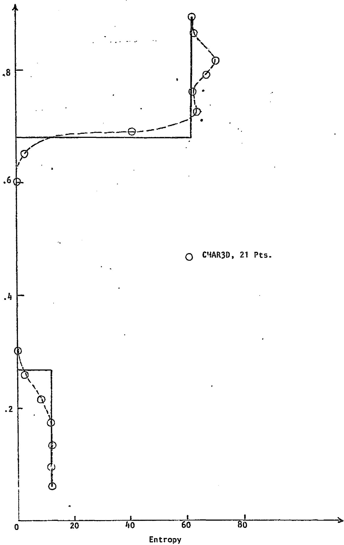
FIGURE 37. DOUBLE WEDGE INLET, ENTROPY PROFILE AT X = .64
