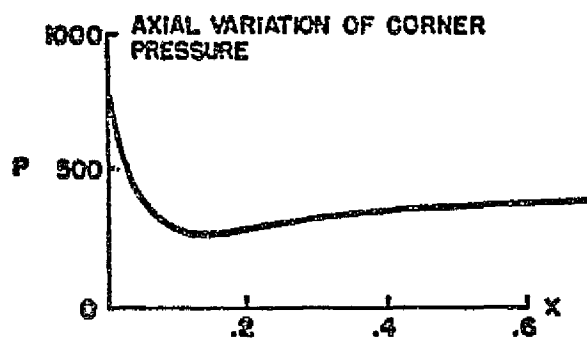
Figure 48. Results for 5° expansion corner. P_c is corner pressure; P_{2D} is two-dimensional wall pressure.
