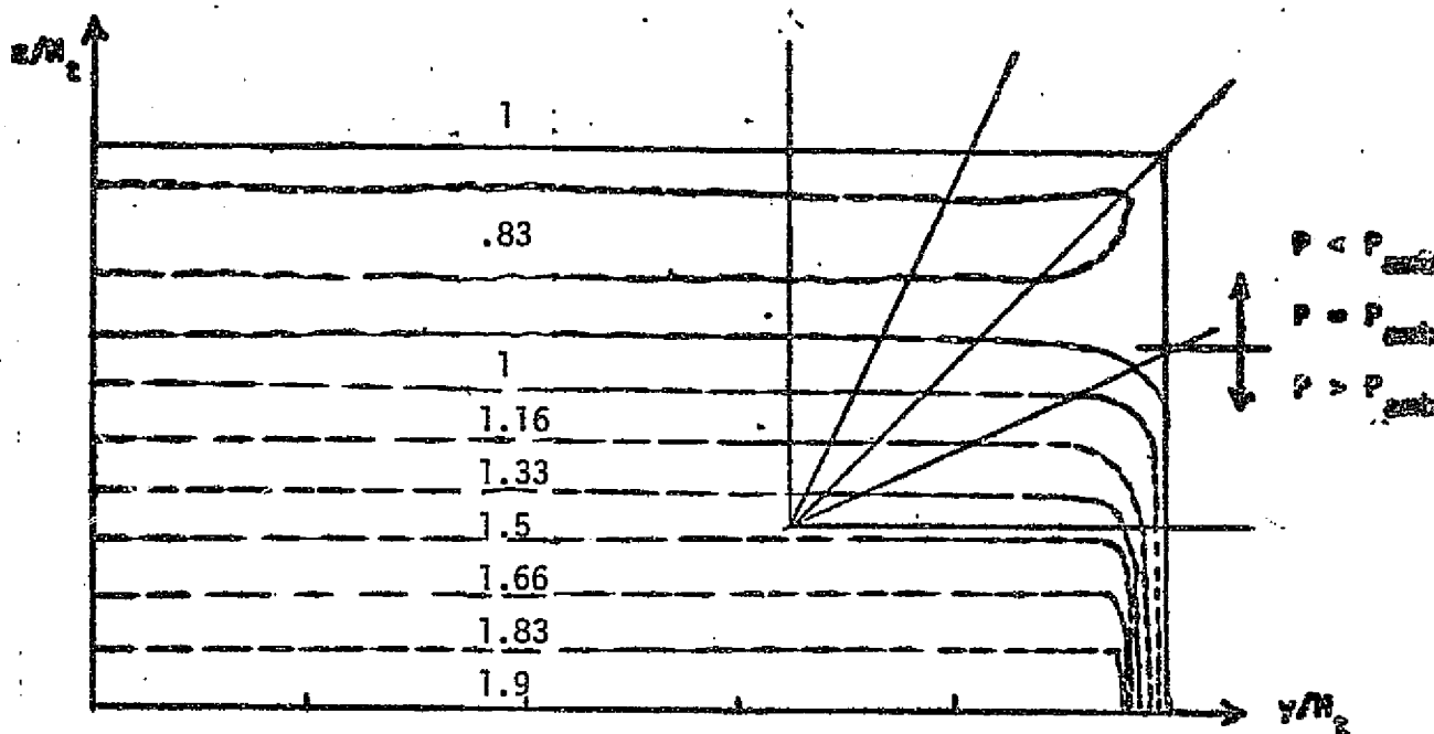
FIGURE 60. SINGLE MODULE ISOBARS AT x/H_t = 3.04
