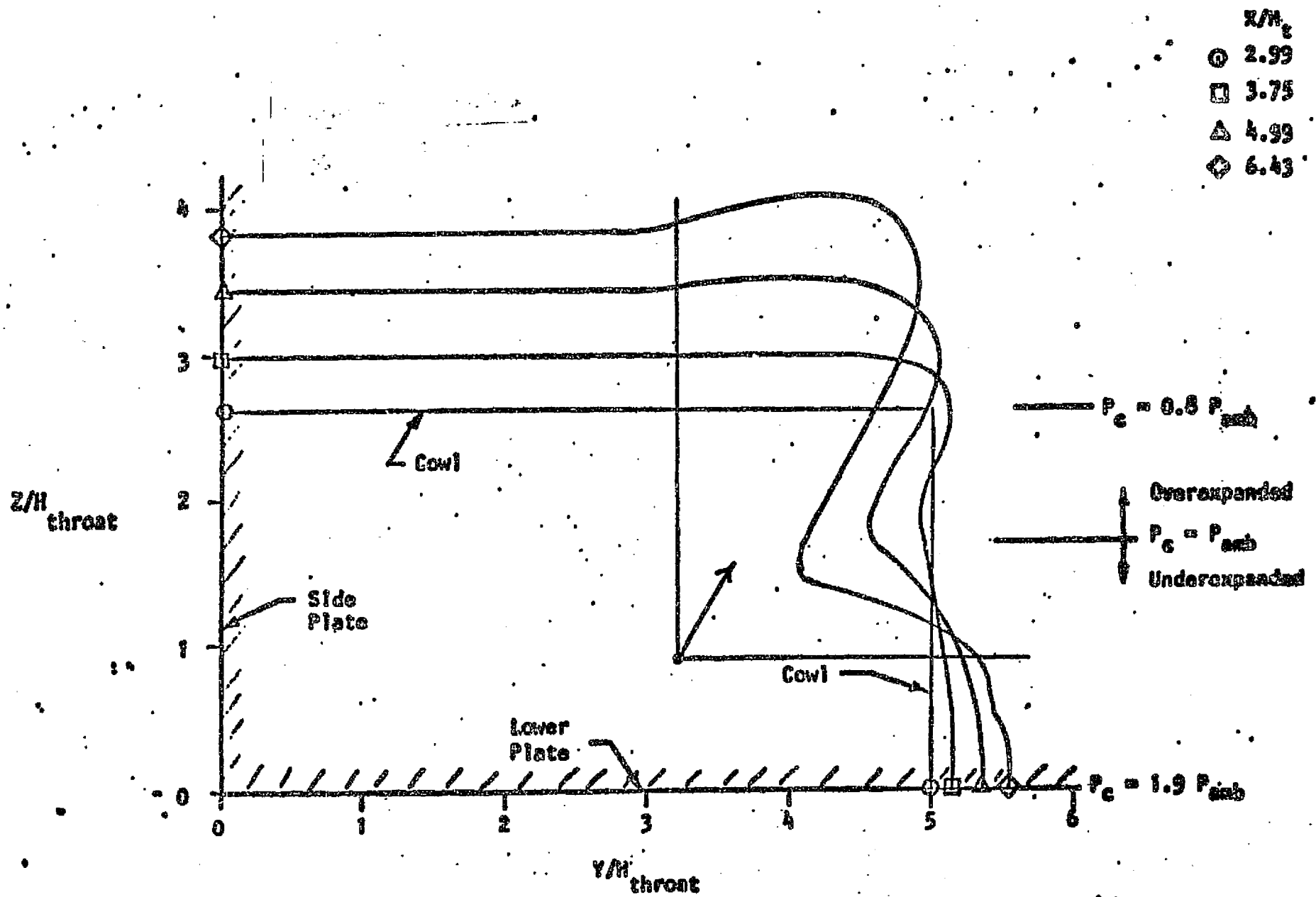
FIGURE 58. SINGLE MODULE, INTERFACE LOCATIONS
