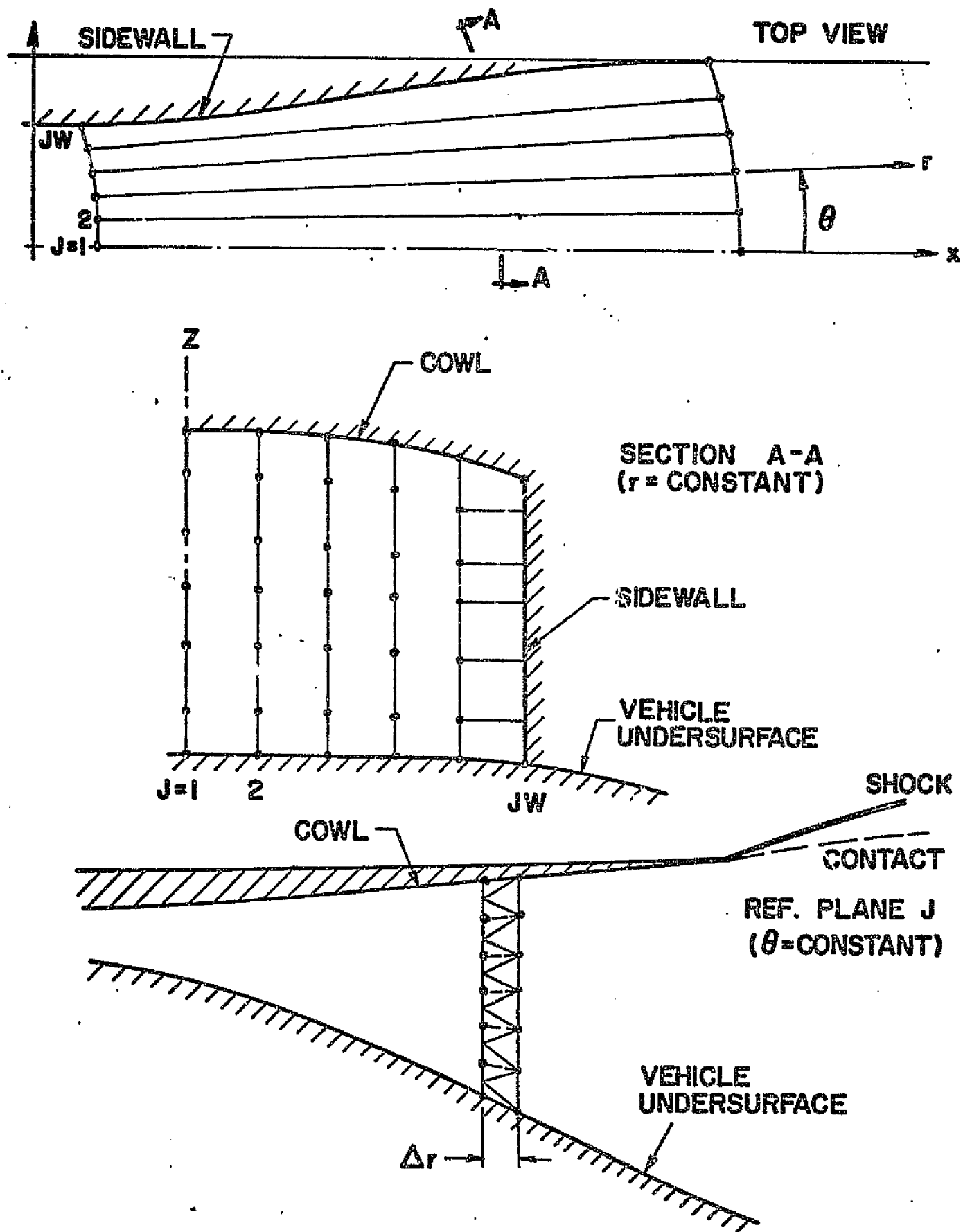
FIGURE 4. LINE SOURCE REFERENCE PLANE SYSTEM
