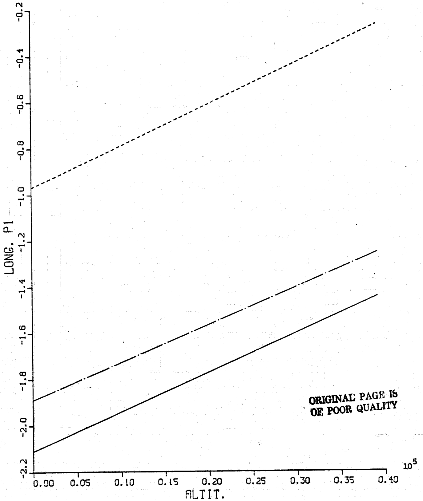
Fig. A.11 LONG. P1 VS. ALTIT. (Newton-Raphson IAS)
