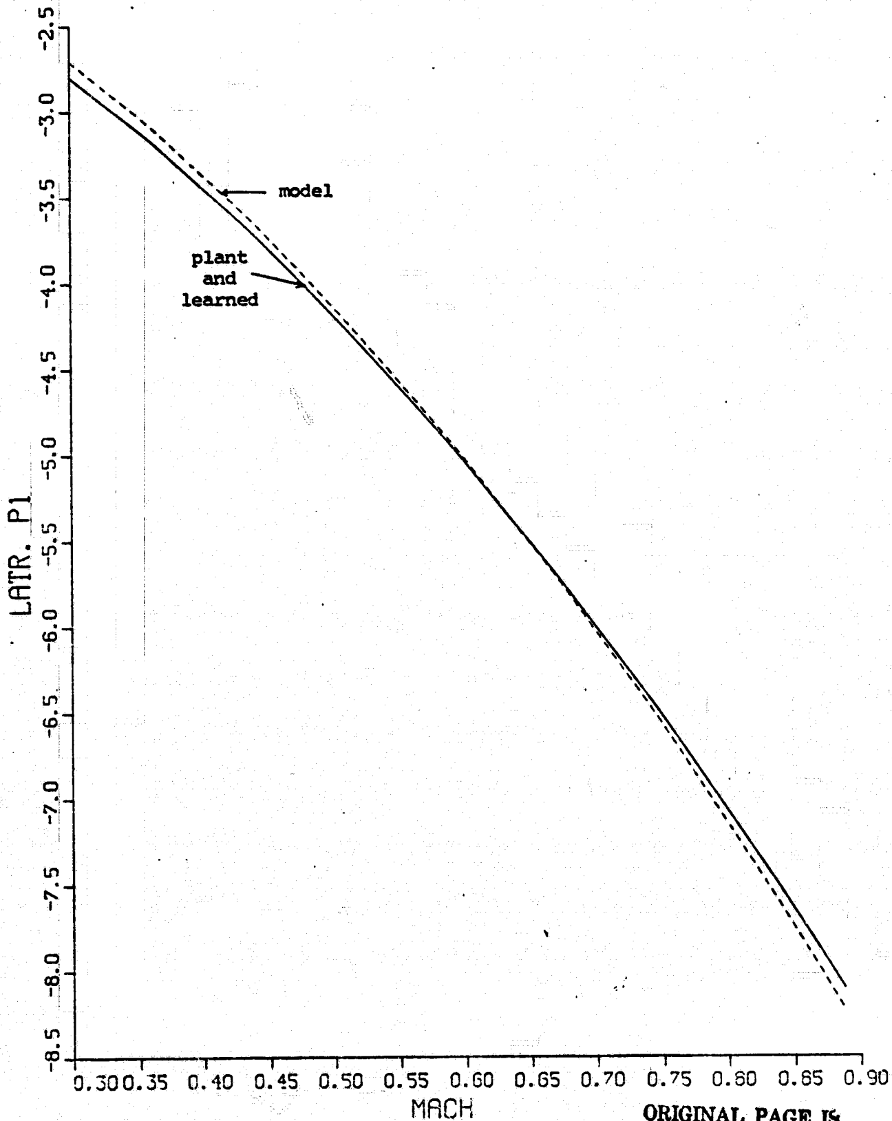
Fig. 6.2 LAIR. P1 VS. MACH (Newton-Raphson IAS)
