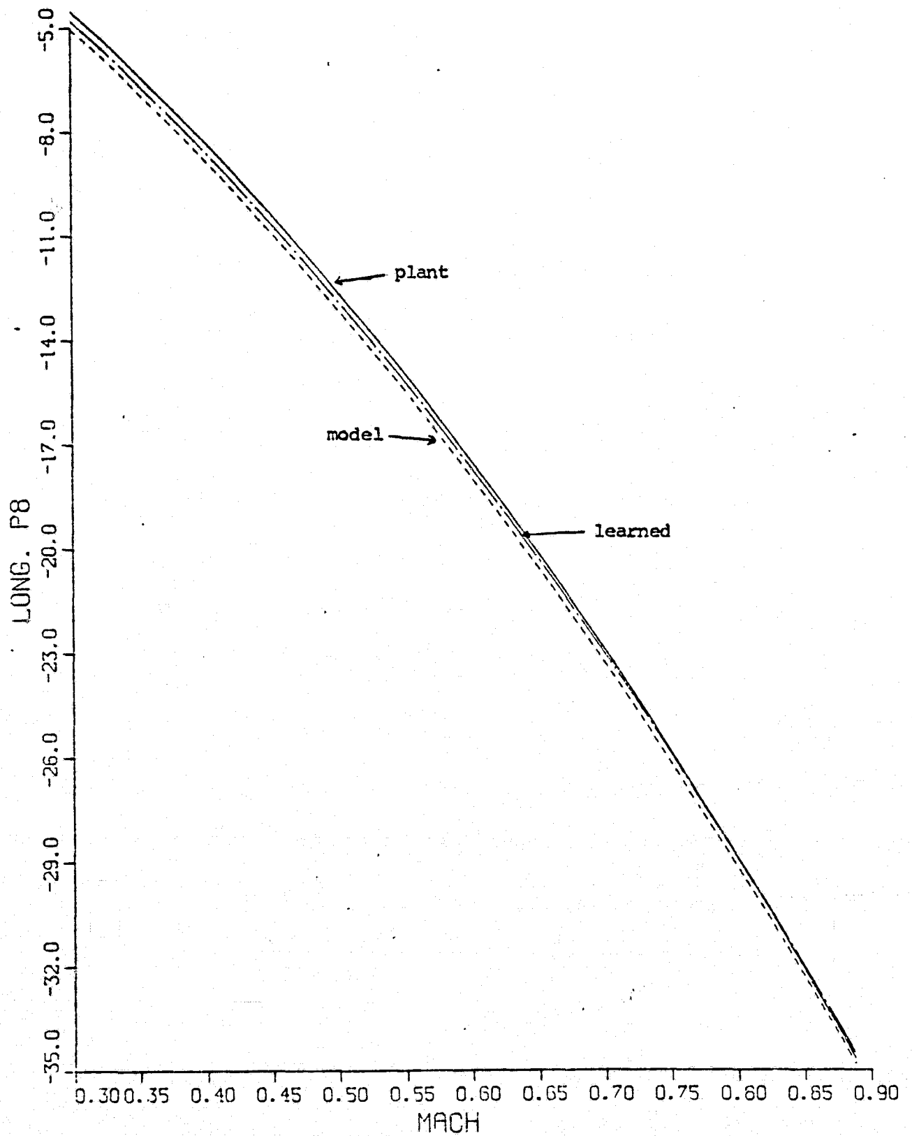
Fig. 4.7 LONG. P8 VS. MACH (Newton-Raphson IAS)
