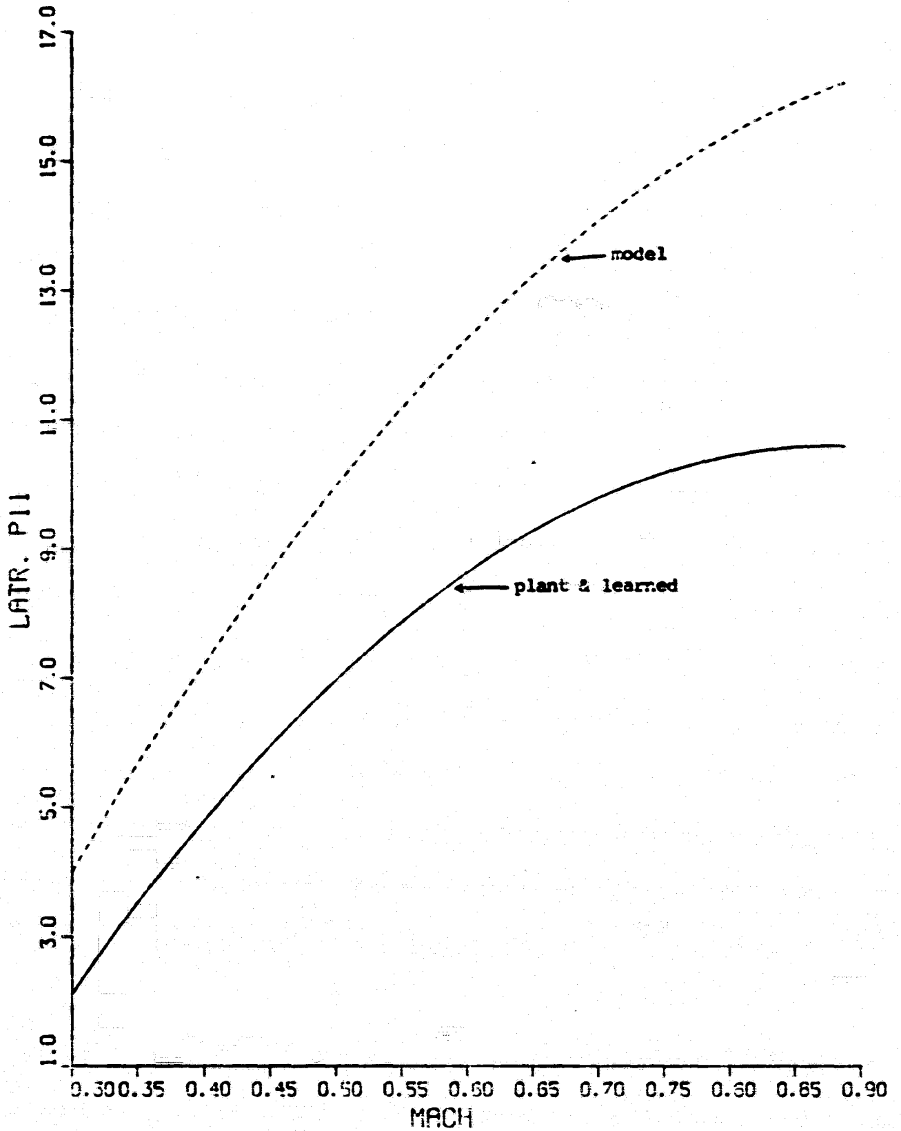
Fig. 4.13 LATR. P11 VS. MACH (Newton-Raphson IAS)
