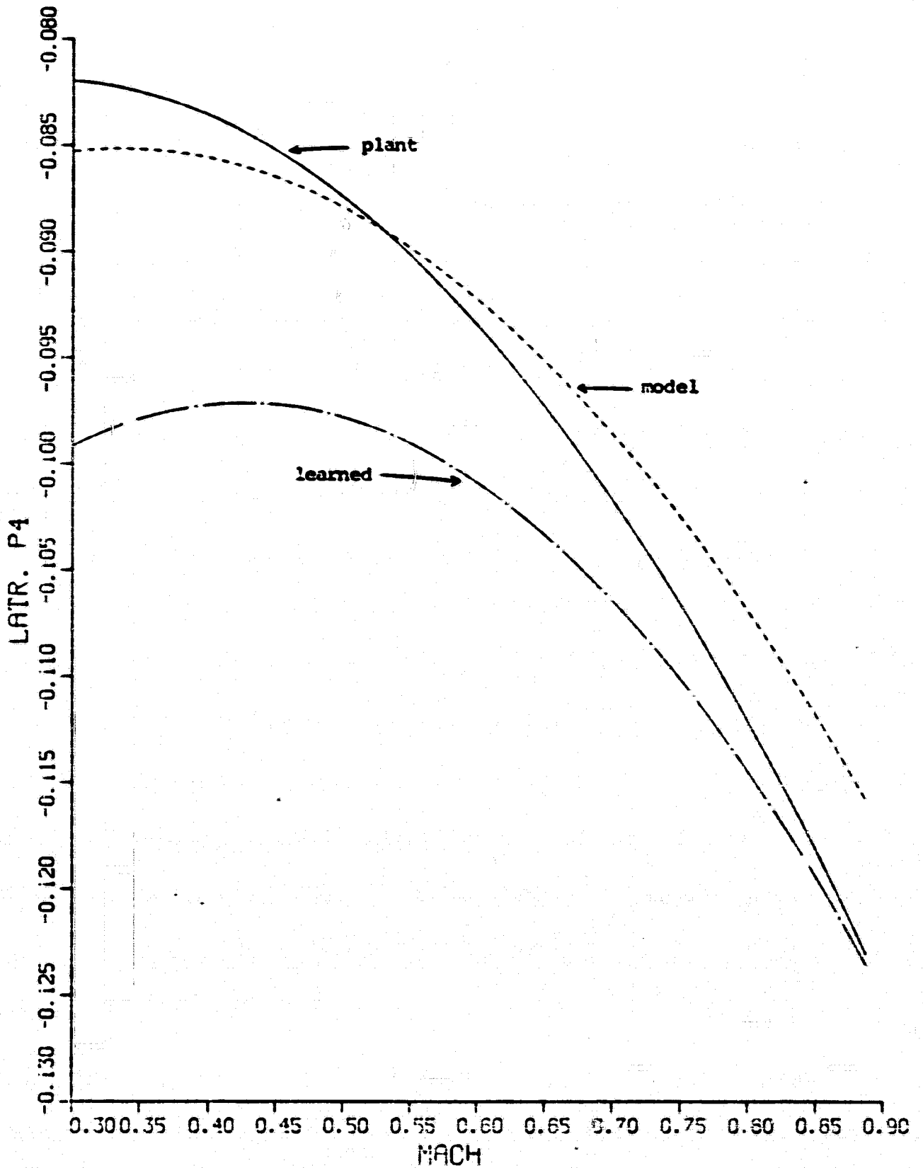
Fig. 4.12 LATR. P4 VS. MACH (Newton-Raphson IAS)
