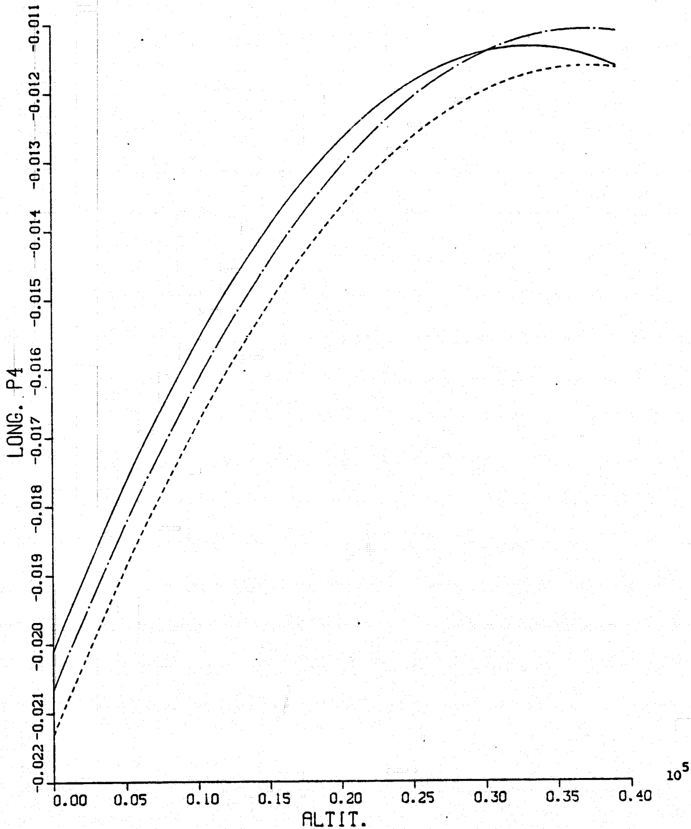
Fig. A.14 LONG. P4 VS. ALTIT. (Newton-Raphson IAS)
