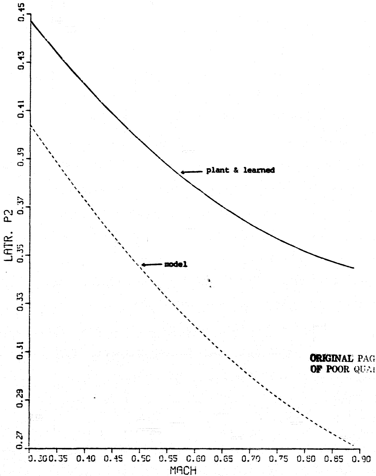
Fig. 4.11 LATR. P2 VS. MACH (Newton-Raphson IAS)
