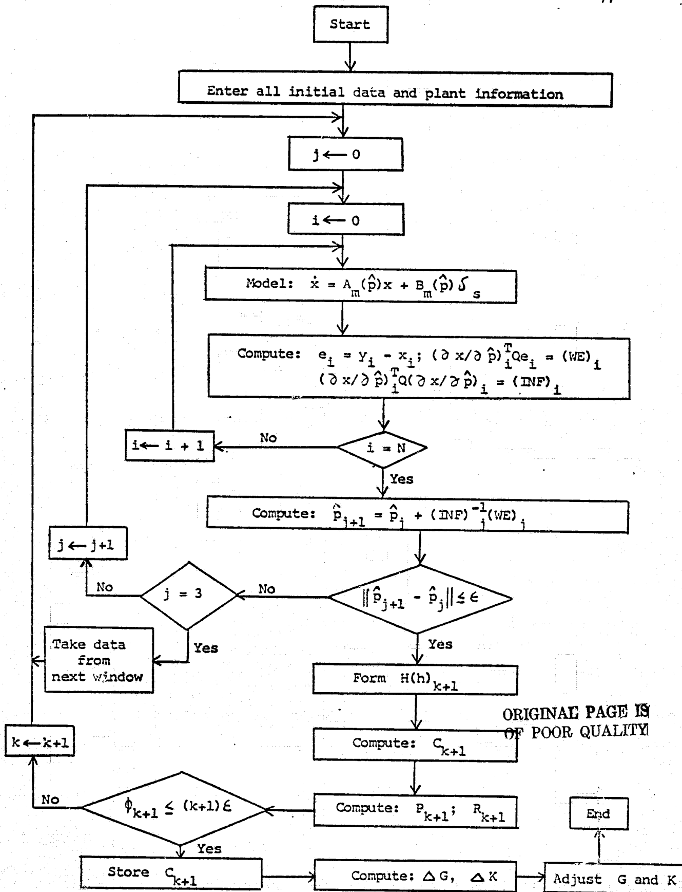
Fig. 4.1b Logic Flow Diagram (IAS - Newton-Raphson Method)
