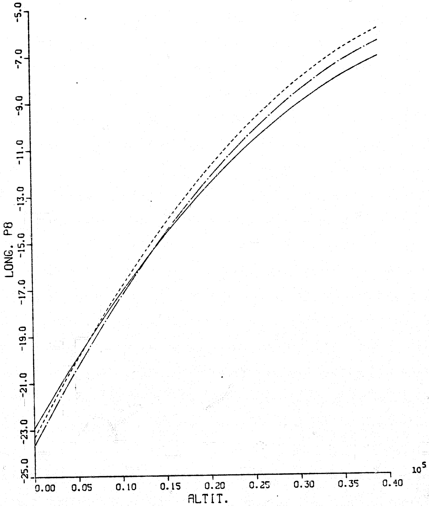
Fig. A.18 LONG. P8 VS. ALTIT. (Newton-Raphson IAS)
