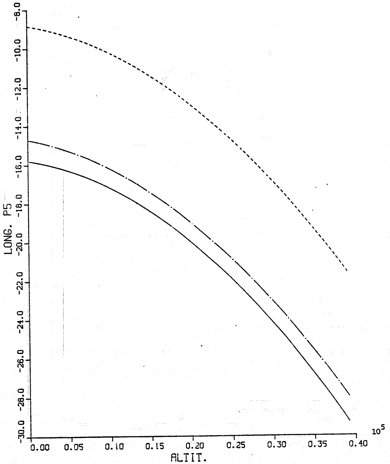
Fig. A.15 LONG. P5 VS. ALTIT. (Newton-Raphson IAS)
