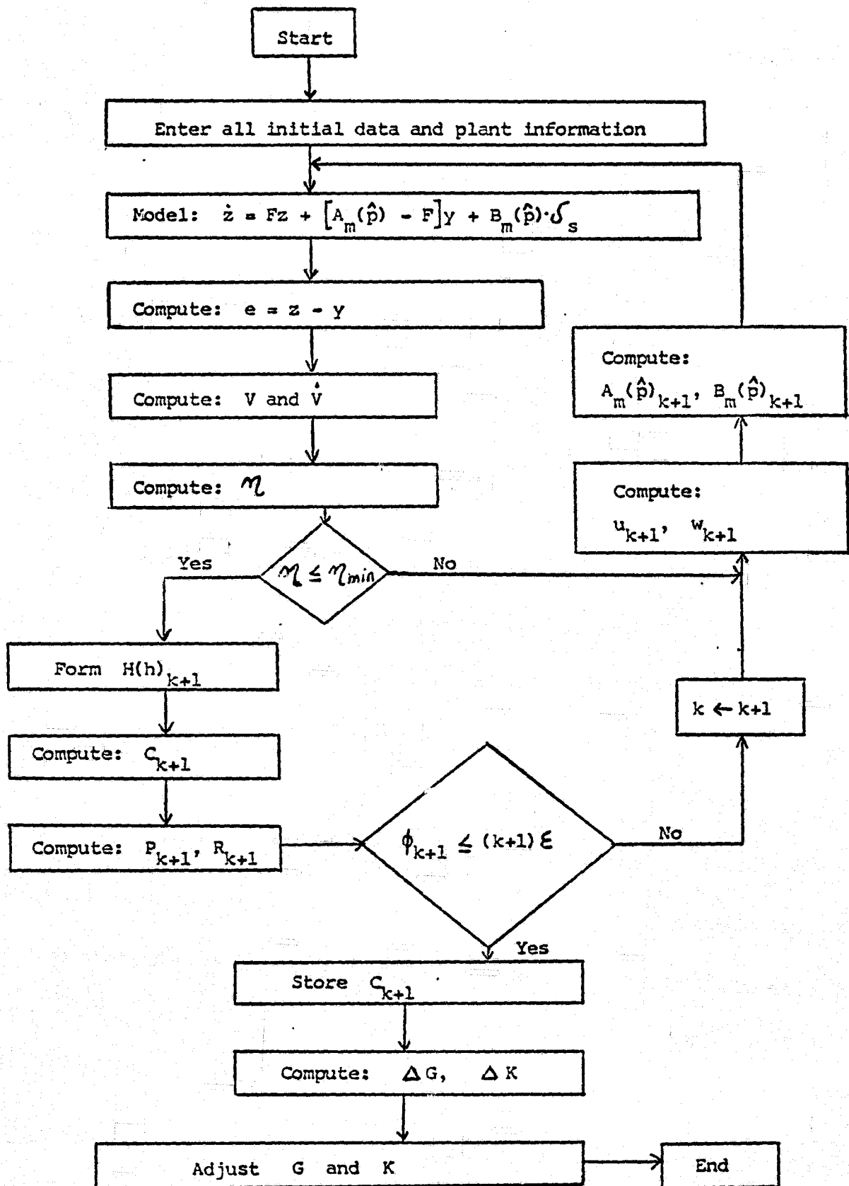
Fig. 4.1a Logic Flow Diagram. (IAS - Liapunov Method)
