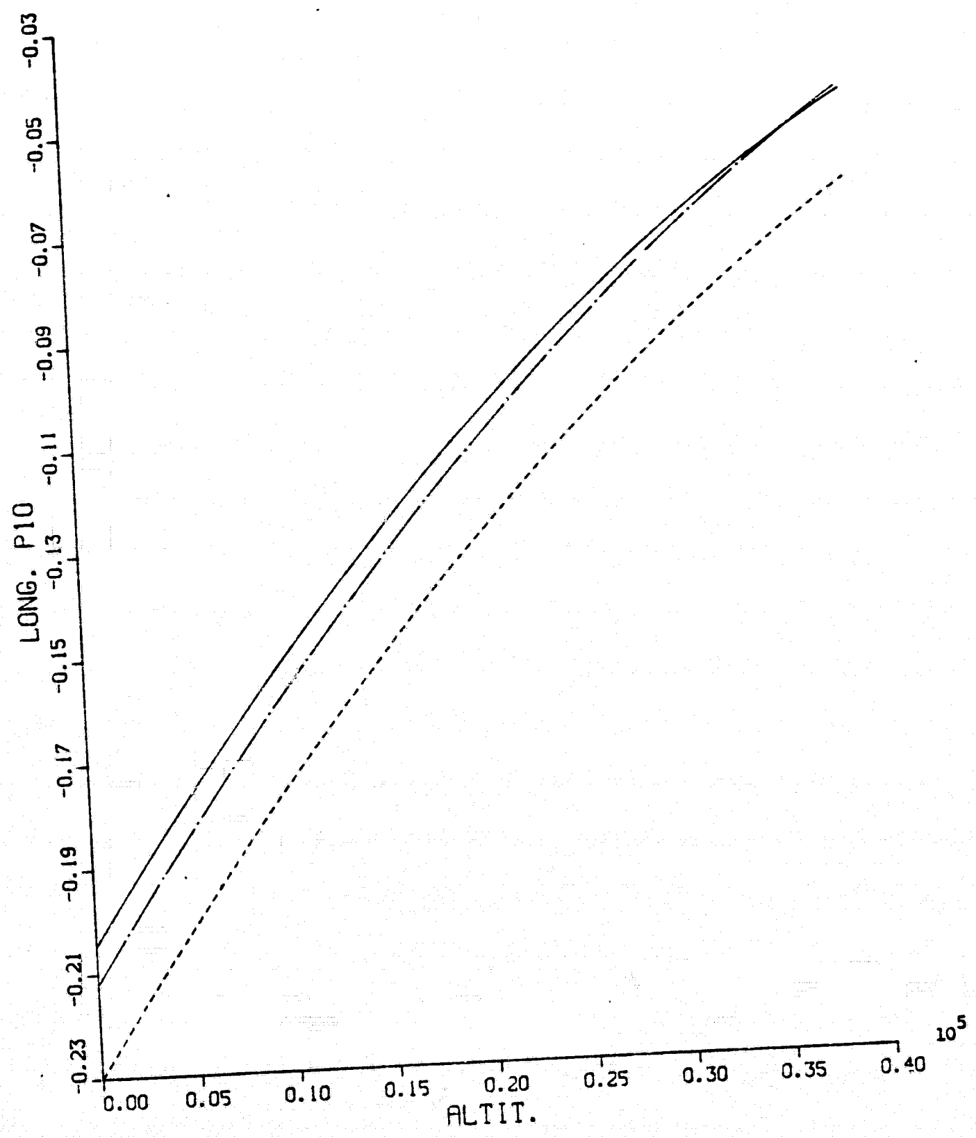
Fig. A.20 LONG. P10 VS. ALTIT. (Newton-Raphson IAS)
