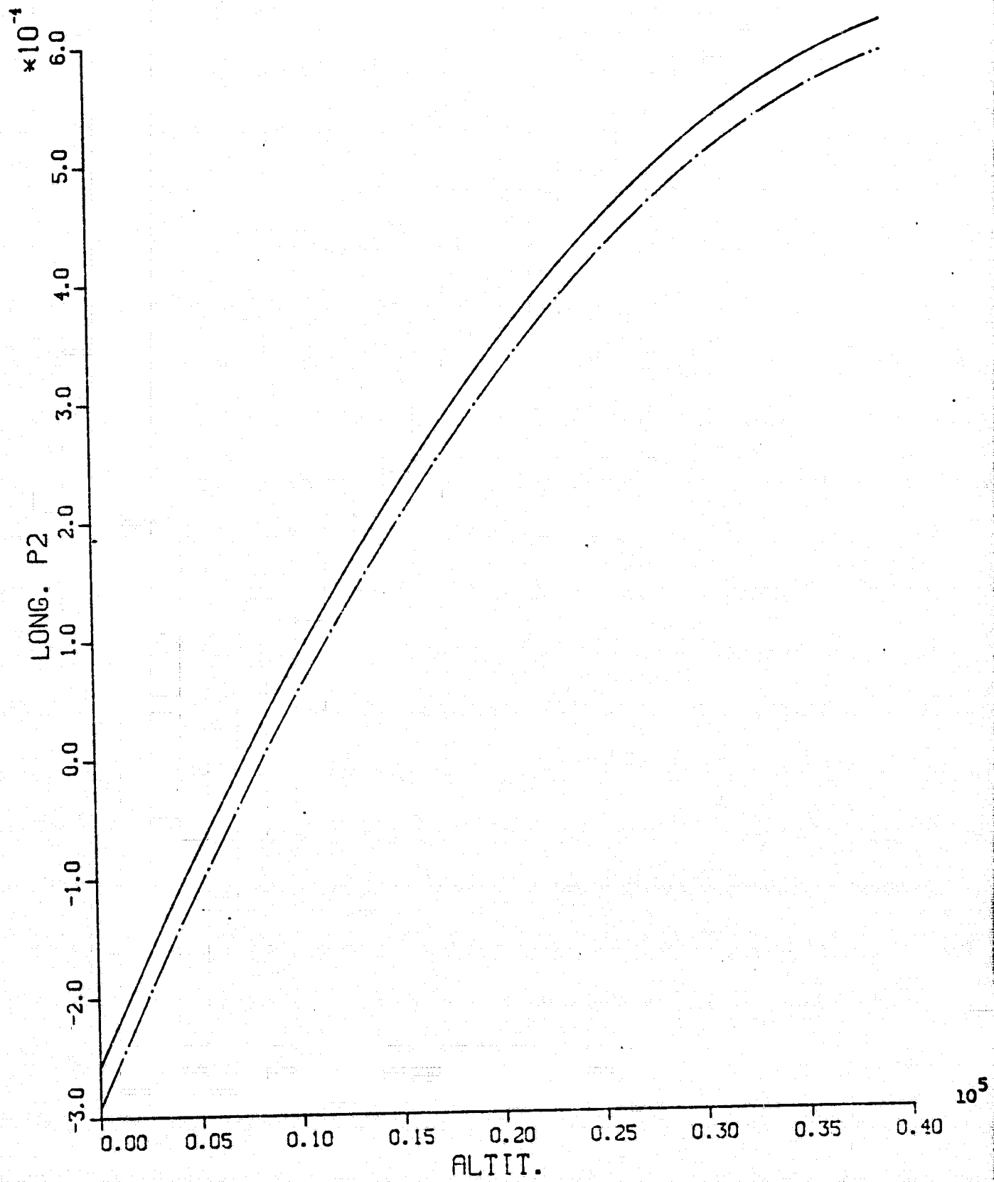
Fig. A.12 LONG. P2 VS. ALTIT. (Newton-Raphson IAS)
