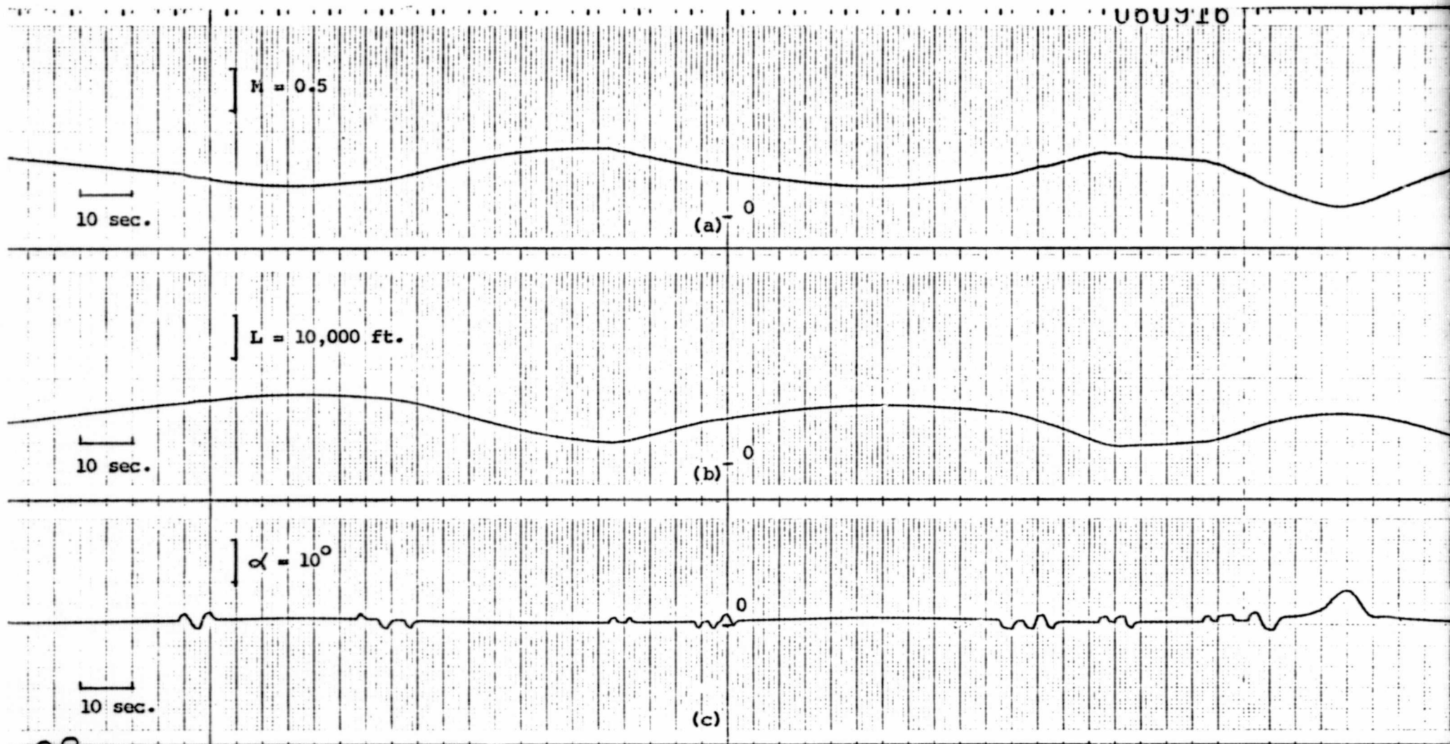
Fig. 5.4 Real-time simulation time histories of the longitudinal dynamics of F-8 DFEW aircraft (a) mach number (b) altitude (c) angle of attack.
