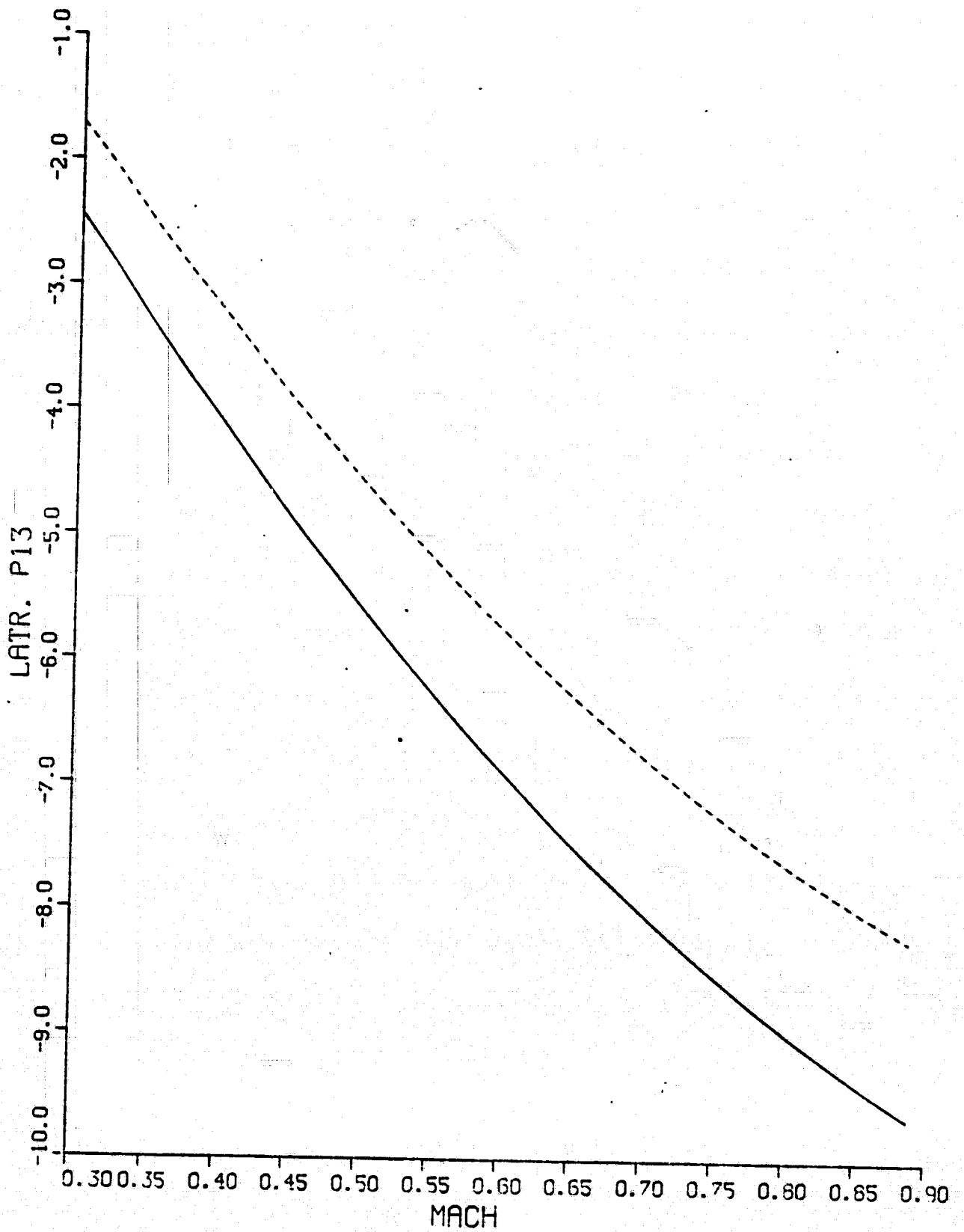
Fig. 6.3 LATR. P13 VS. MACH (Newton-Raphson Method)
