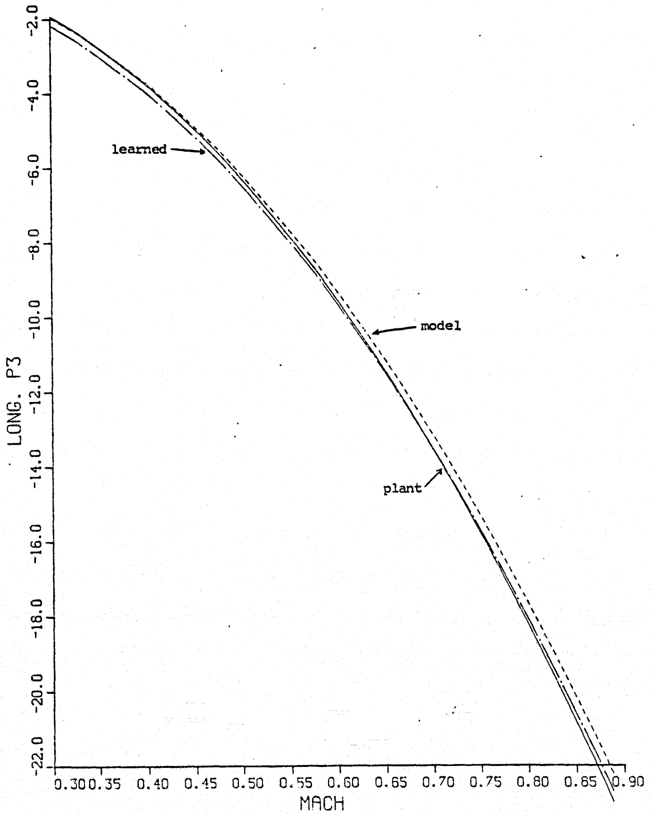
Fig. 4.6 LONG. P3 VS. MACH (Newton-Raphson IAS)
