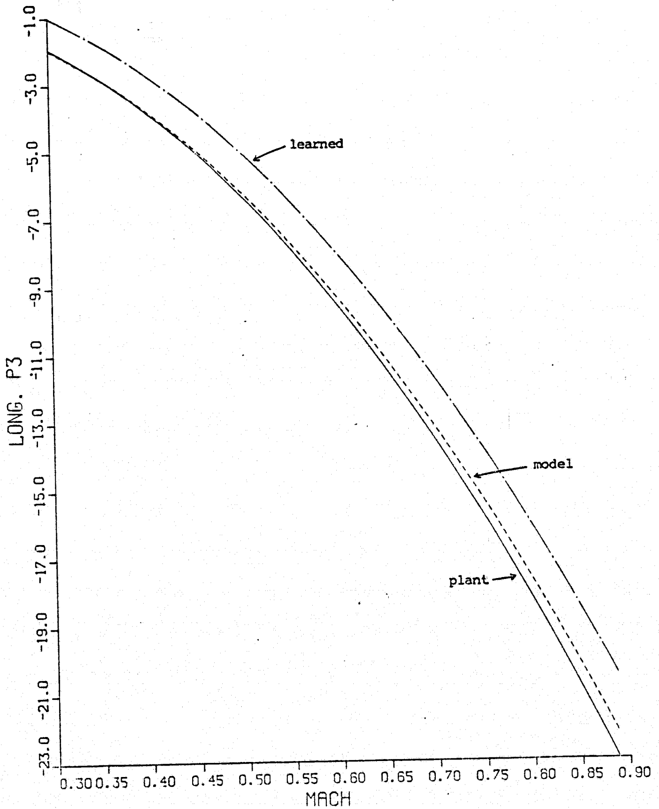
Fig. 4.3 LONG. P3 VS. MACH (Liapunov IAS)
