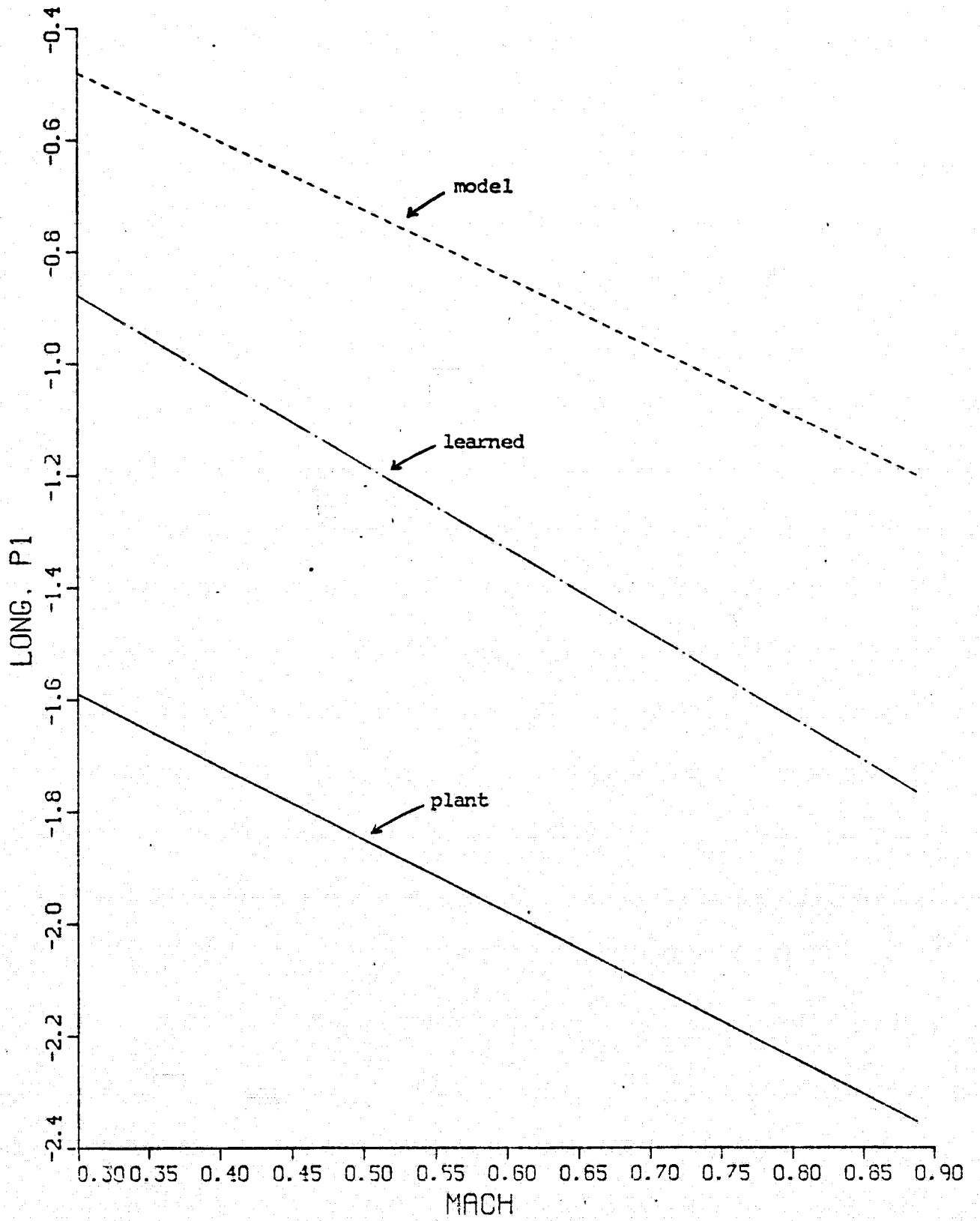
Fig. 4.2 LONG. P1 VS. MACH (Liapunov IAS)
