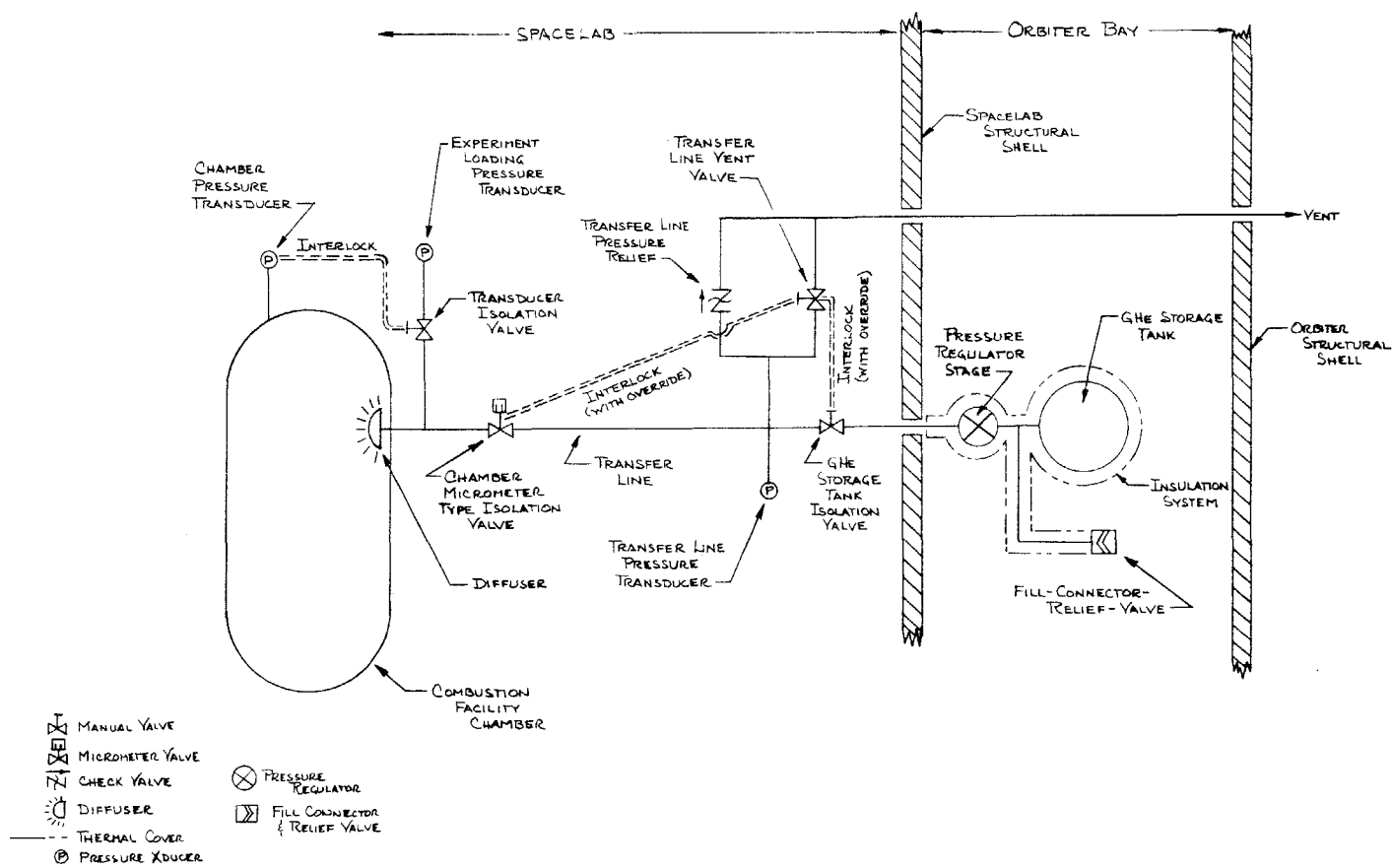
Figure 8. - Schematic of gaseous helium storage and supply subsystem.
