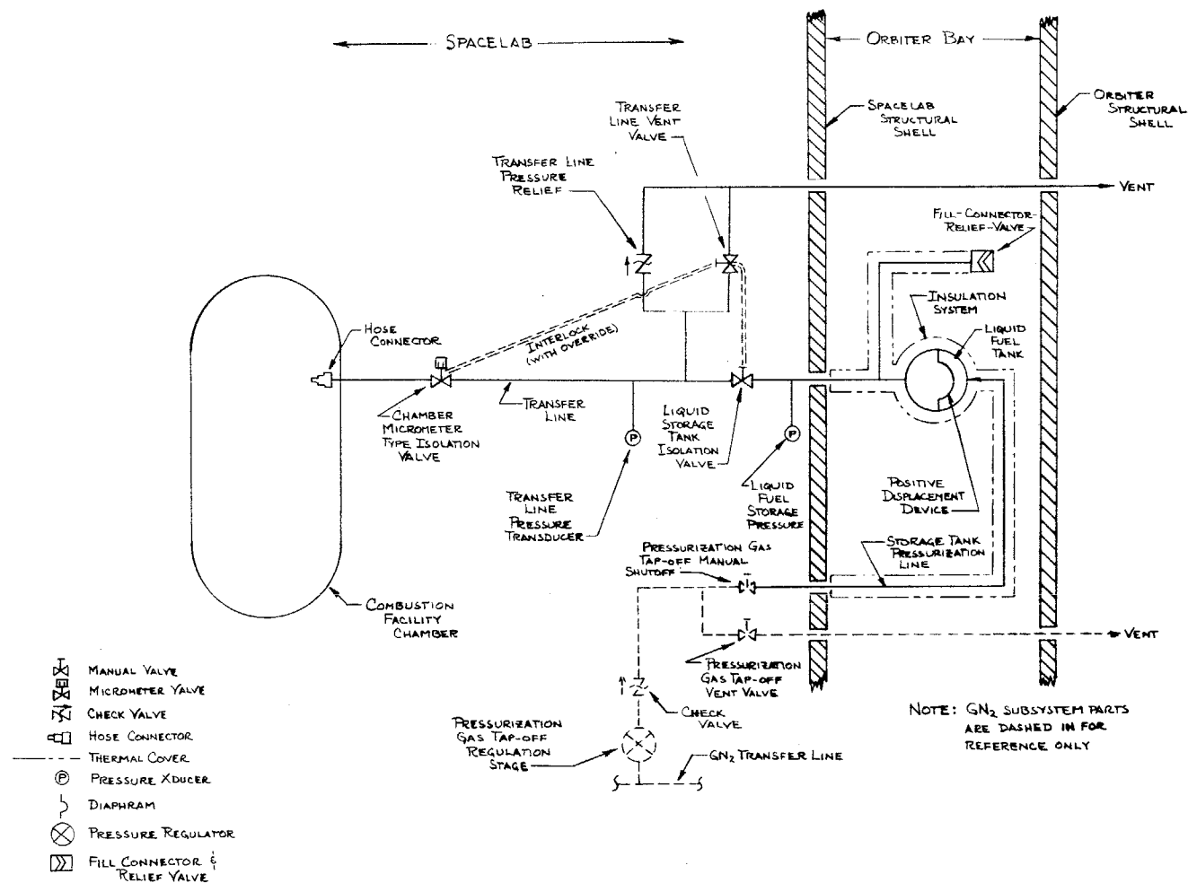
Figure 5. - Schematic of liquid-fuel storage and supply subsystem.
