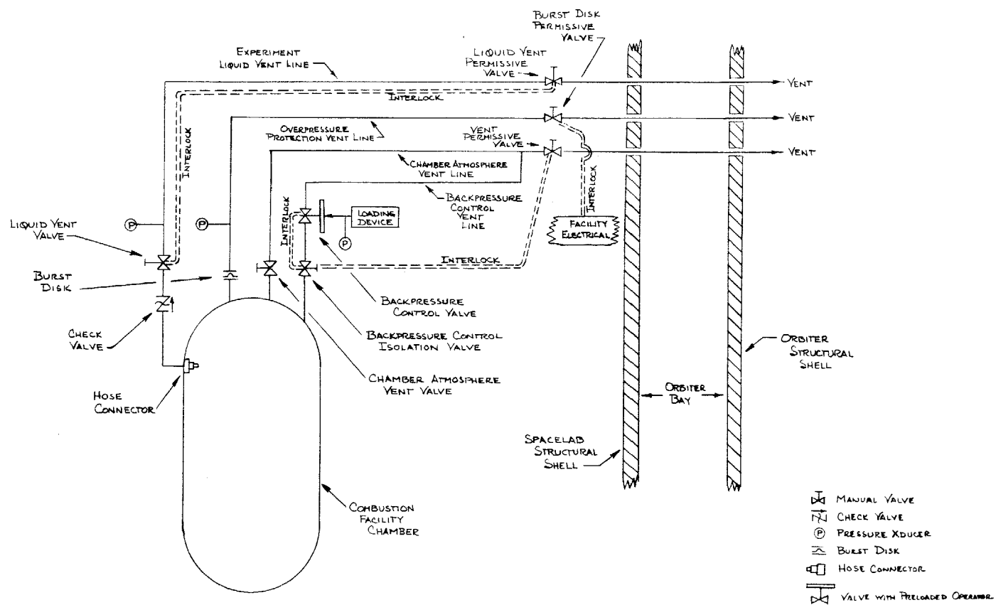
Figure 10. - Schematic of complete vent assembly.
