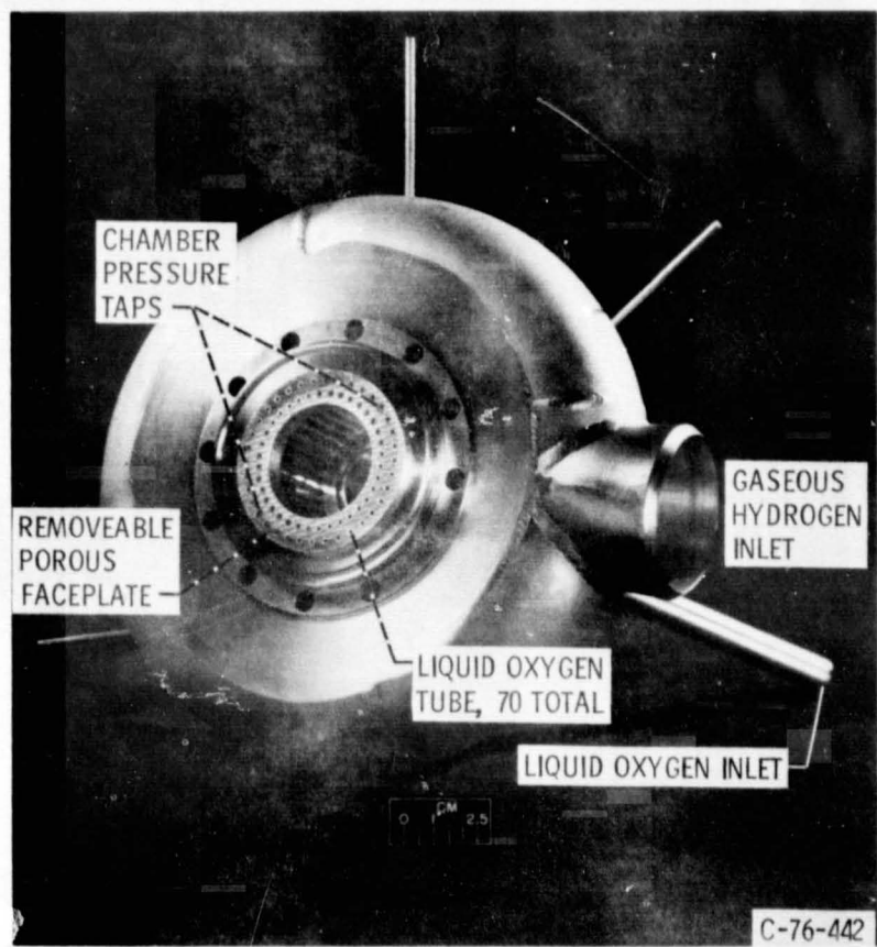
Figure 5. - Annular injector.
