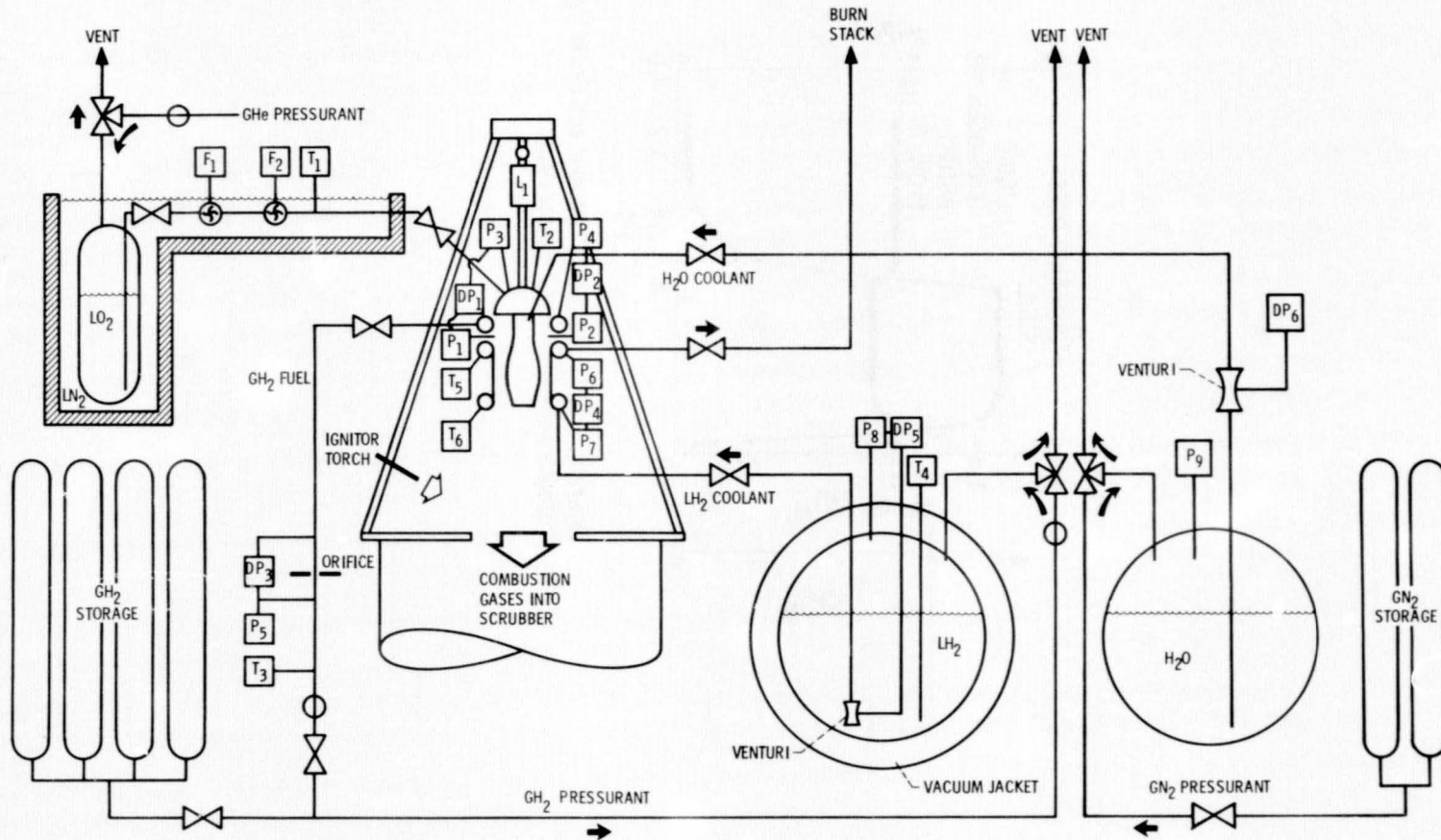
Figure 7. - Schematic of test facility.
