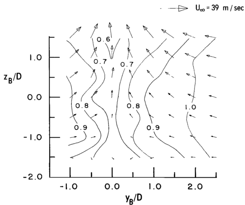
(b) Measured velocities, U_B/U_\infty and (\vec{V}_B + \vec{W}_B)/U_\infty .
