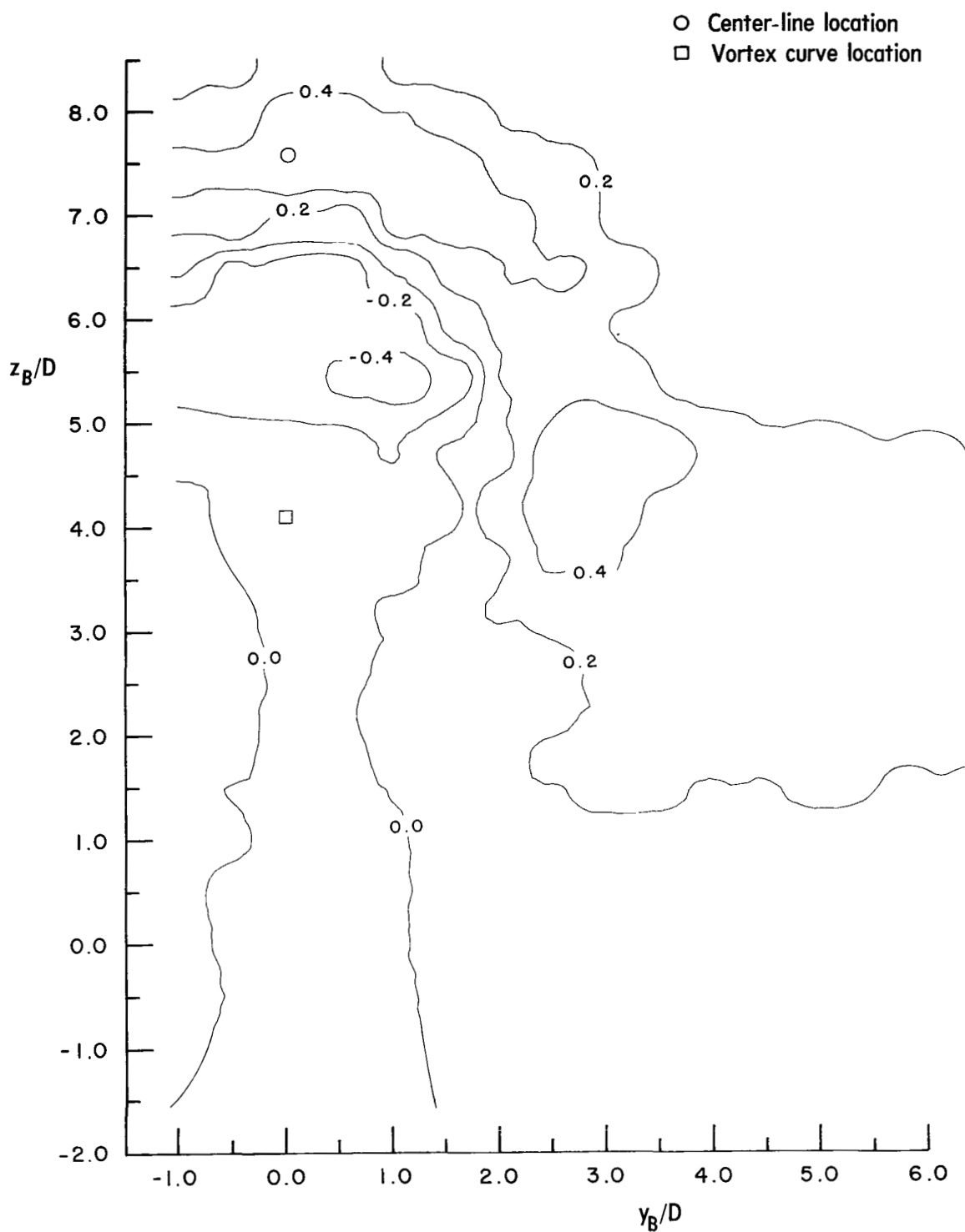
(a) Total-pressure coefficient C_{p,t} .
