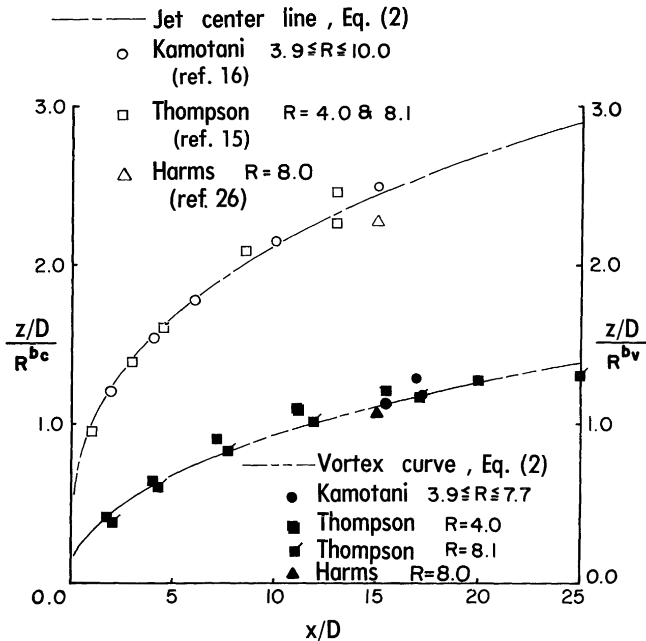
Figure 11.- Jet center line and vortex curve, comparison with other experiments.
