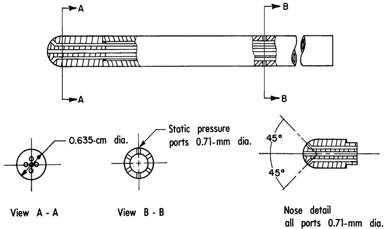
Figure 5.- Yaw-pitch probe.
