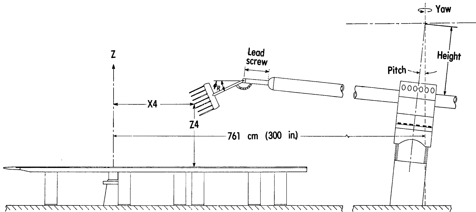
Figure B1.- Schematic of rake positioning system.
