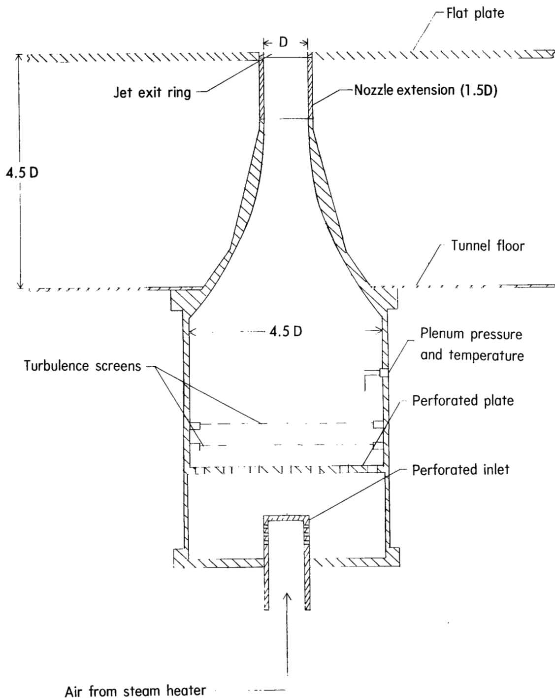
Figure 3.- Jet nozzle and plenum.
