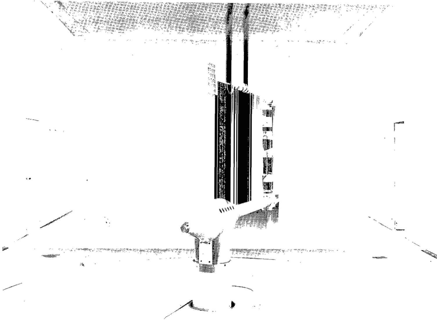
Figure 8.- Experimental arrangement in V/STOL tunnel for probe calibration.
