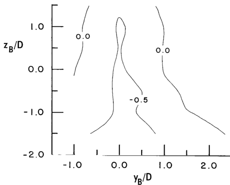
(a) Total-pressure coefficient C_{p,t} .
