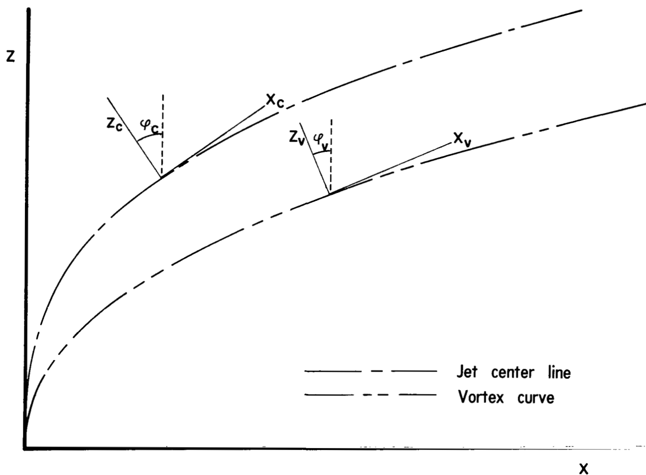
Figure 2.- Jet center line and vortex curve with associated coordinates systems.
