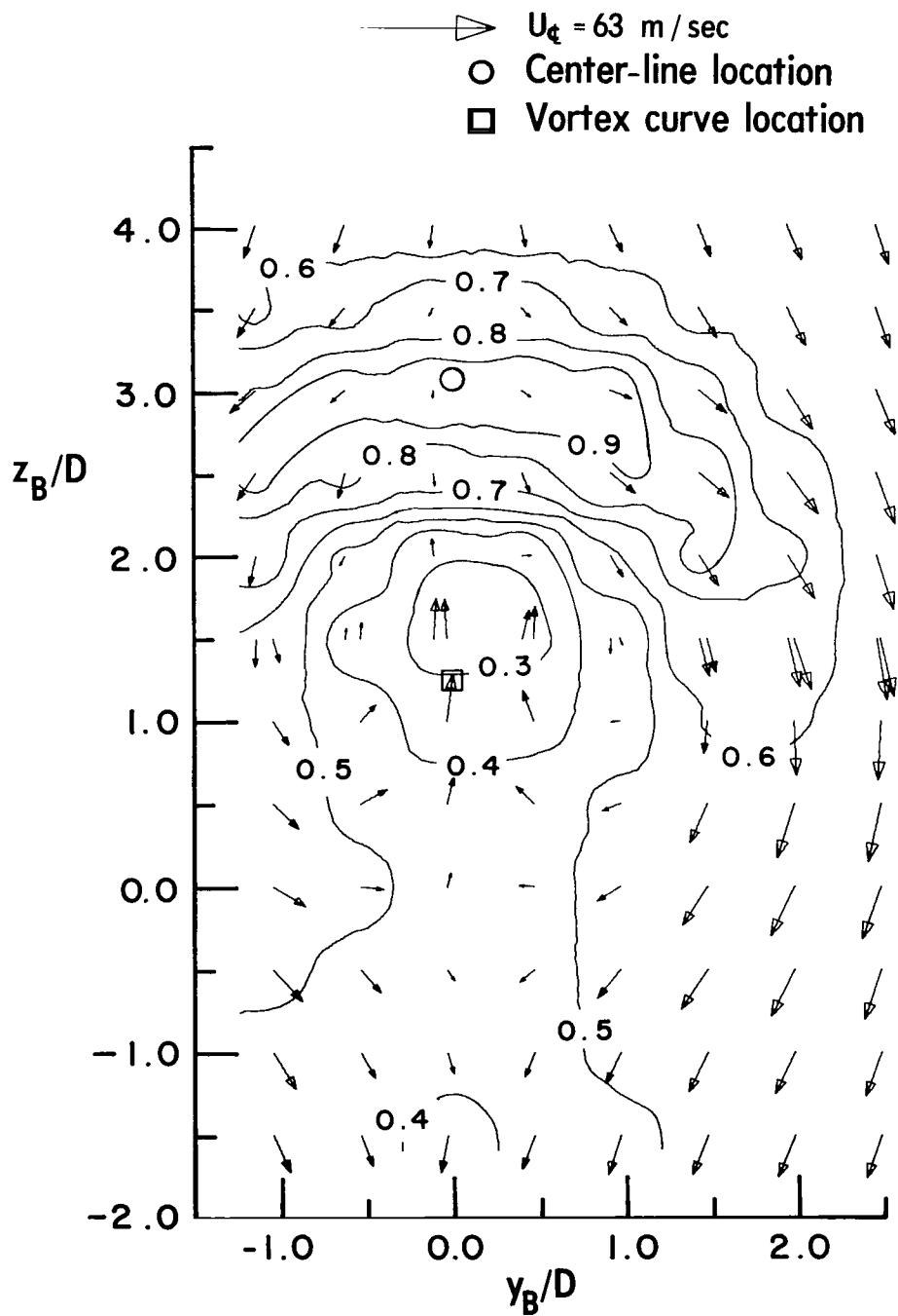
(b) Measured velocities, U_B/U_{\infty} and (\vec{V}_B + \vec{W}_B)/U_{\infty} .
