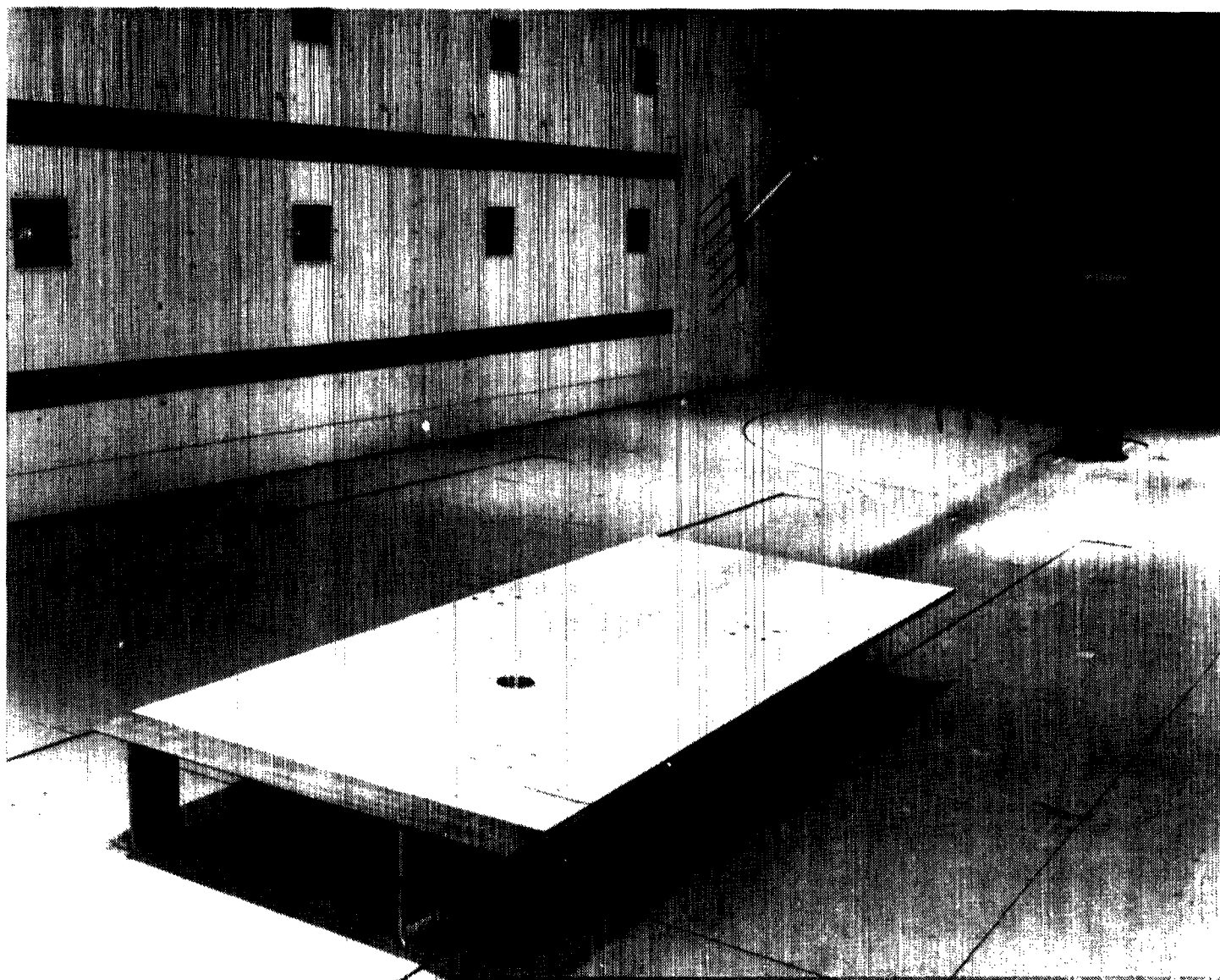
Figure 6.- Experimental arrangement in V/STOL tunnel for jet in a crossflow experiment.
