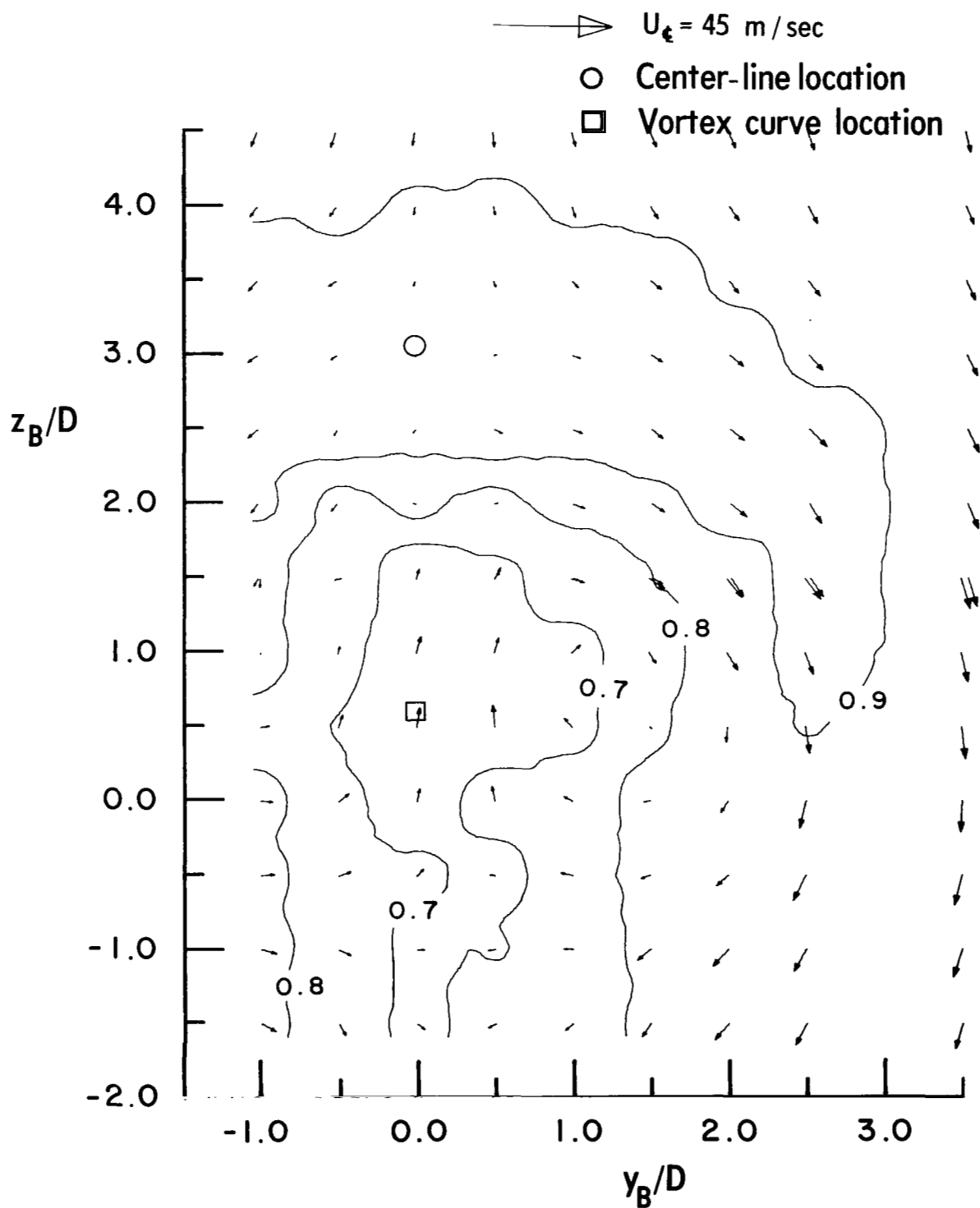
(b) Measured velocities, U_B/U_{\infty} and (\vec{v}_B + \vec{w}_B)/U_{\infty} .
