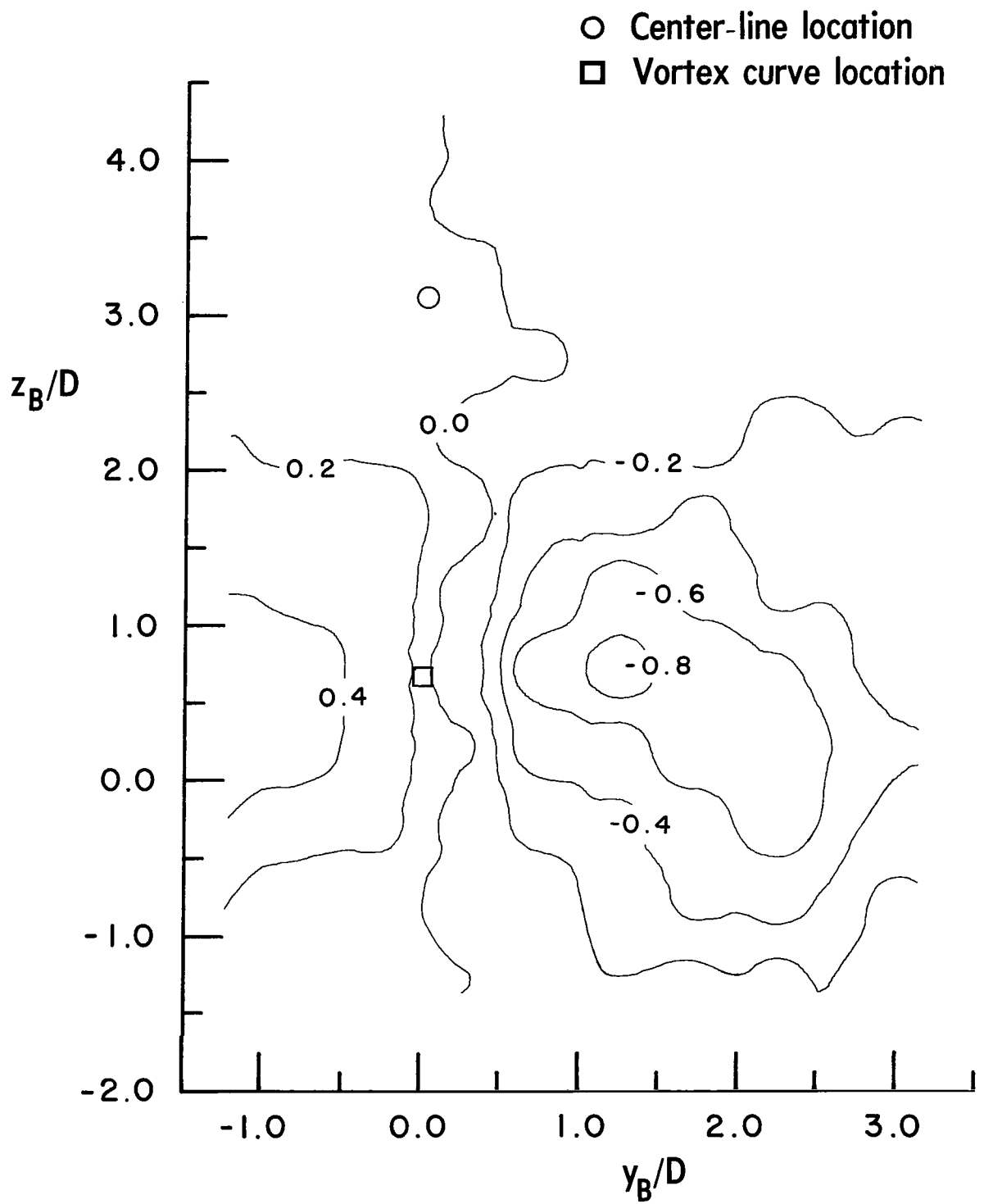
(c) Vorticity \omega/\omega_{\max} .
