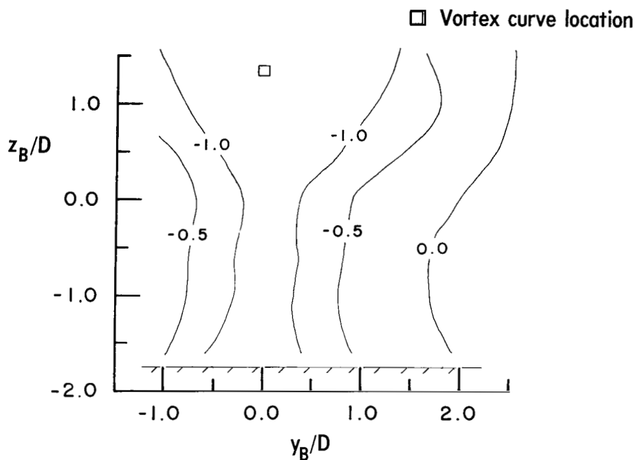
(a) Total-pressure coefficient C_{p,t} .
