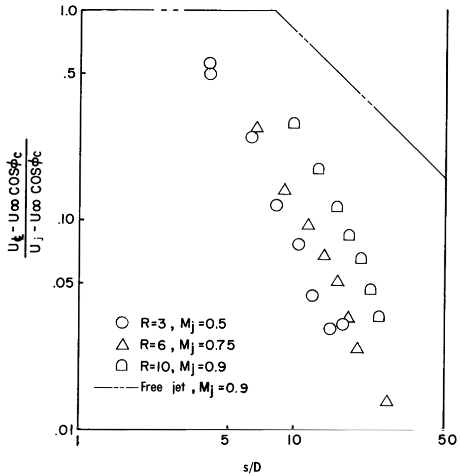
(b) Effect of velocity ratio.
