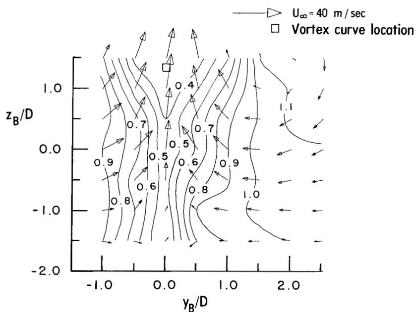
(b) Measured velocities, U_B/U_\infty and (\vec{v}_B + \vec{w}_B)/U_\infty .
