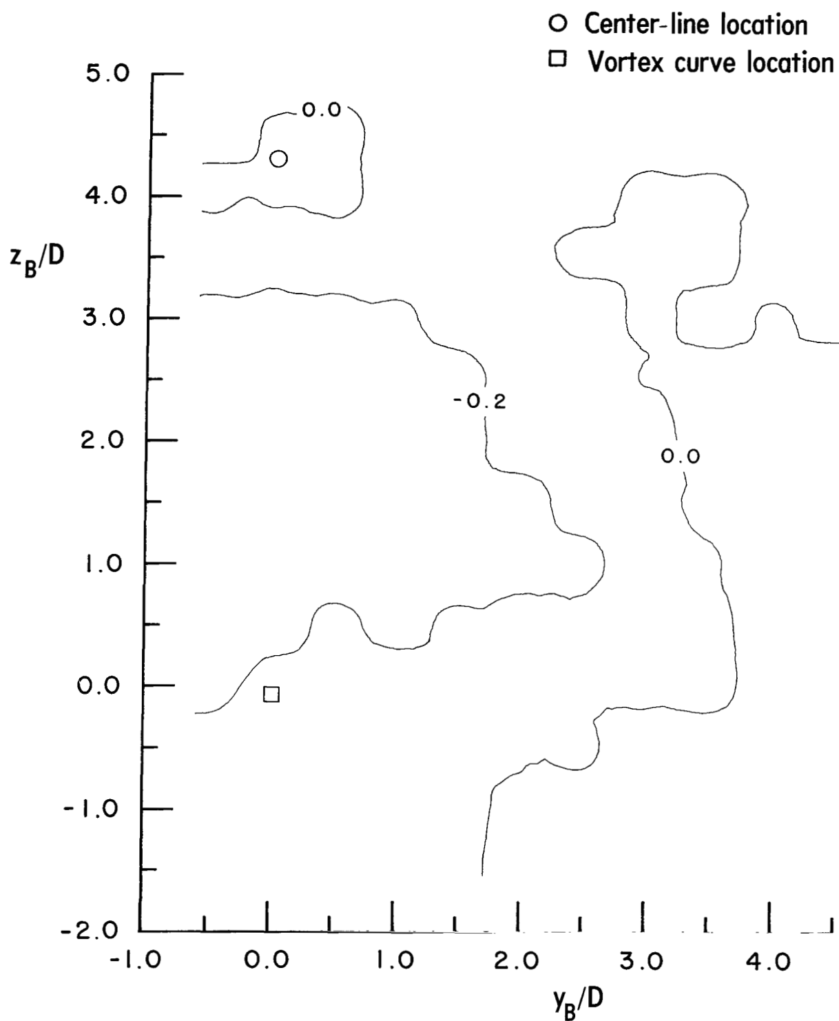
(a) Total-pressure coefficient C_{p,t} .
