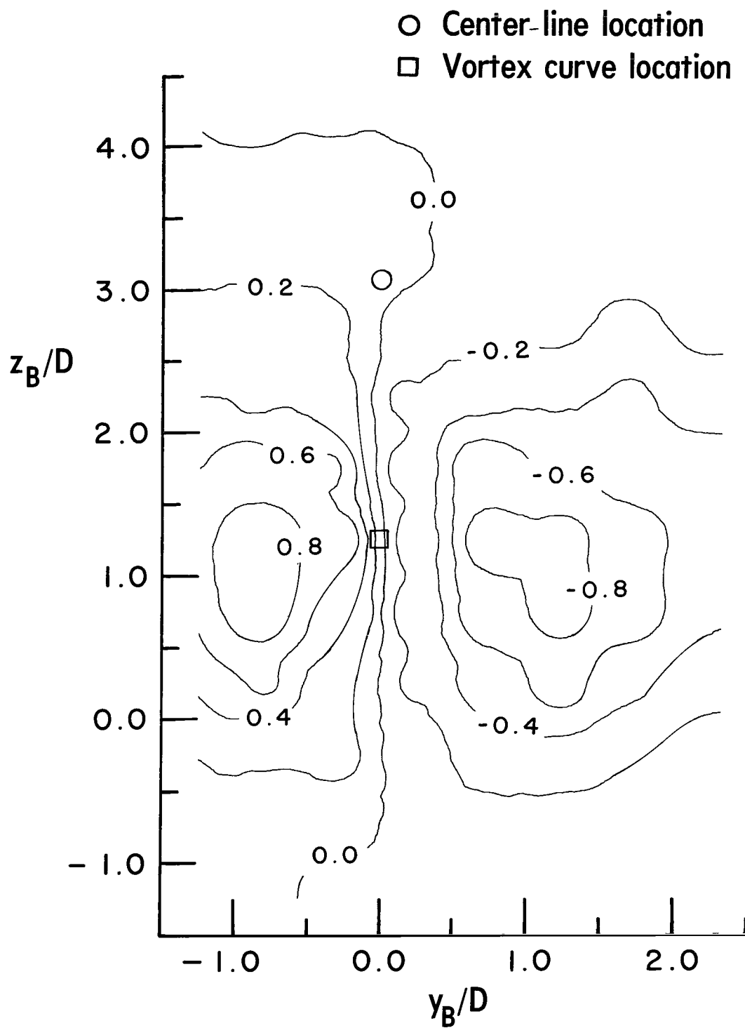
(c) Vorticity \omega/\omega_{\max} .
