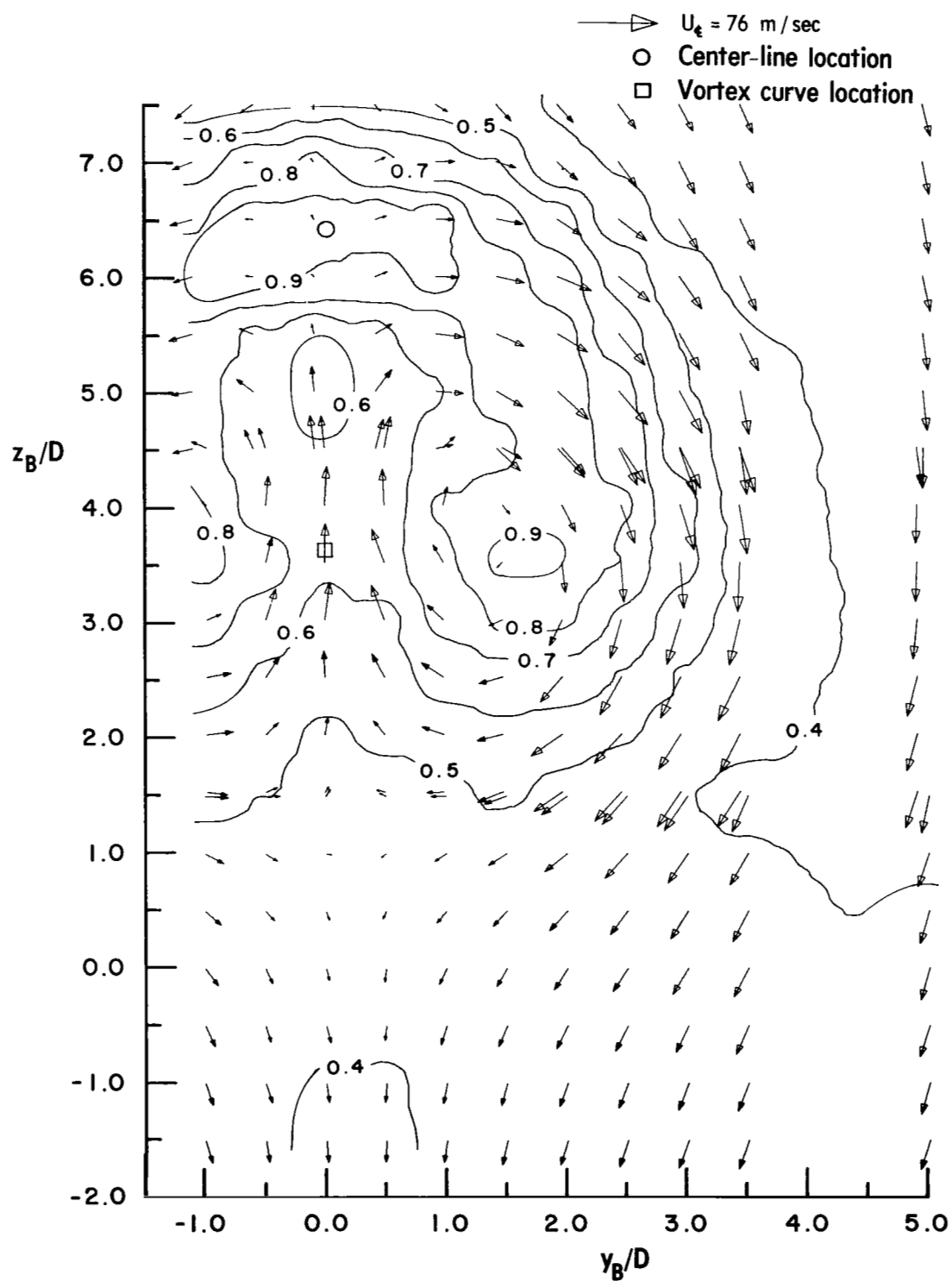
(b) Measured velocities, U_B/U_t and (\vec{V}_B + \vec{W}_B)/U_t .
