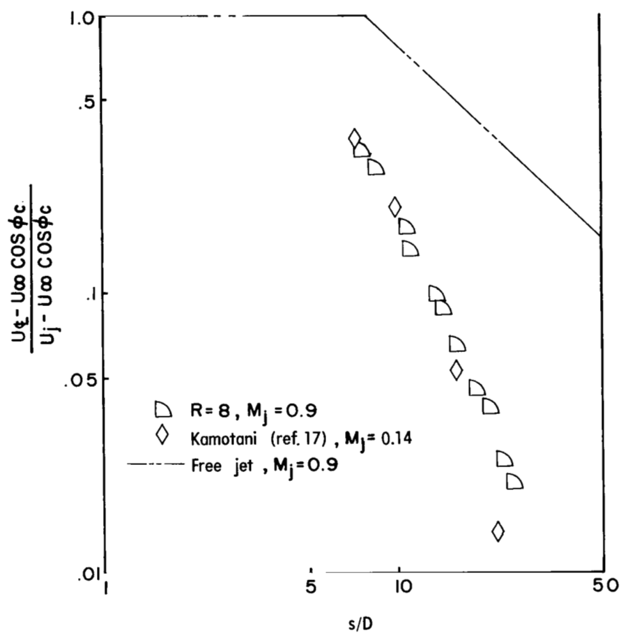
Figure 9.- Decay of jet center-line speed.
