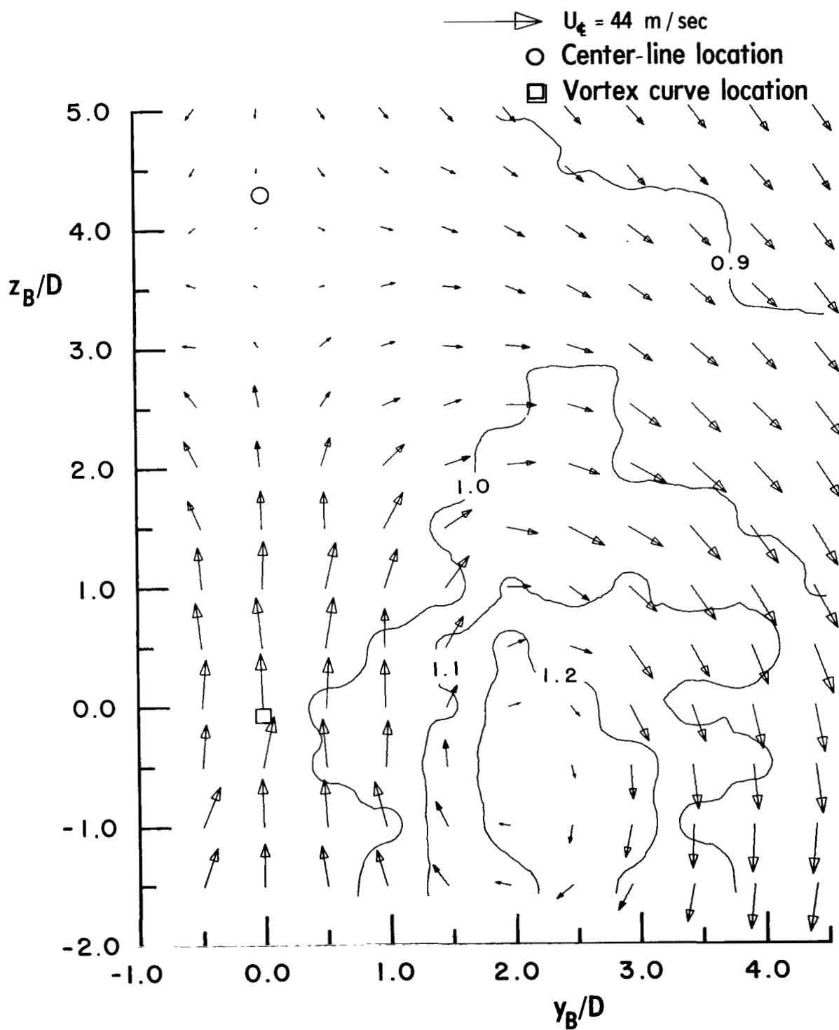
(b) Measured velocities, U_B/U_\phi and (\vec{v}_B + \vec{w}_B)/U_\phi .
