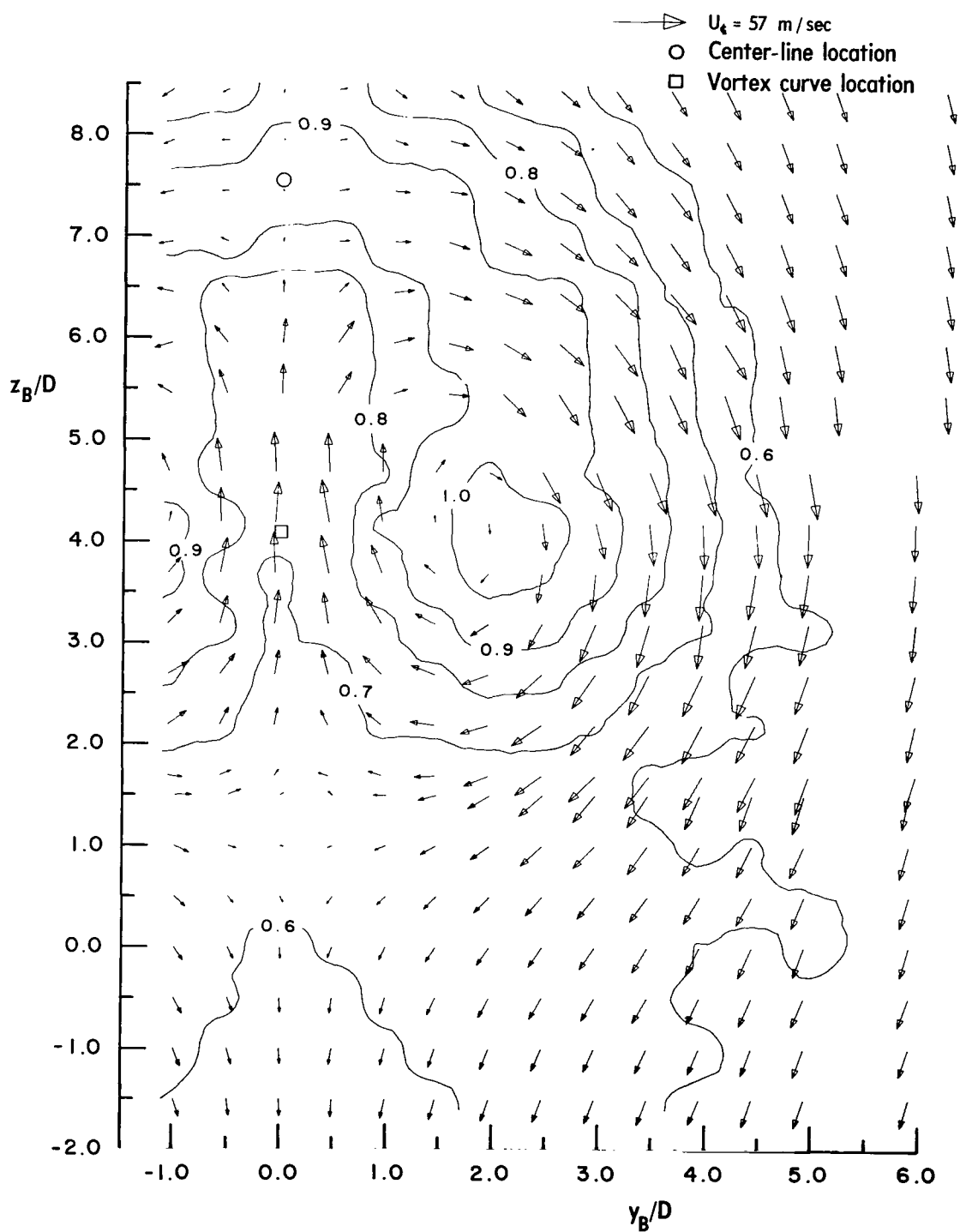
(b) Measured velocities, U_B/U_\infty and (\vec{V}_B + \vec{W}_B)/U_\infty .
