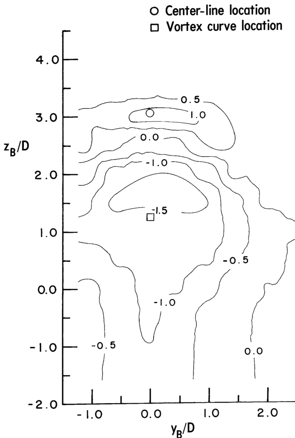
(a) Total-pressure coefficient C_{p,t} .
