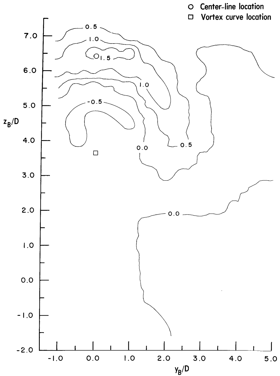
(a) Total-pressure coefficient C_{p,t} .
