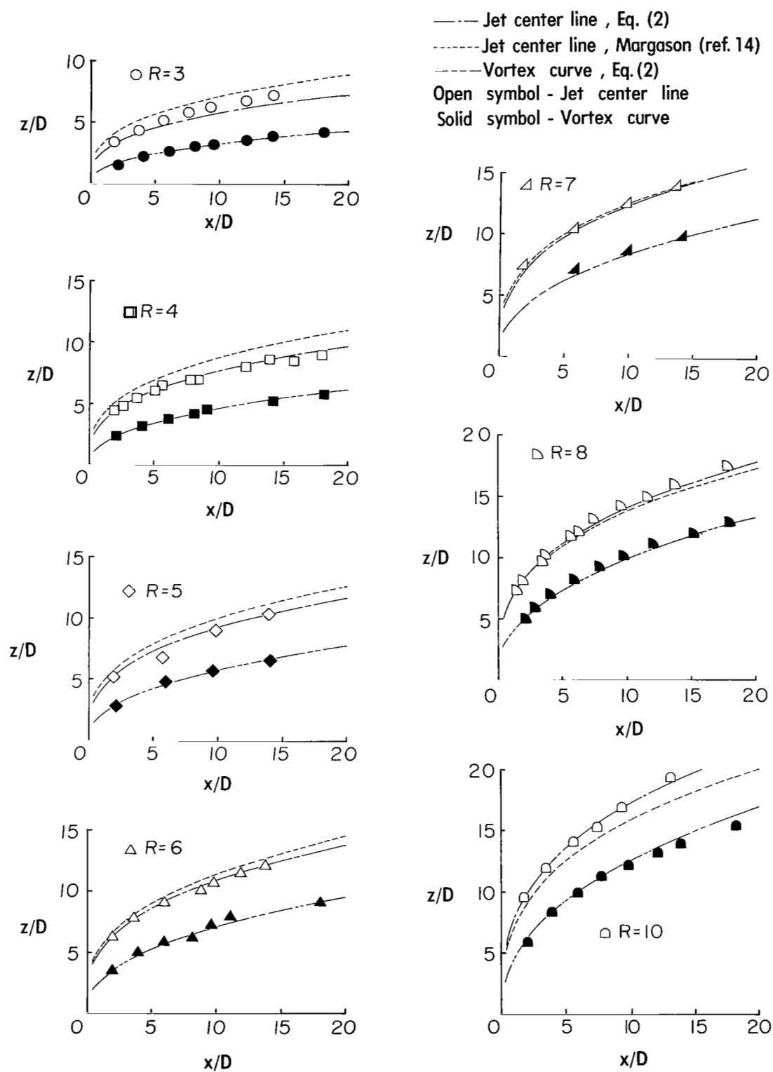
Figure 10.- Jet center lines and vortex curves.
