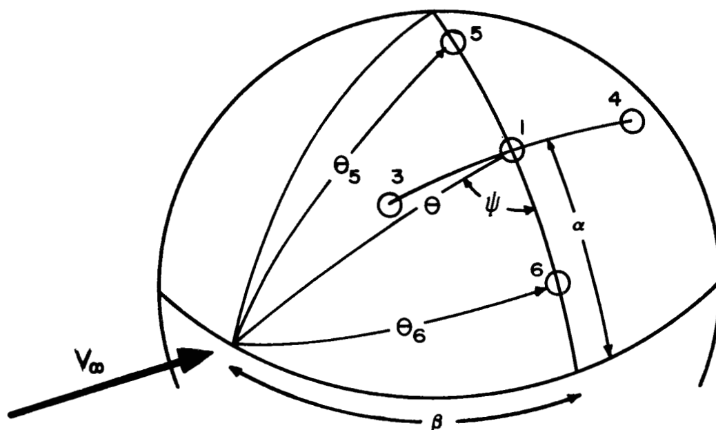
Figure A1.- Probe coordinate system.
