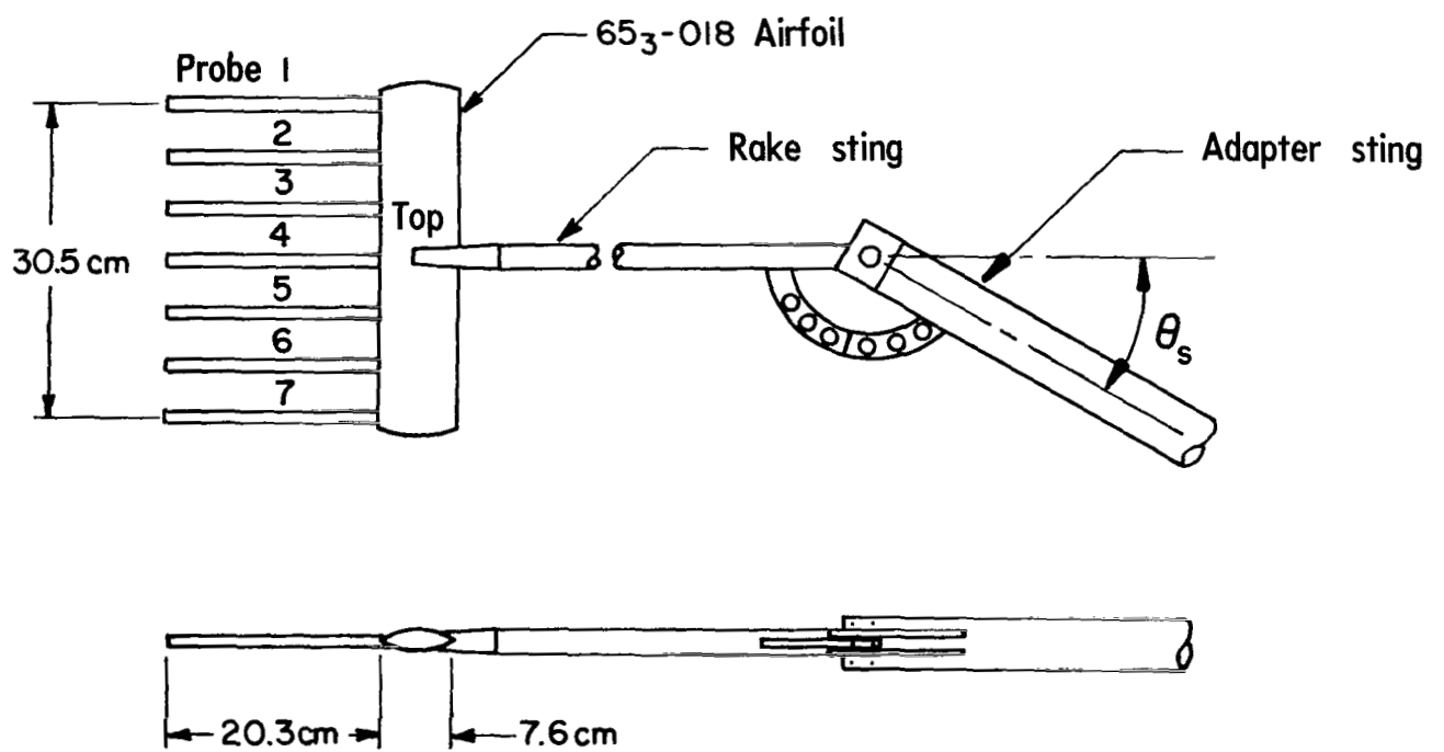
Figure 4.- Rake of yaw-pitch probes.
