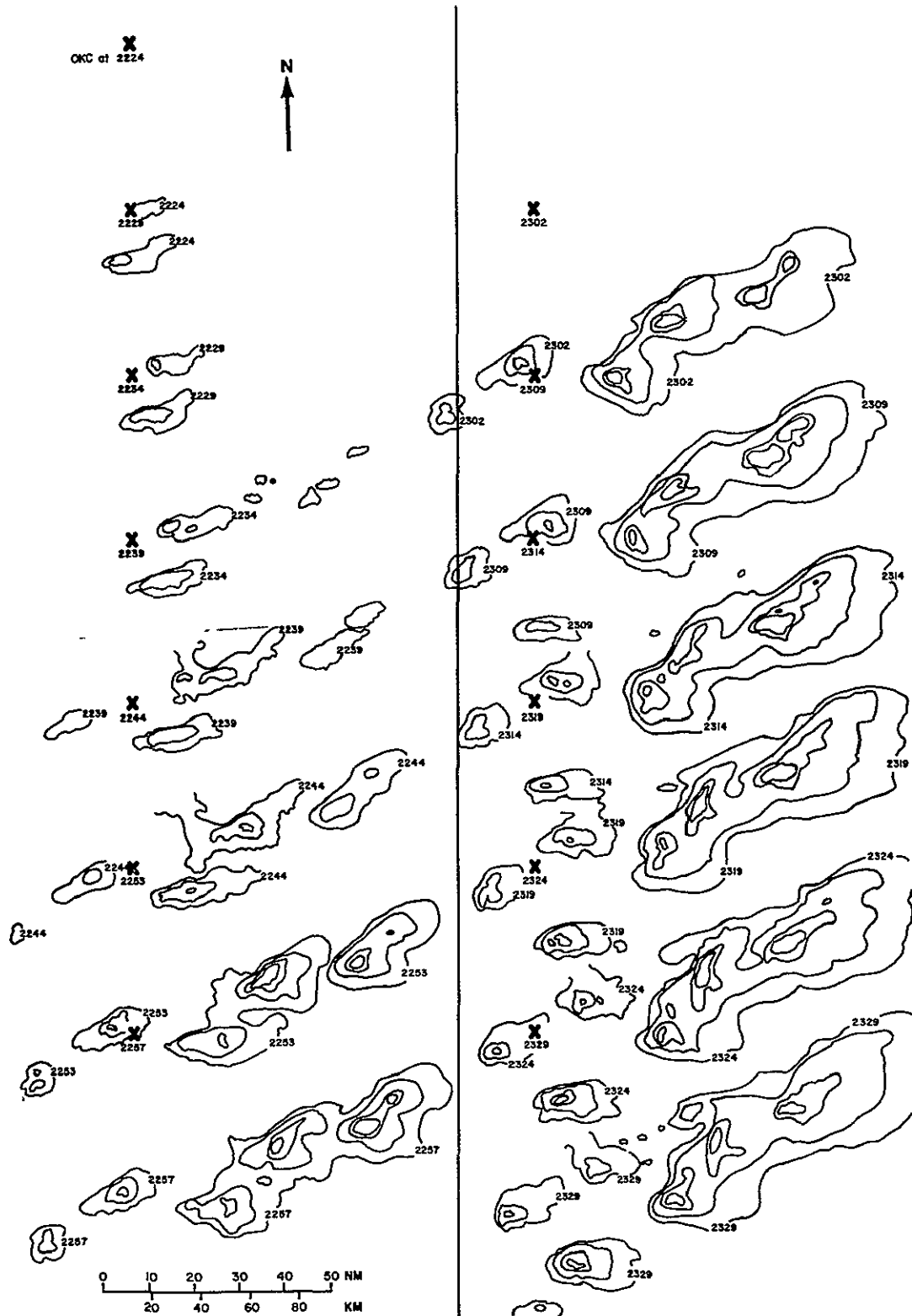
Figure 5-1 Intensity contoured radar reflectivities for the Wewoka storm.
