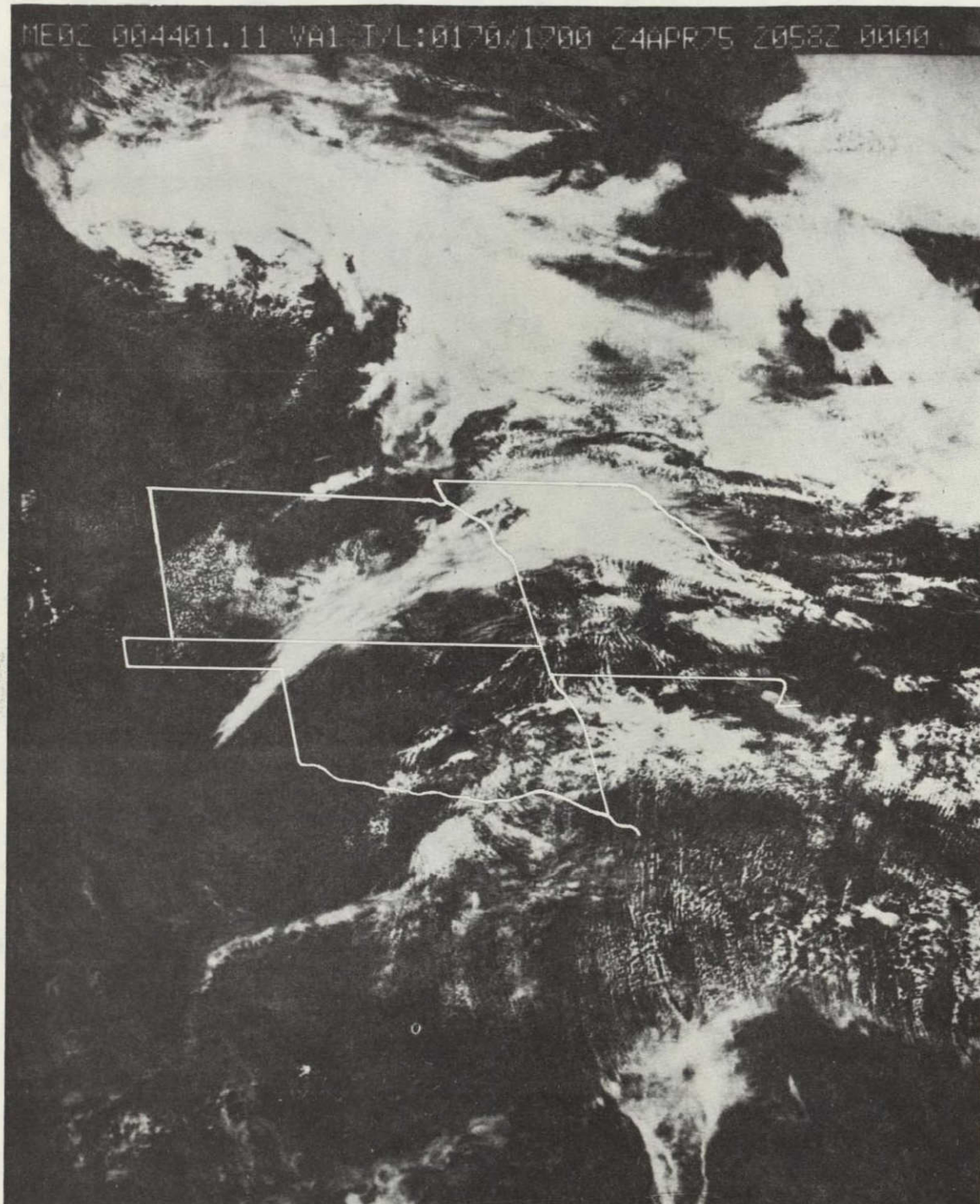
Figure 3-1 SMS-2 visible channel image at 2058 GMT.
