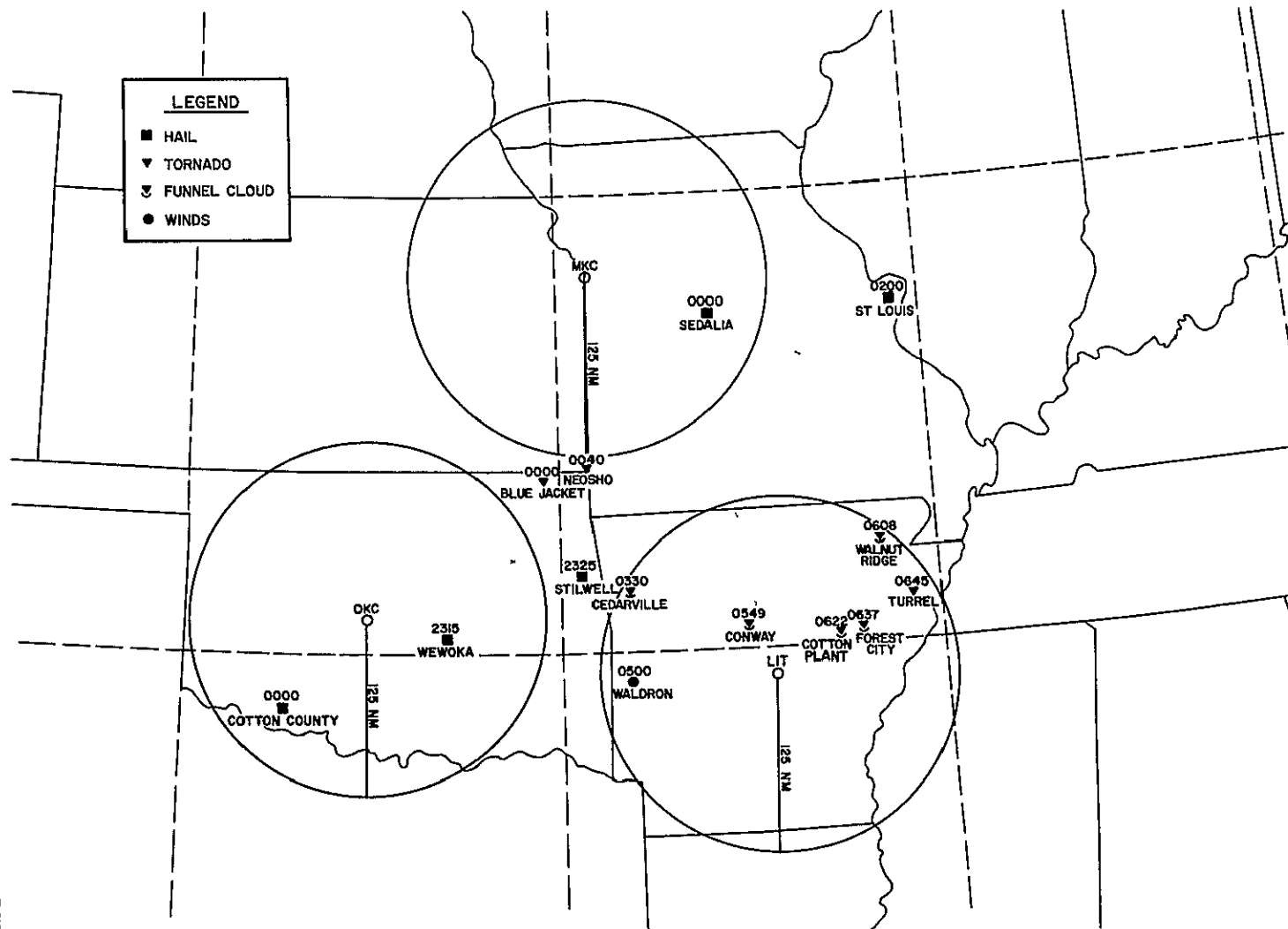
Figure 2-7 Severe storm reports 24-25 April 1975.
