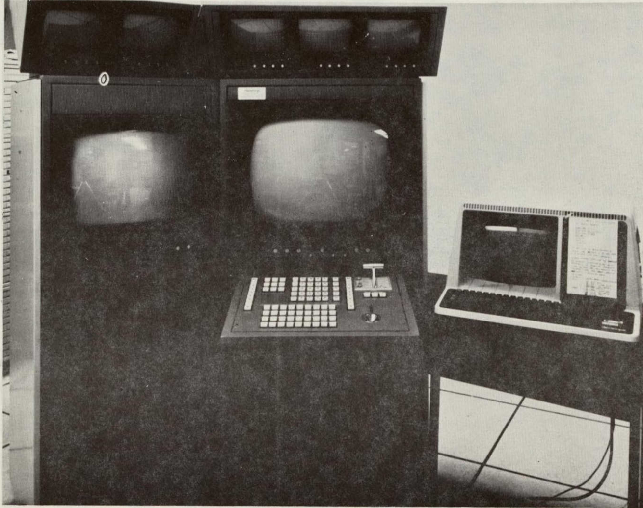
Figure 3-2 A portion of the AOIPS used for cloud tracking.
