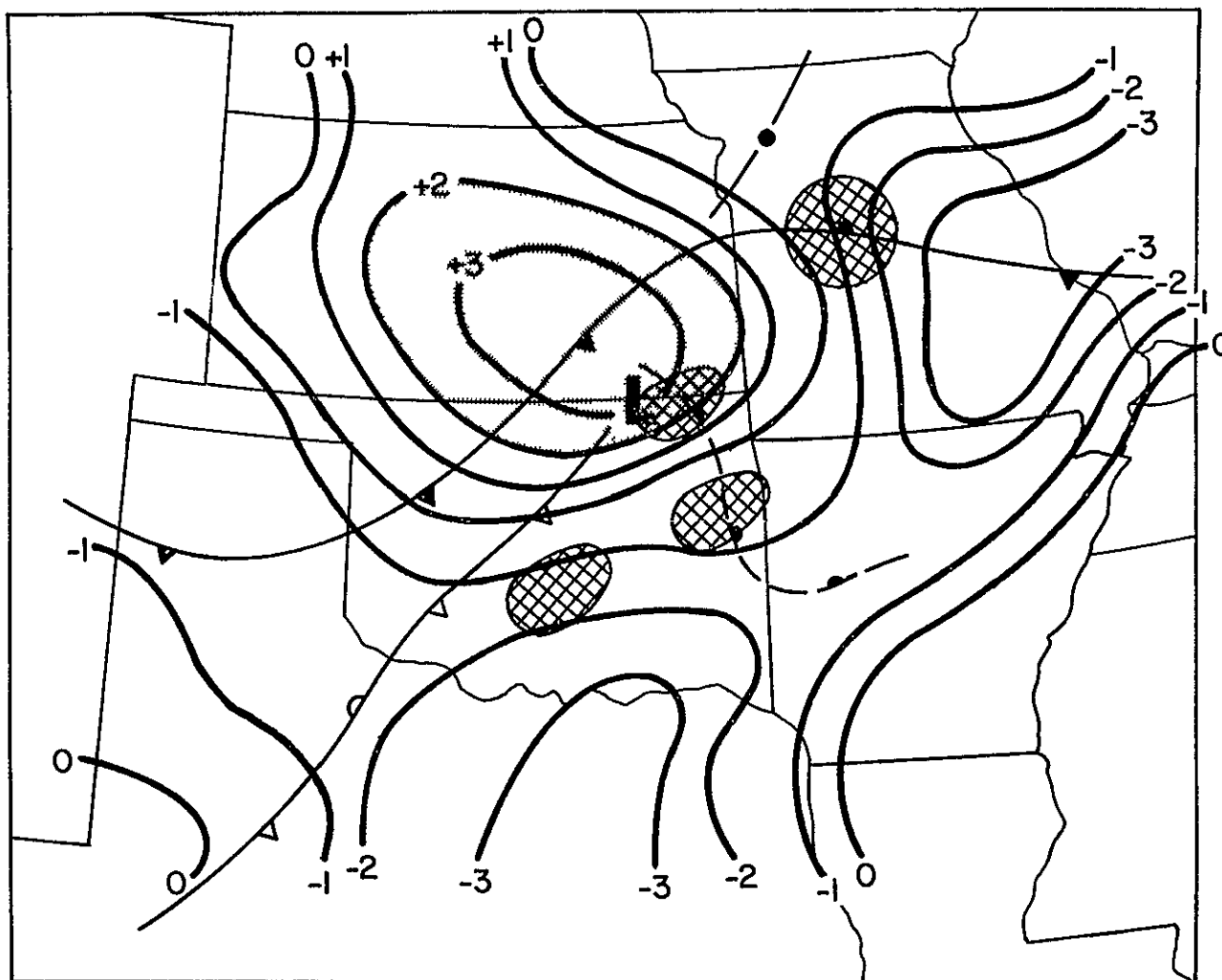
Figure 2-6 700 millibar vertical velocity in \mu\text{bars s}^{-1} (from Wilson, 1976). Regions where severe thunderstorms developed are cross-hatched.
