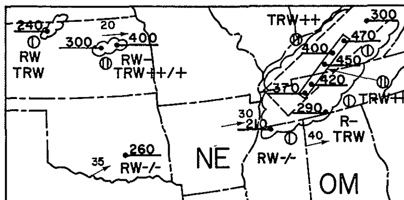
Figure 3-10 NWS radar summary at 1835 GMT.
