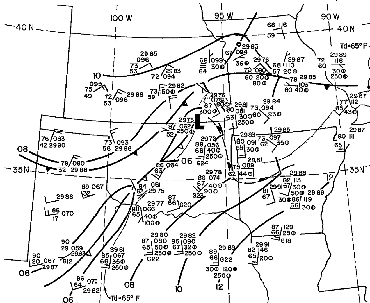
Figure 2-2 Surface analysis 24 April 1975 2100 GMT.
