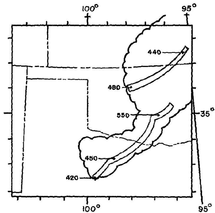
b) NWS radar summary 19 April 1972 1945 CST.
