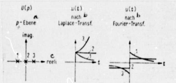
Fig. 1. Pole position of a single pole in the complex frequency plane, and corresponding time function according to Laplace and Fourier transformations.
