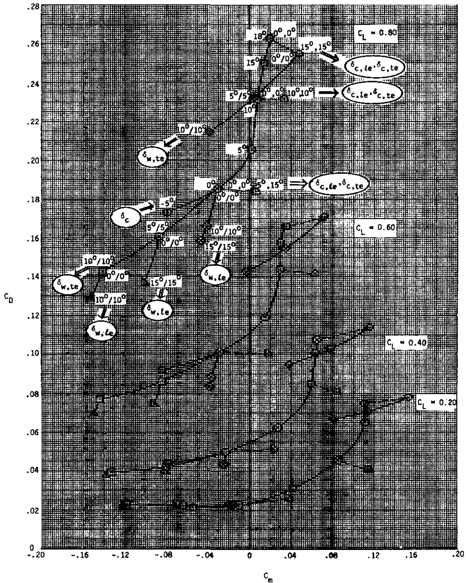
Figure 20.- Variation of drag coefficient with pitching-moment coefficient for all control variables (canard on) for constant values of lift coefficient at M = 0.40 . (This figure is generated from crossplots of basic data; symbols indicate geometric control settings, not actual data points.)
