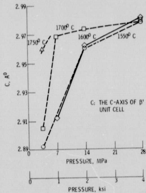
Figure 10. - Pressure and temperature effects on lattice parameter of \beta phase.
