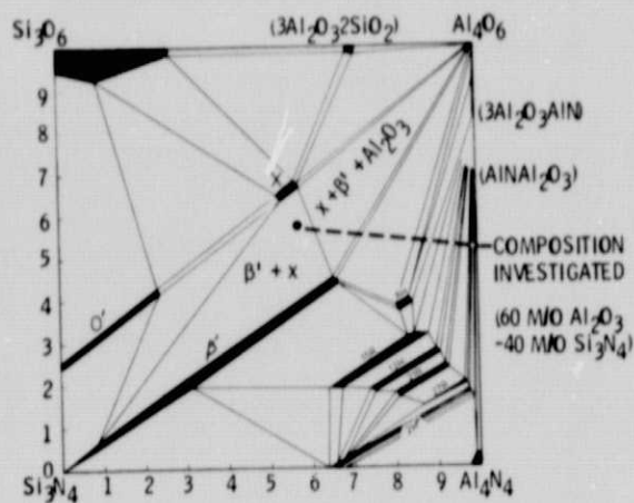
Figure 9. - The \text{Si}_3\text{N}_4 - \text{AlN} - \text{Al}_2\text{O}_3 - \text{SiO}_2 system (from ref. 9).
