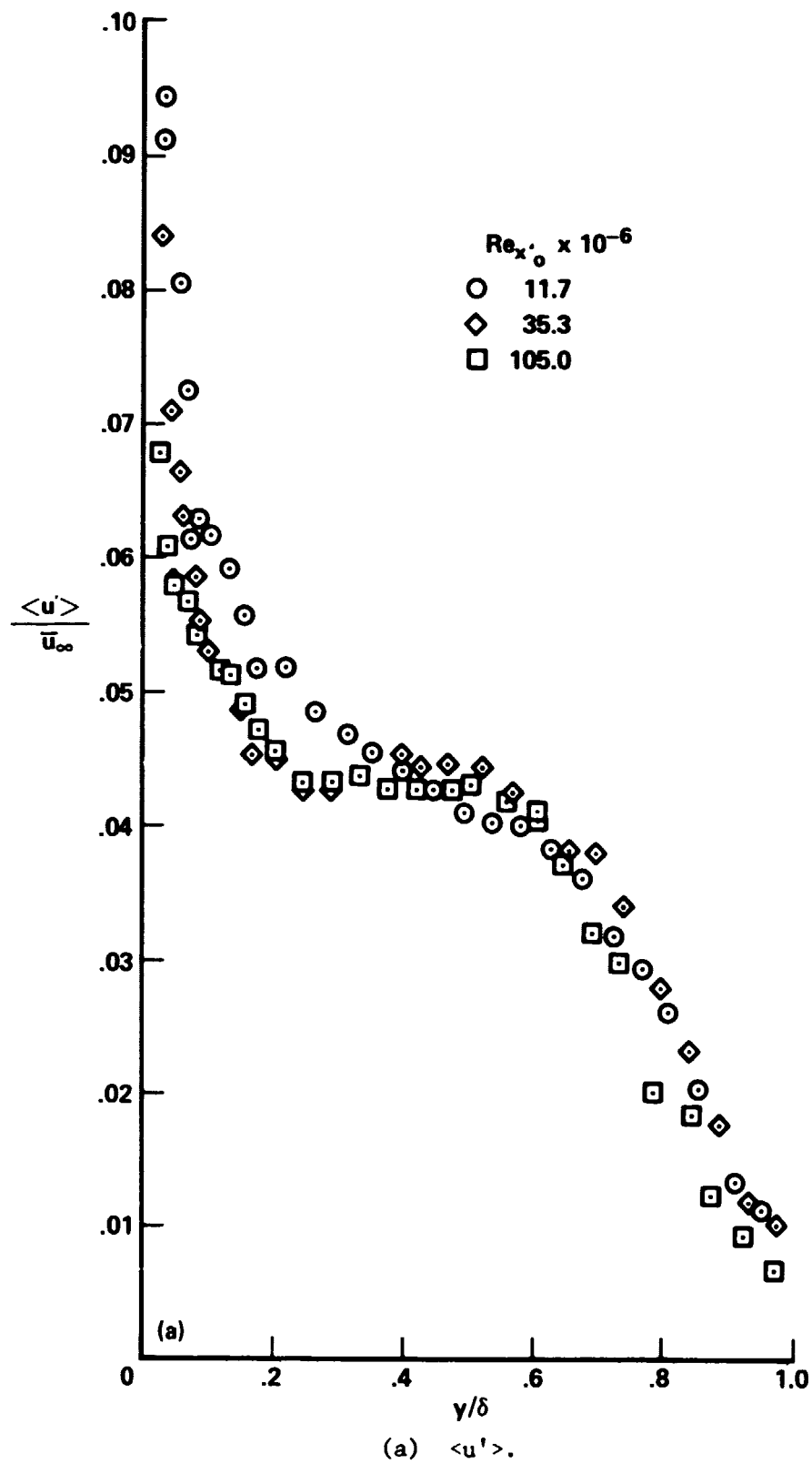
Figure 16.- Velocity fluctuation distributions across the upstream boundary layer at three Reynolds numbers.
