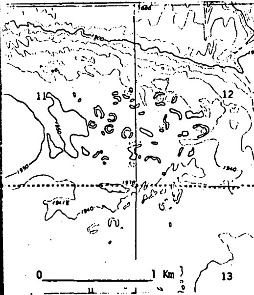
the prominent rings described for the Odessa area by McKee and Stradling (1970) and by Hodges (1976).
