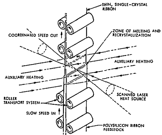
d) Laser Zone Crystallization
