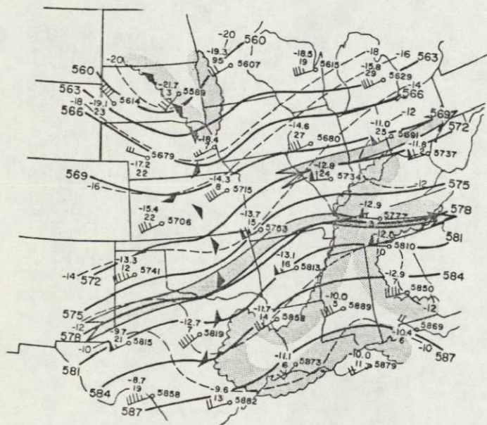
Fig. 2. 1500 CST 500 mb analysis. Triangles show locations of short-wave troughs. Arrows depict axes of maximum wind speeds, full barb = 10 kt, flag = 50 kt. Moist regions with T-T_d \leq 6^\circ\text{C} are shaded.
