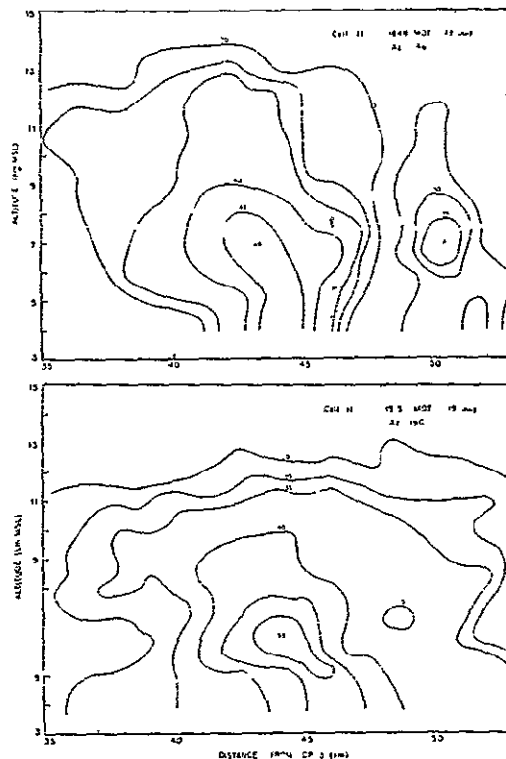
Figure 7. Reconstructed PPI cross sections of C11 from the 1848 MDT (7a) and 1916 MDT (7b) sector scans. The reflectivity factor contours are drawn for 20, 30, 35, 40, 45, and 50 dBZ. The corresponding PPI's appear in Fig. 6. It should be noted that a 4-min. time period was taken to obtain this reflectivity data.
