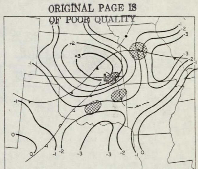
Fig. 4. 1500 CST 700 mb vertical velocity in \mu\text{bars s}^{-1} (from Wilson, 1976). Regions where severe thunderstorms developed during the following 2 h are cross-hatched.
