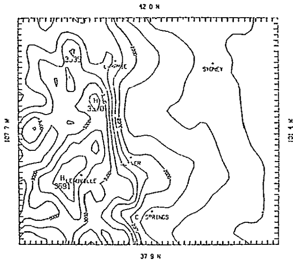
Fig. 4. Smoothed topography (2 and 4Δx trends removed for a 11 km grid) used as input in the Pielke mesoscale model. (contour interval 250 m) function of differences in thermal inertia of the soil types. The importance of such a temperature difference is even more striking when one realizes that the plateau represents a large-area elevated heat source some 2600 to 4000 feet above the surrounding plains. Thus, it would appear to be a major driving force in the mountain upslope flow.
