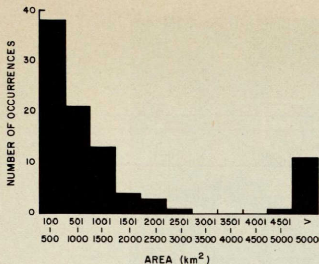
FIG. 2. Cloud size distribution histograms for Miles City, Mont., area as observed from the ATS-3 satellite. The satellite resolution is 113 \text{ km}^2 .
