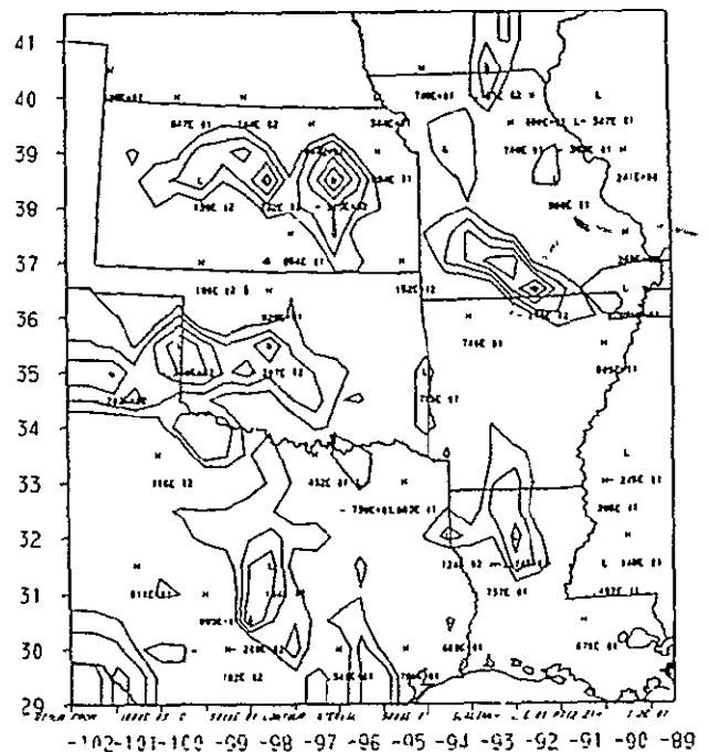
Fig 9. The moisture divergence field. Units are 10^{-5} cm H_2O s^{-1} . Only negative values (moisture convergence) have been contoured.
