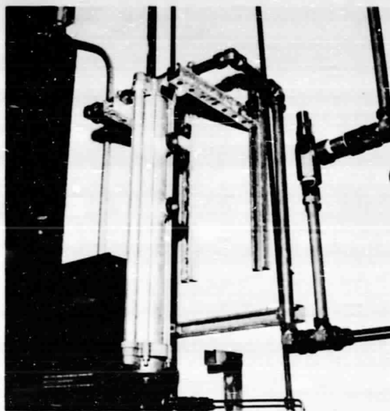
Figure 25.- Water Immersion Facility breathing air carbon monoxide filter.
