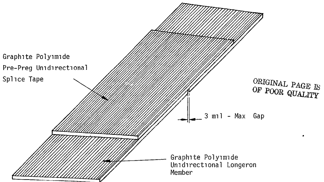
TYPICAL LONGERON JOINT
