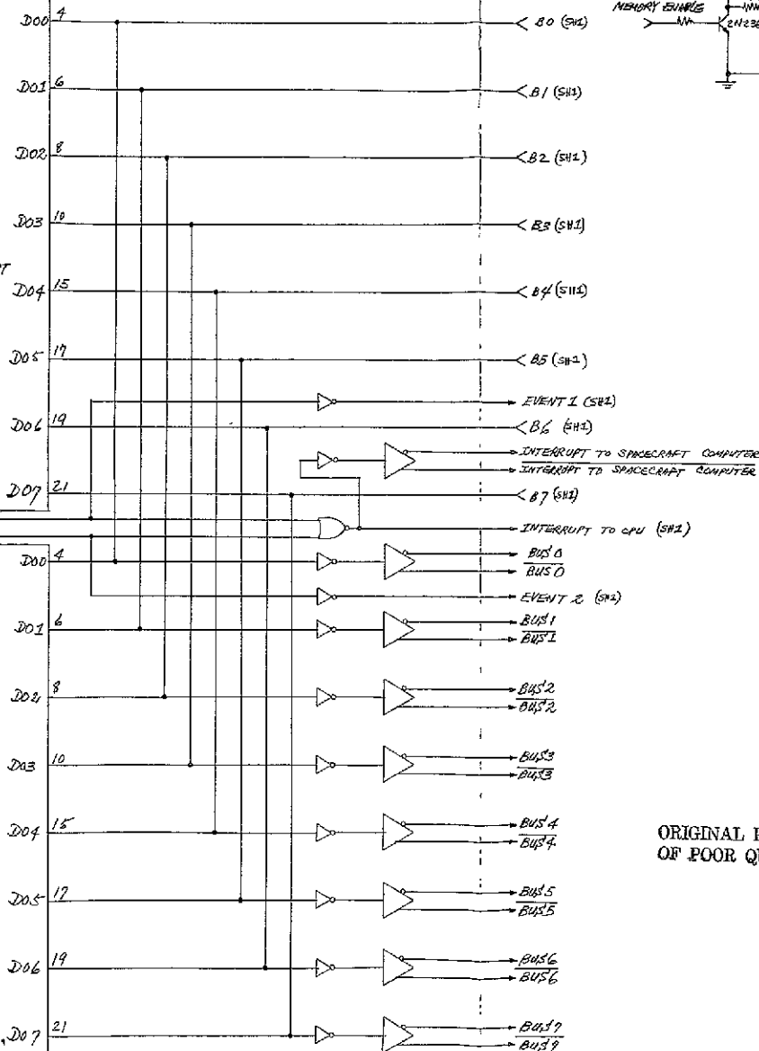
Figure 3-29 Digital Interface Unit
