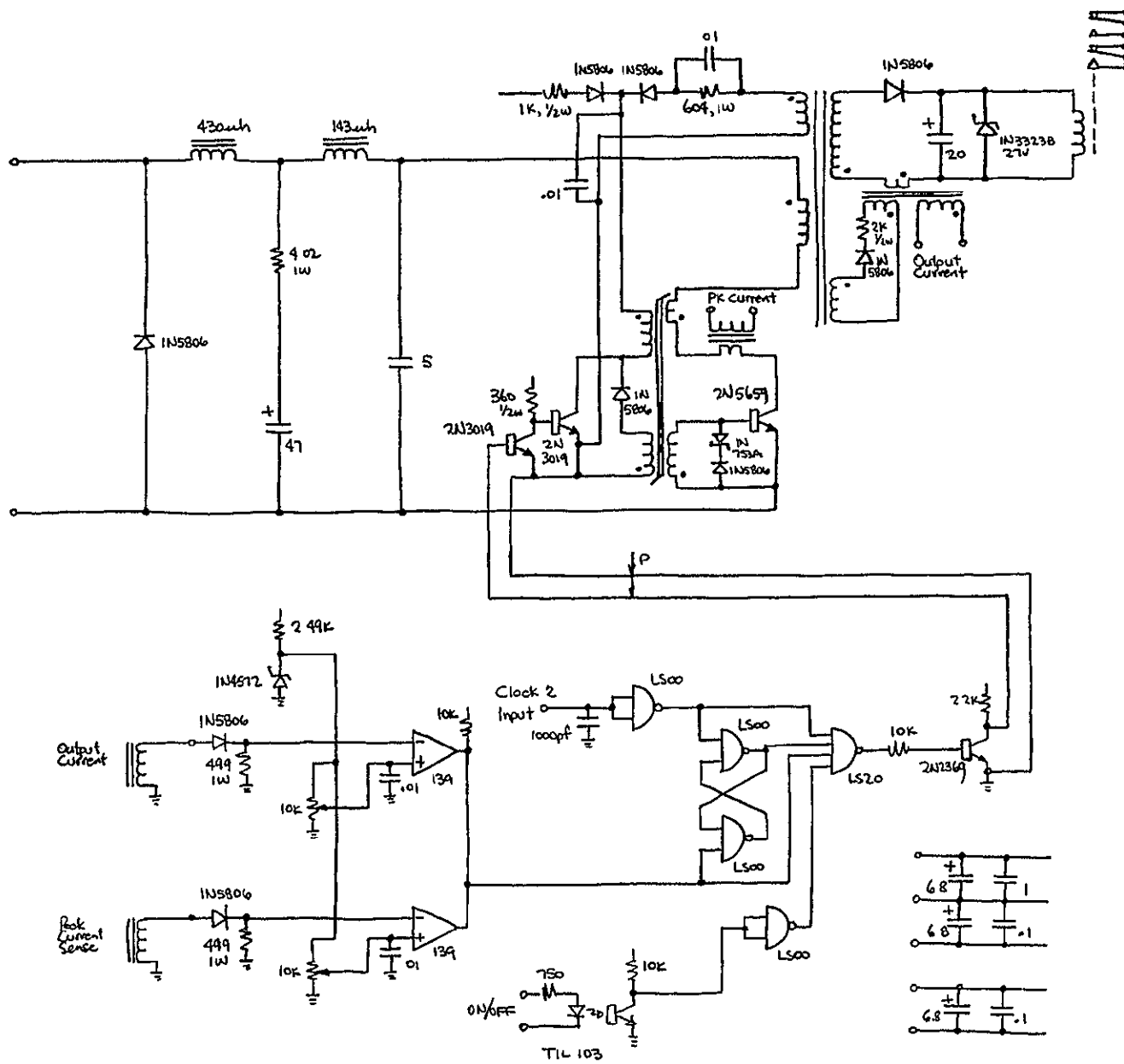
Figure 3-23 Relay Driver
