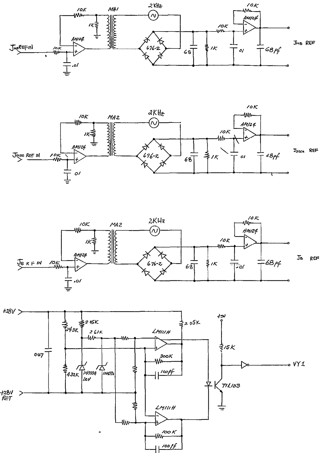
Figure 3-35 Command and Protection
