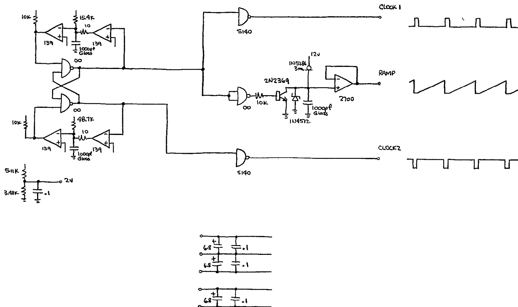
Figure 3-18 Multiple Buck Boost Converter Master Oscillator & Ramp Generator
