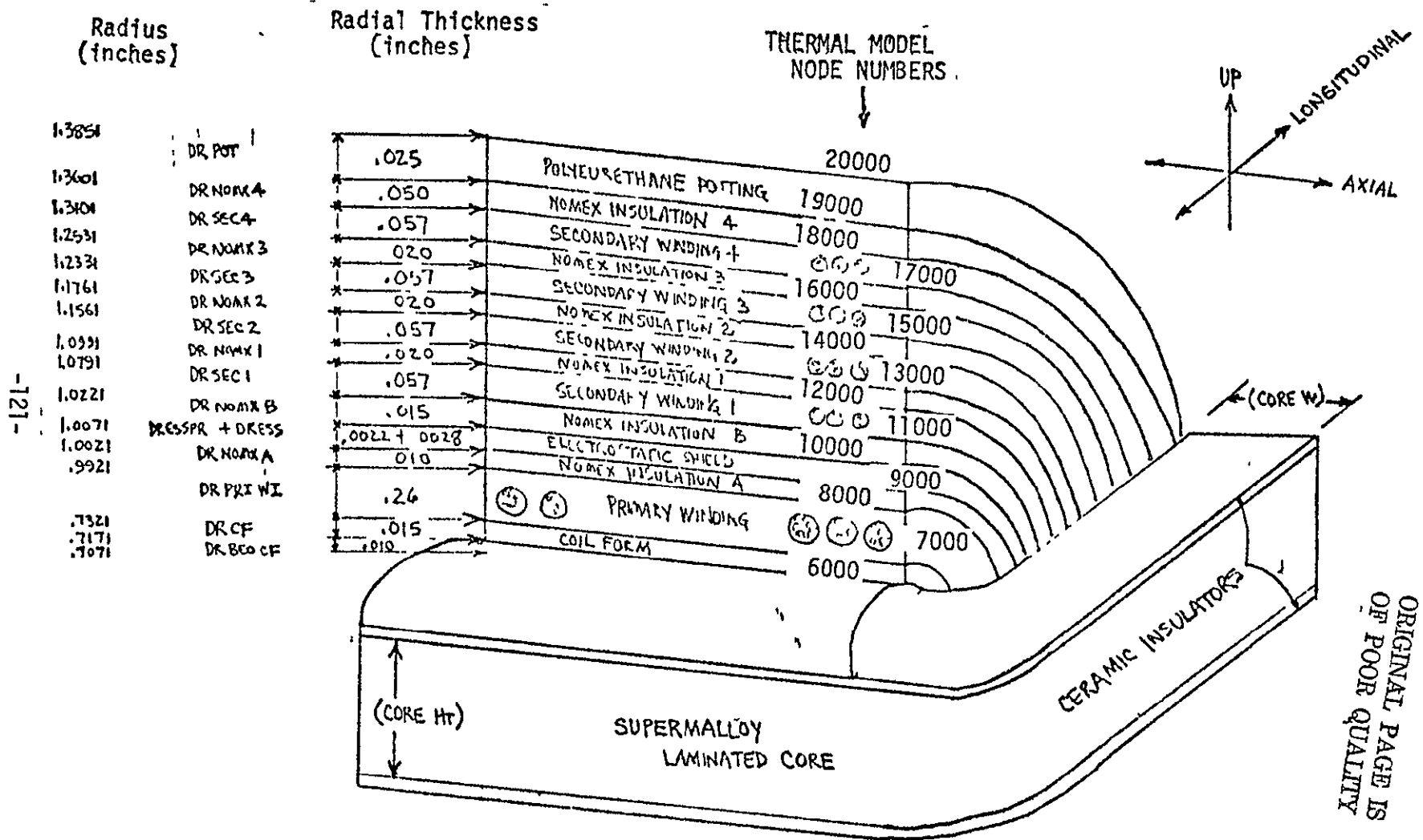
FIGURE 3-46.THERMAL MODEL - TRANSFORMER COIL
