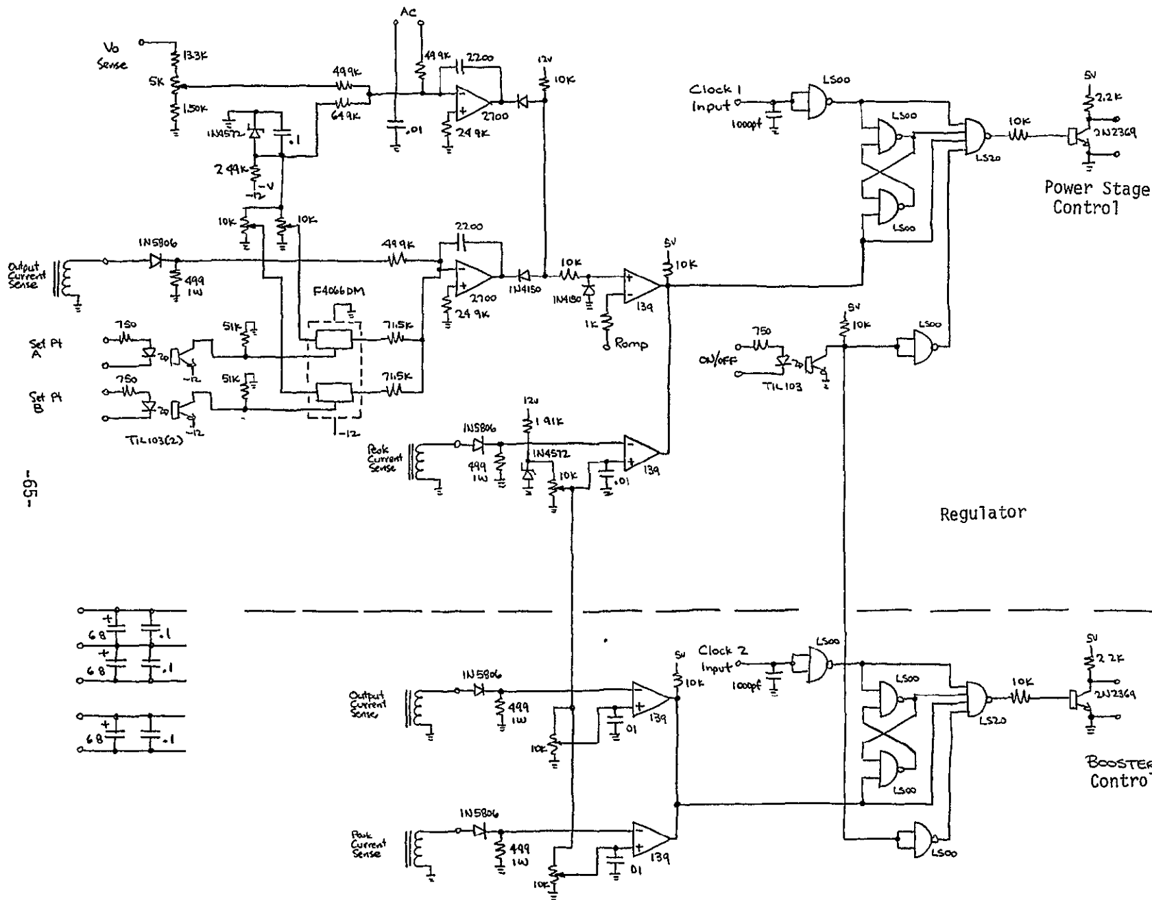
Figure 3-22 V7 Regulator
