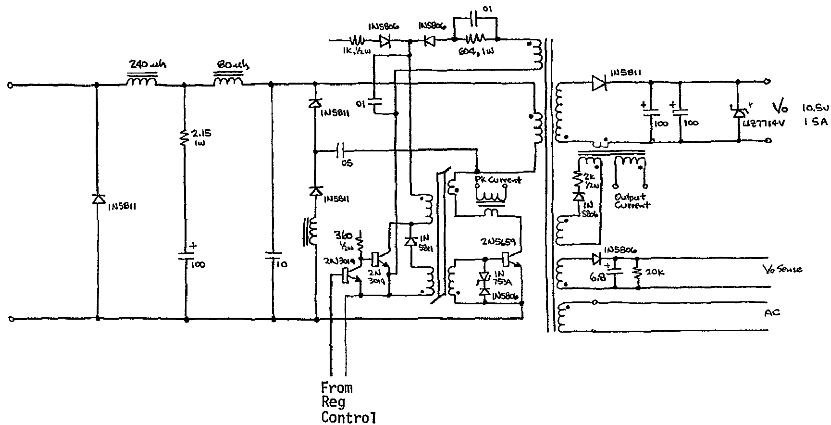
Figure 3-19 V1 Output
