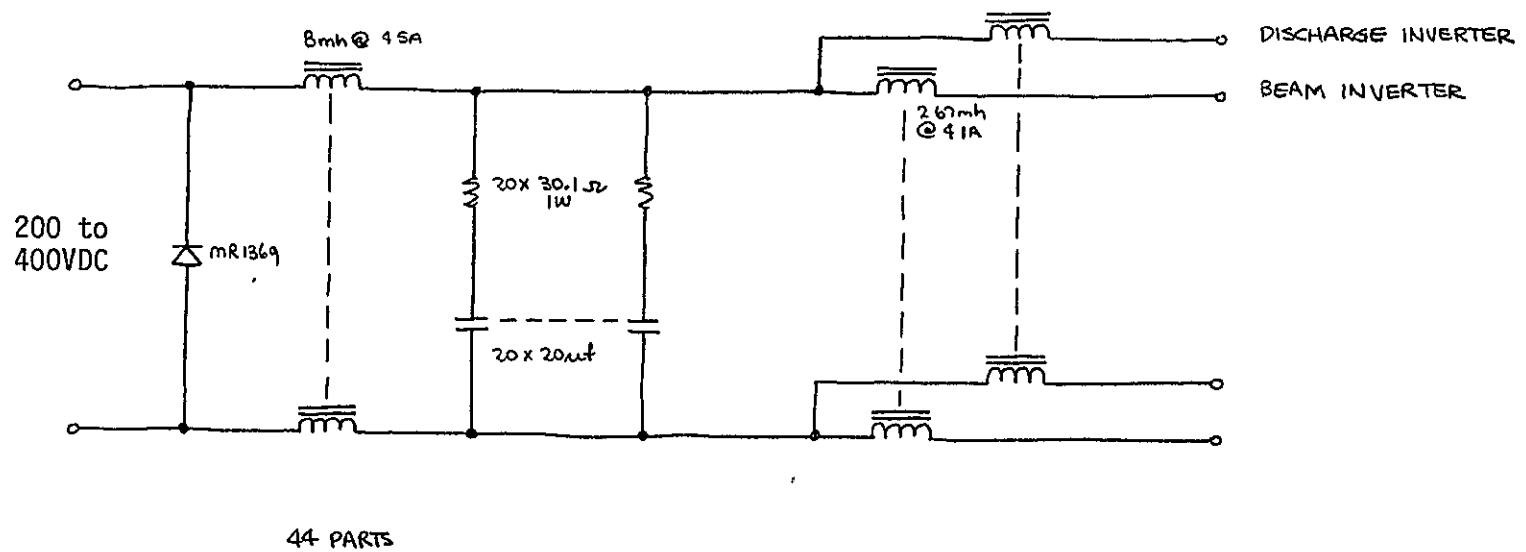
FIGURE 3-8 Input Filter
