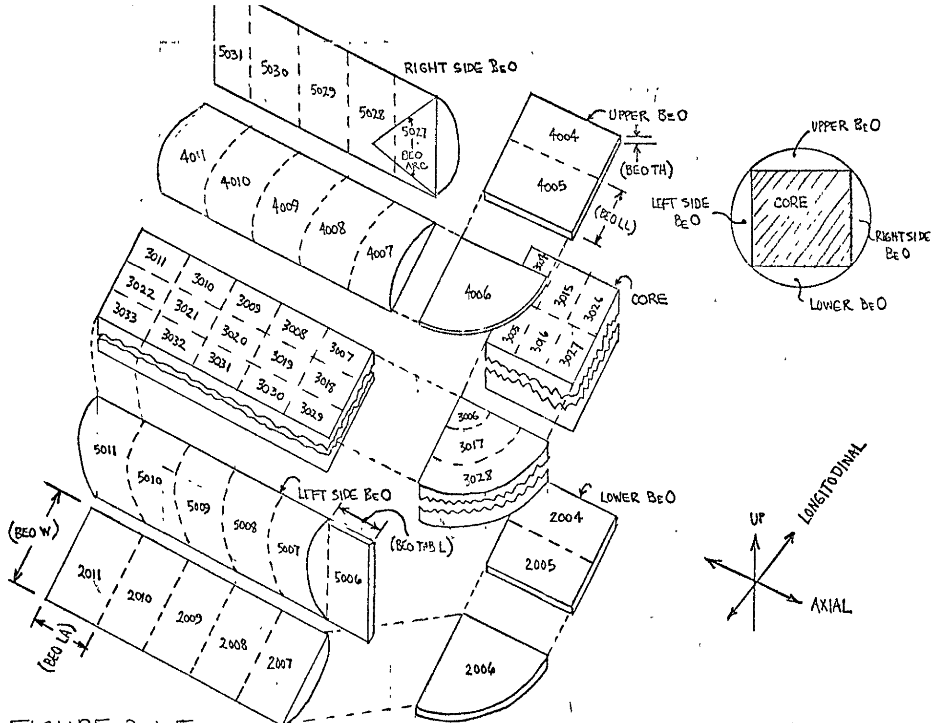
FIGURE 3-45. THERMAL MODEL - CORE AND CERAMIC INSULATORS
