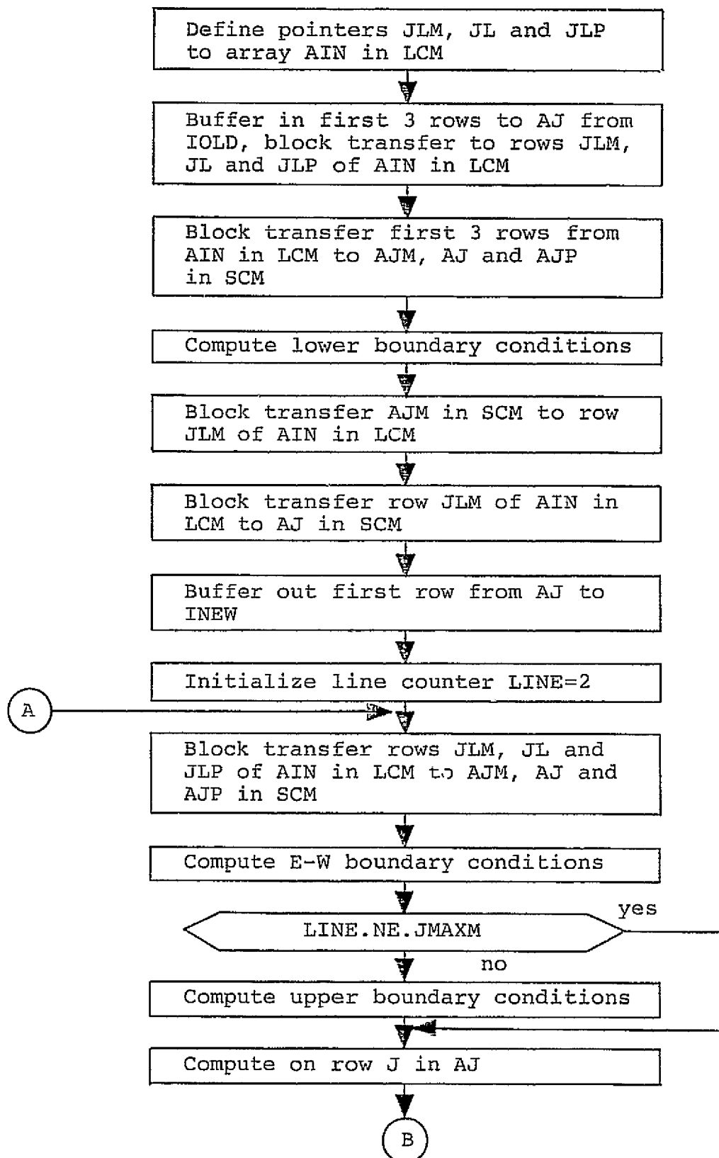
FIGURE III-7: DATA FLOW FOR ONE SWEEP OF THE DATA FILE - MODEL PEFHFV
