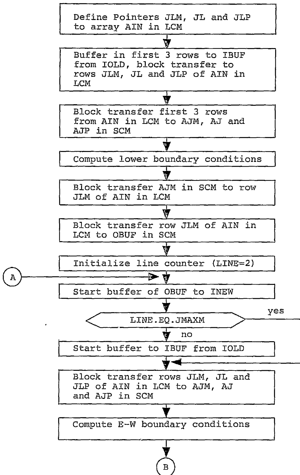
FIGURE III-6: DATA FLOW FOR ONE SWEEP OF THE DATA FILE - MODEL PEFHCV
