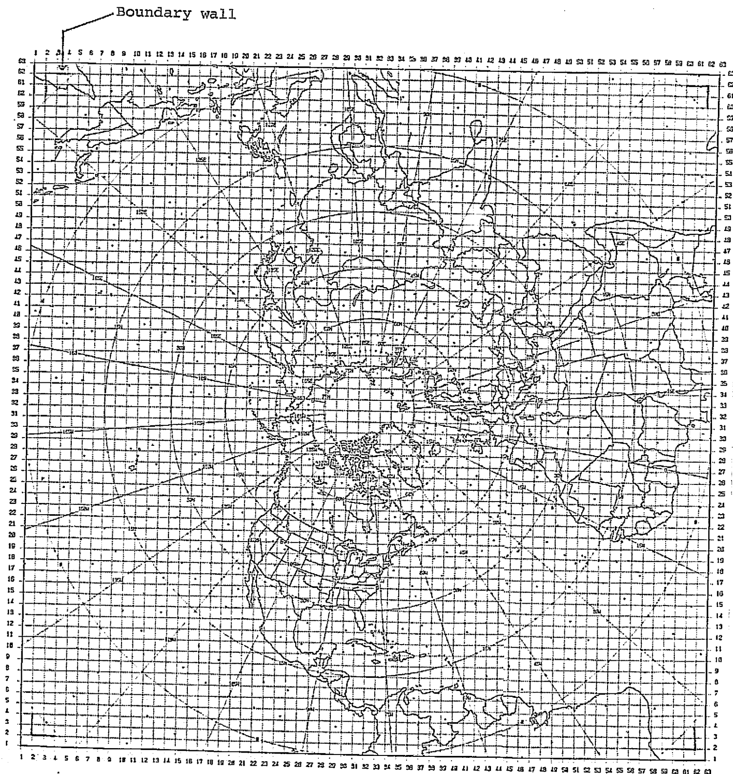
FIGURE II-2: NORTHERN HEMISPHERE POLAR STEREOGRAPHIC GRID (63 x 63).
