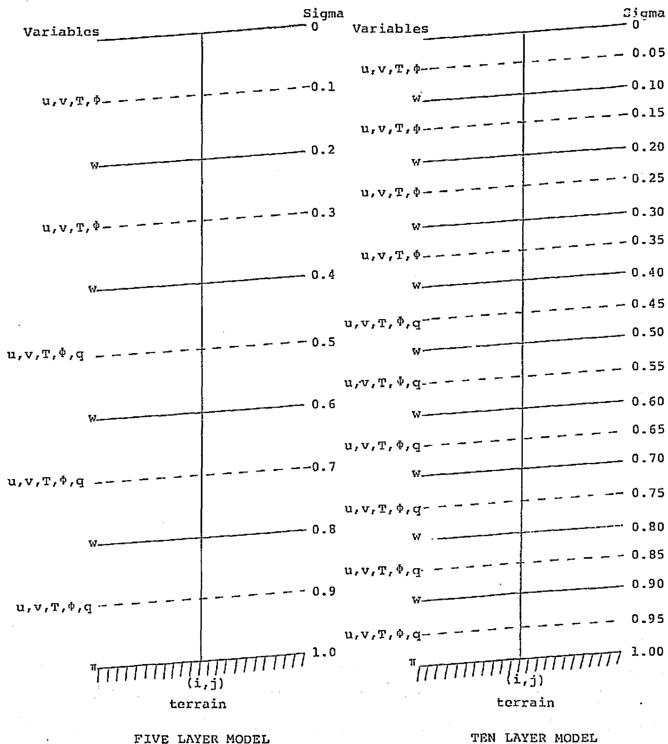
FIGURE II-1: DIAGRAM OF SIGMA SURFACES AND VARIABLES
