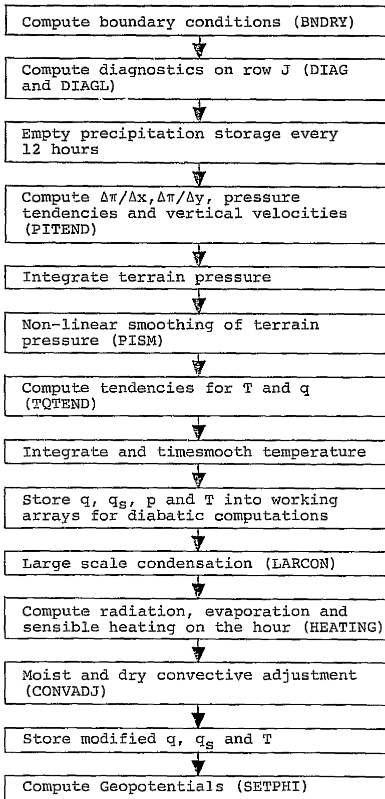
FIGURE III-11: COMPUTATION FOR ONE TIME STEP IN LSTEPP
