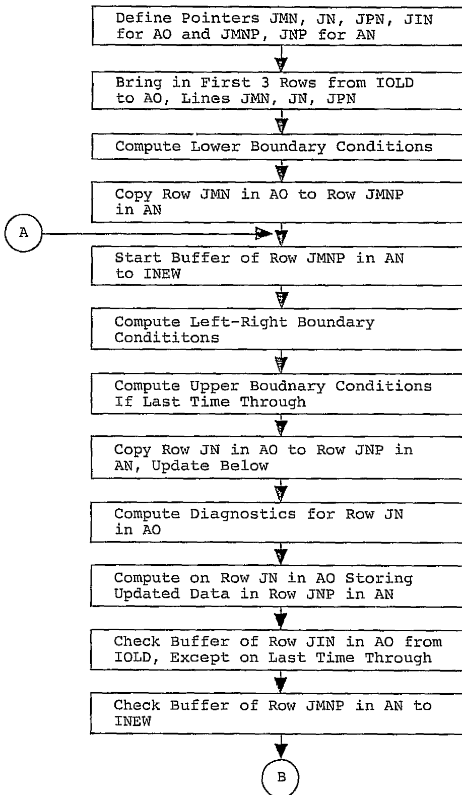
FIGURE III-3: DATA FLOW FOR ONE SWEEP OF THE DATA FILE - MODELS PECHCV AND PECHFV
