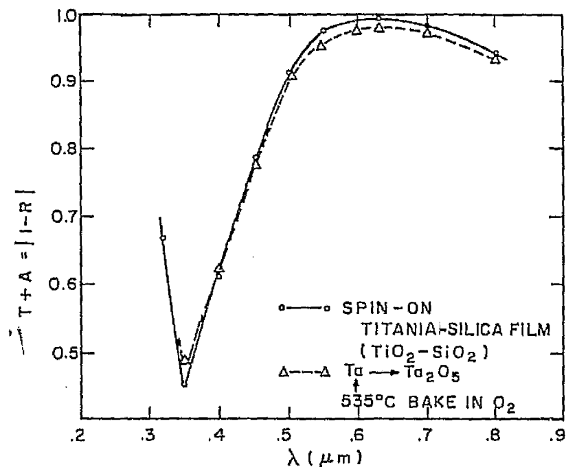
Figure 24. Reflection spectra: spin-on titania-silica film and Ta_2O_5 formed by thermal oxidation of evaporated Ta.
