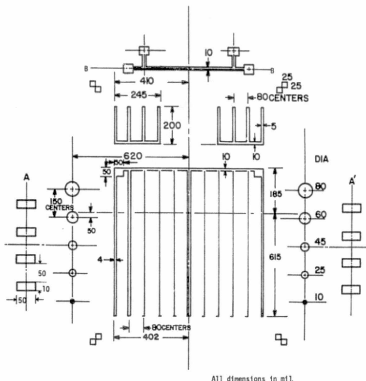
Figure 73. Solar cell mask design including diagnostic cells.
