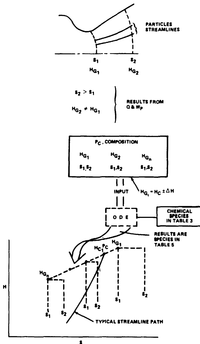
Figure 8. Schematic of thermochemistry table construction.
