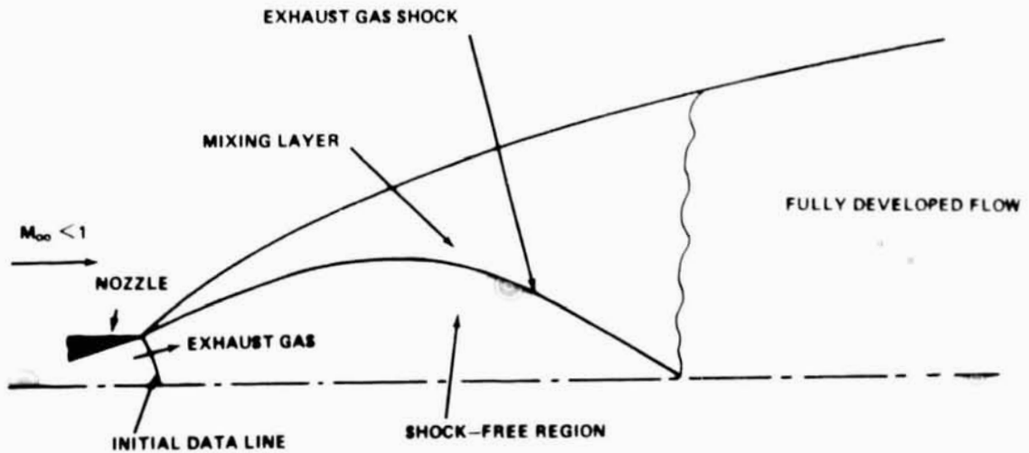
Figure 12. Plume afterburning schematic.
