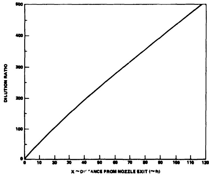
Figure 14. HARPOON booster afterburning analysis dilution ratio versus distance.
