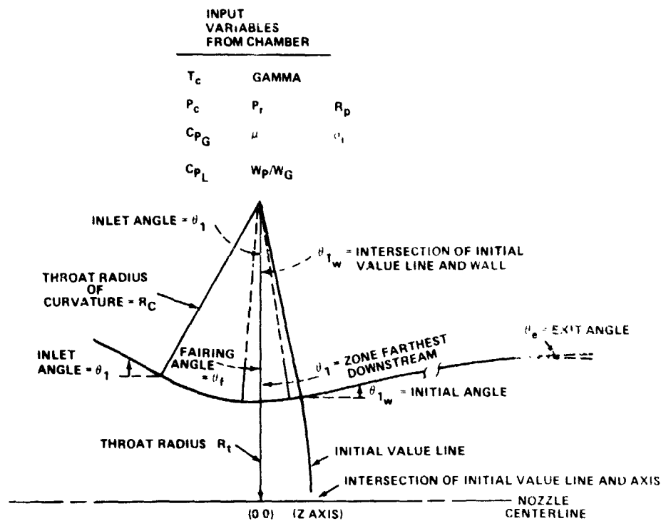
Figure 6. Nozzle parameters.
