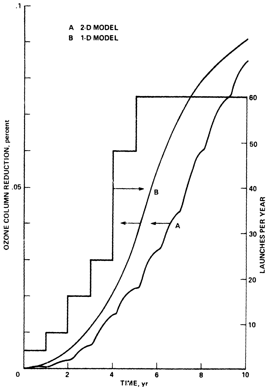
Figure C-1.- Time dependence of the globally averaged ozone reduction. Curve A - Ames 2-D model; curve B - an Ames 1-D model (the 1-D predicted ozone reduction after 20 years was approximately 0.11 percent). Also shown is a candidate Space Shuttle launch schedule.
