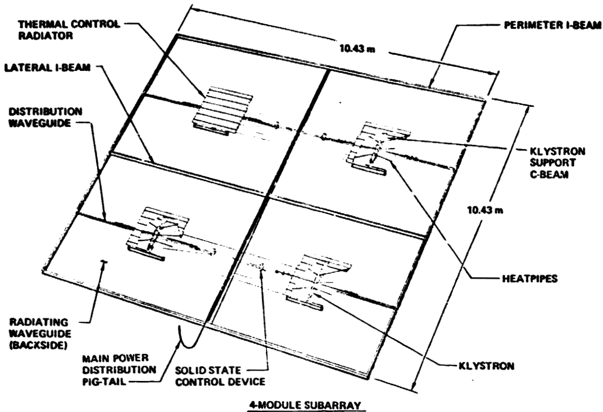
Figure 1.1.5-12 Reference MPTS-Integrated Subarray
