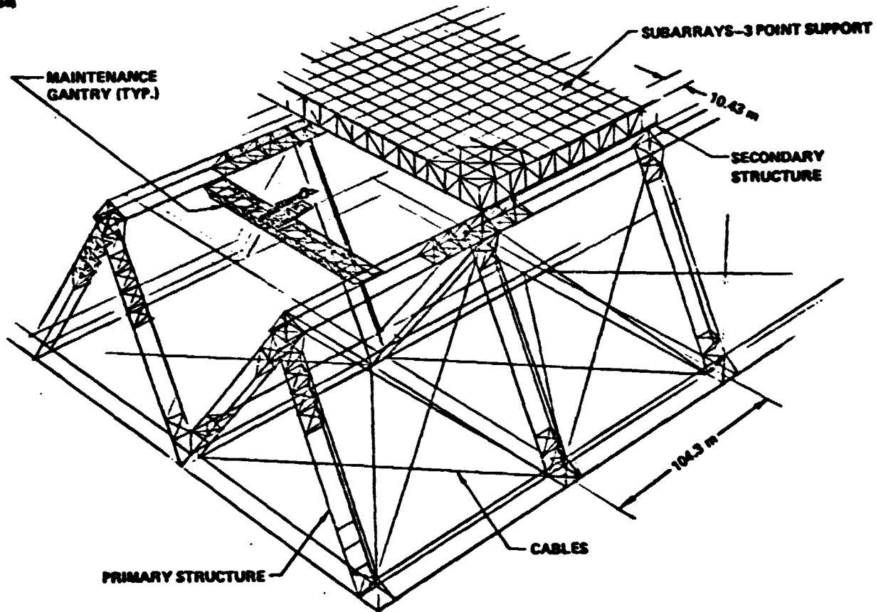
Figure 1.1.5-3 Reference MPTS Structure Interfaces
