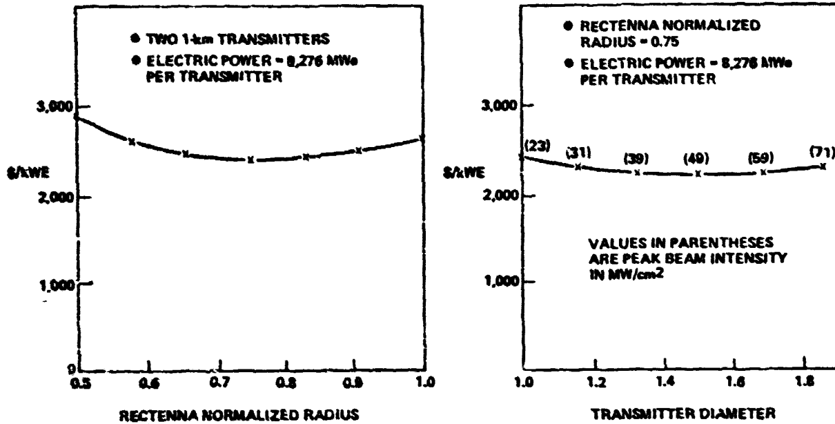
Figure A1-1 Size Sensitivity Results Power Transmission Optimization
