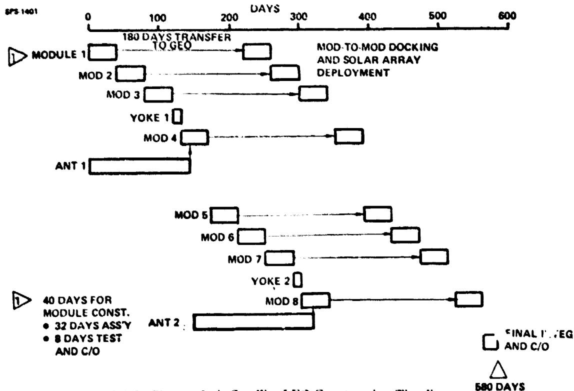
Figure 1.3.0-2 Photovoltaic Satellite LEO Construction Timeline
