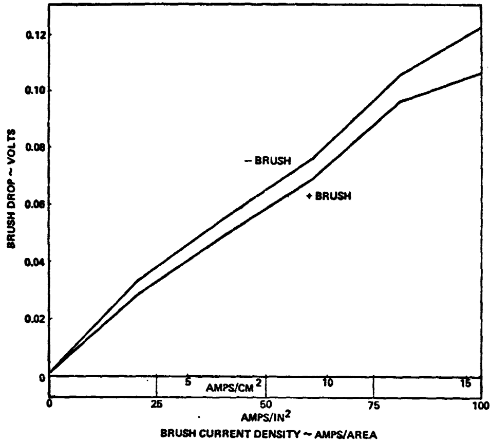
Figure 1.1.4-10 Sliver Slip-Ring Grade 26 Brush 85 Ag 3 GR 12 Mo S 2
