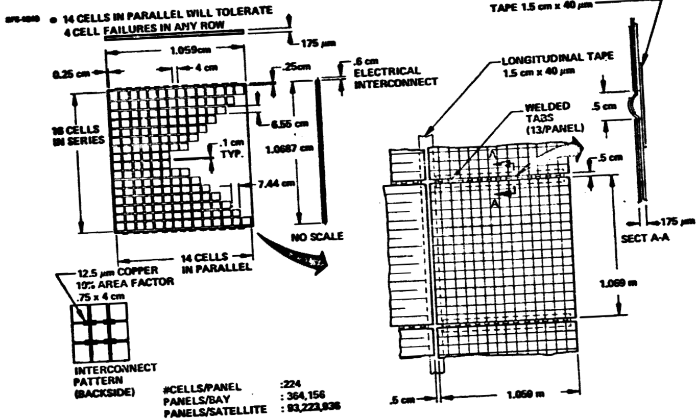
Figure 1.1.3-2 Array Blanket Description
