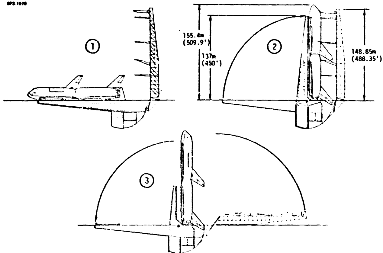
Figure 1.4.1-7 Launcher/Erector Concept
