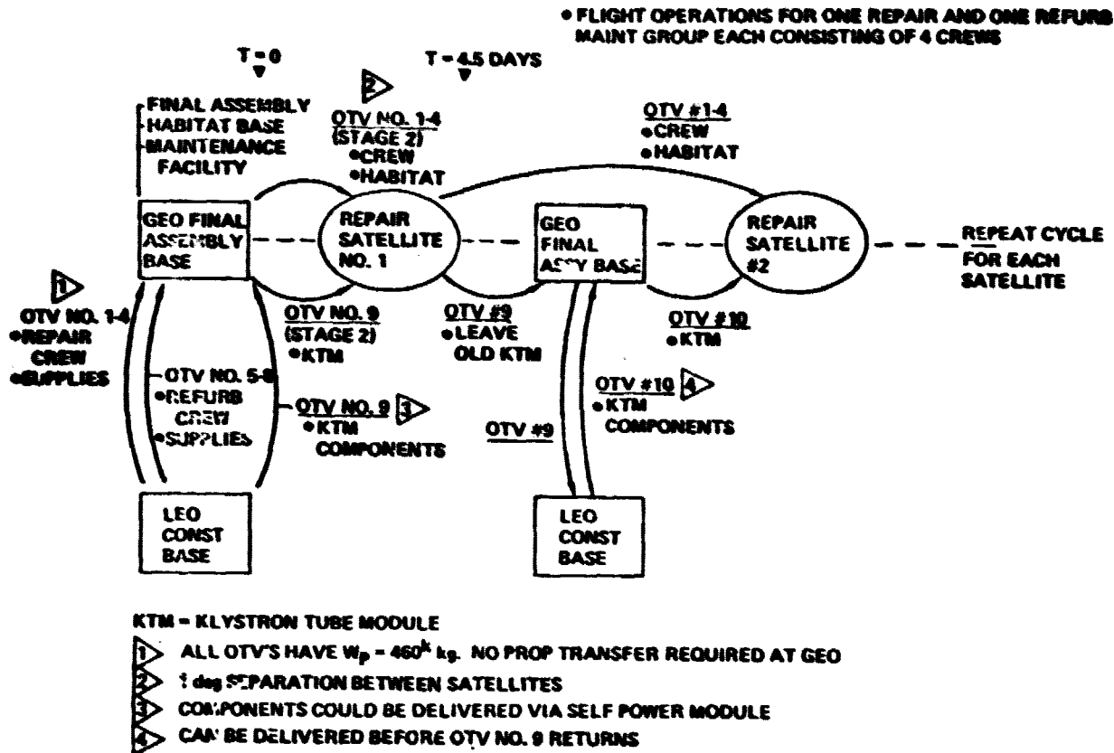
Figure 1.3.3-1 Selected Maintenance Mission Concept
