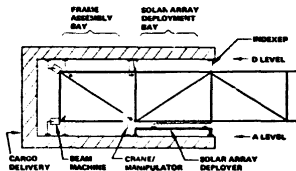
Figure 1.3.1-1 LEO Construction Base Photovoltaic Satellite
