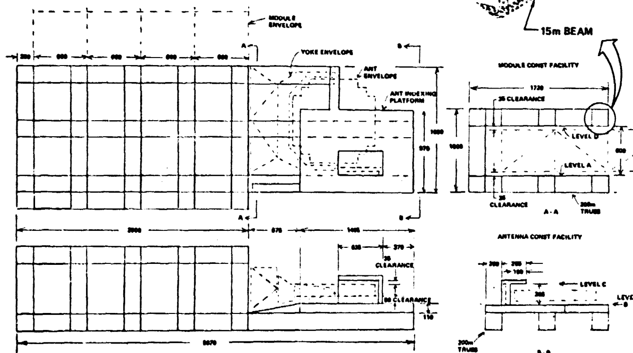
Figure 1.3.1-9 LEO Construction Base
