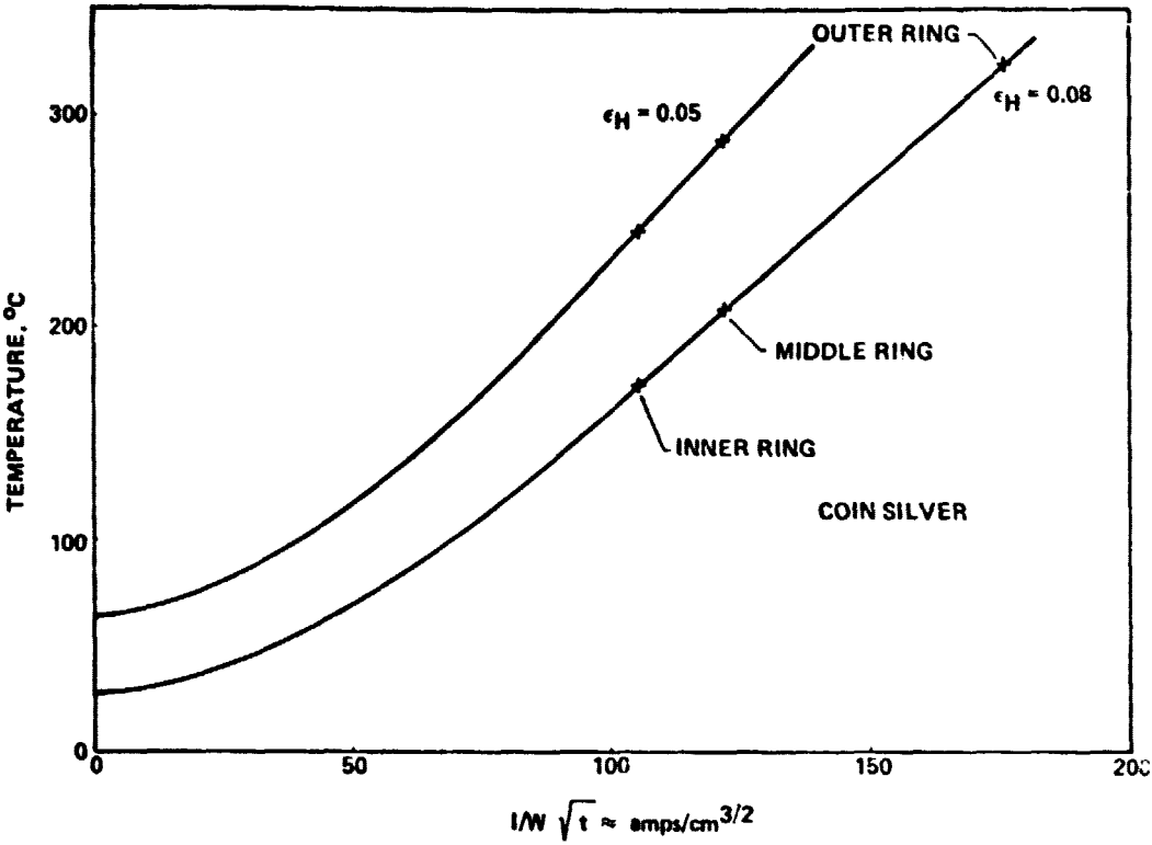
Figure 1.1.4-12 Slip-Ring Temperatures
