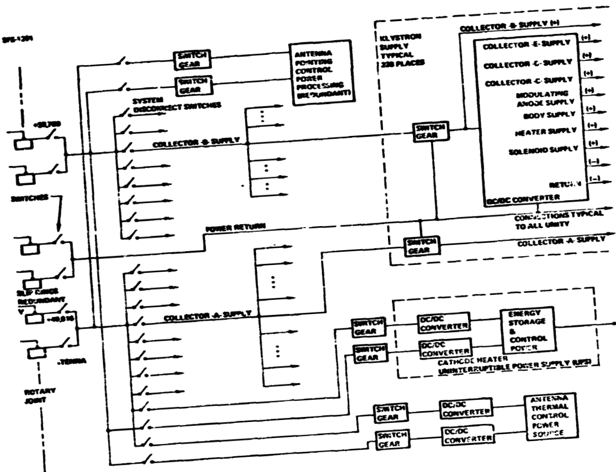
Figure 1.1.5-7 MPTS Power Conditioning Subsystem
