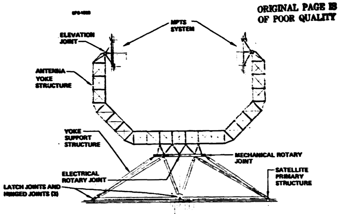
Figure 1.1.1-9 Antenna Yoke and Turntables
