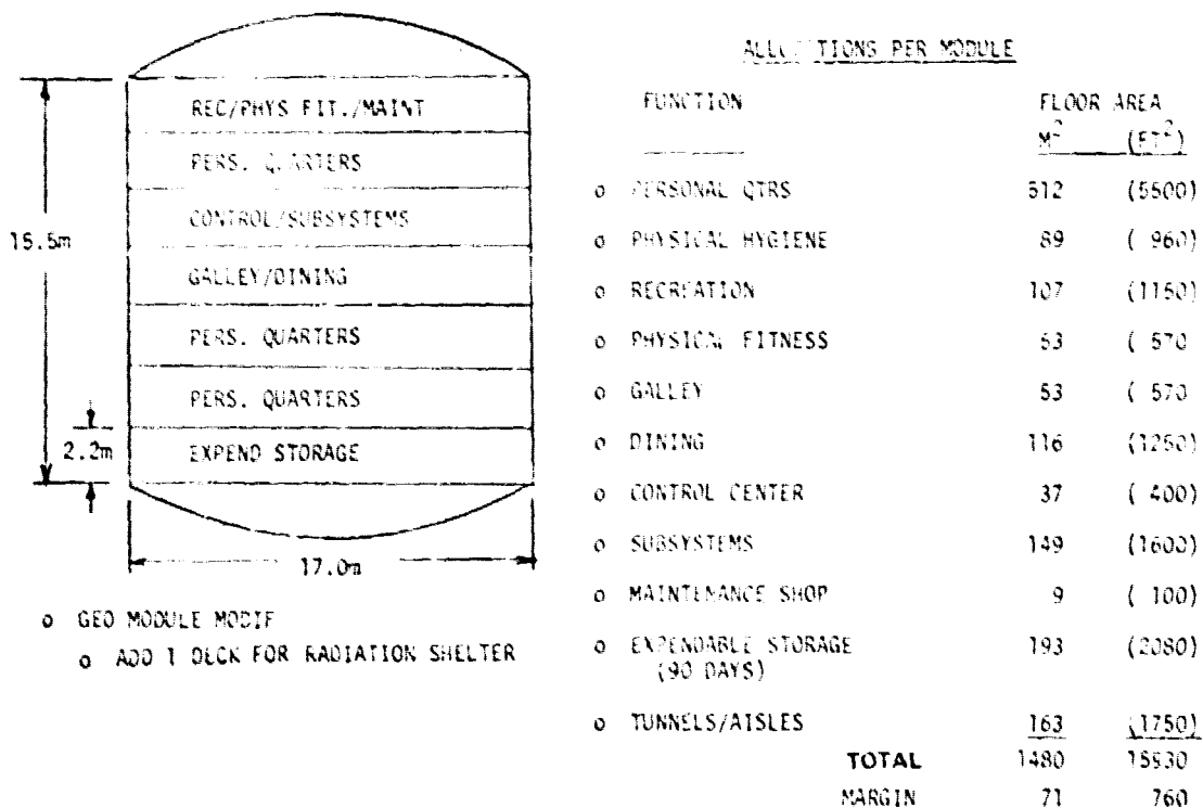
Figure 1.3.1-10 Crew Quarters Sizing
