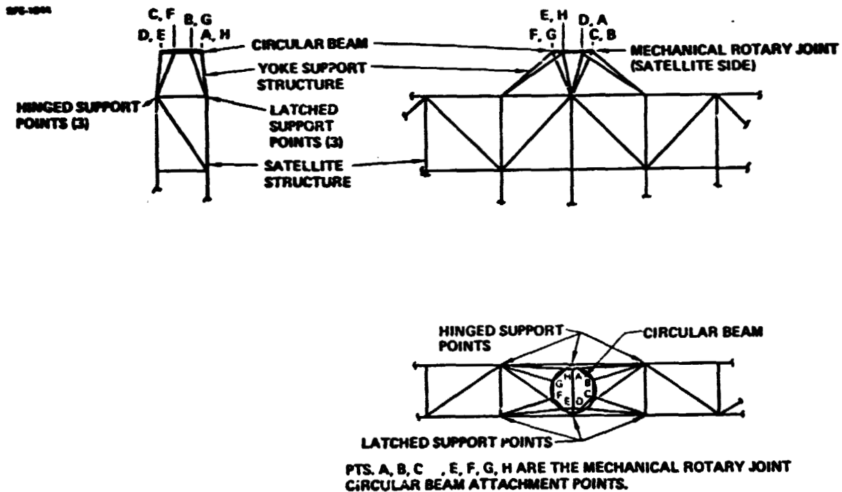
Figure 1.1.1-10 Yoke Support Structure
