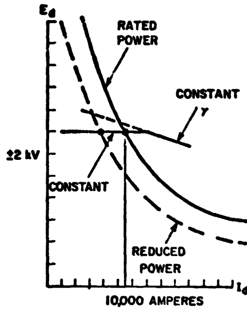
Figure 1.2.4-10 Converter Characteristic
