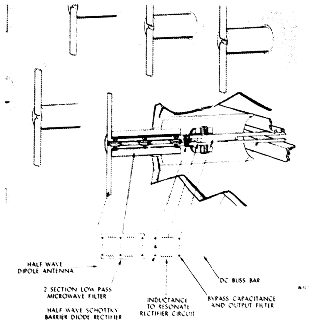
Figure 1.2.4-1. Cutaway section of the three-plane rectenna approach used in the RXCV at JPL's Goldstone facility showing how the rectenna elements plug into the array. Although this approach was satisfactory electrically, it is complicated from a fabrication point of view. A greatly simplified mechanical approach is the two-plane system which preserves all of the desirable electrical properties of the three-plane system.
