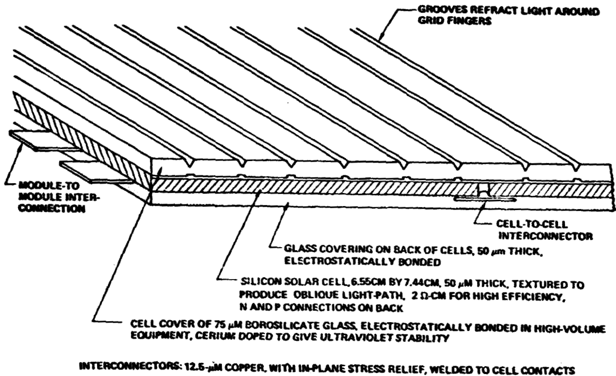
Figure 1.1.3-1 Solar Array Blanket
