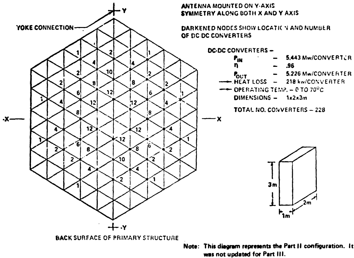
Figure 1.1.5-6 MPTS Reference Antenna Power Conditioning Placement
