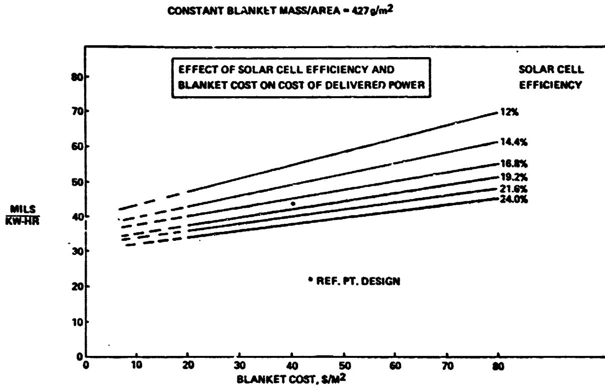
Figure A1-3 Busbar Cost of Power Relatively Insensitive to Solar Blanket Cost and Efficiency
