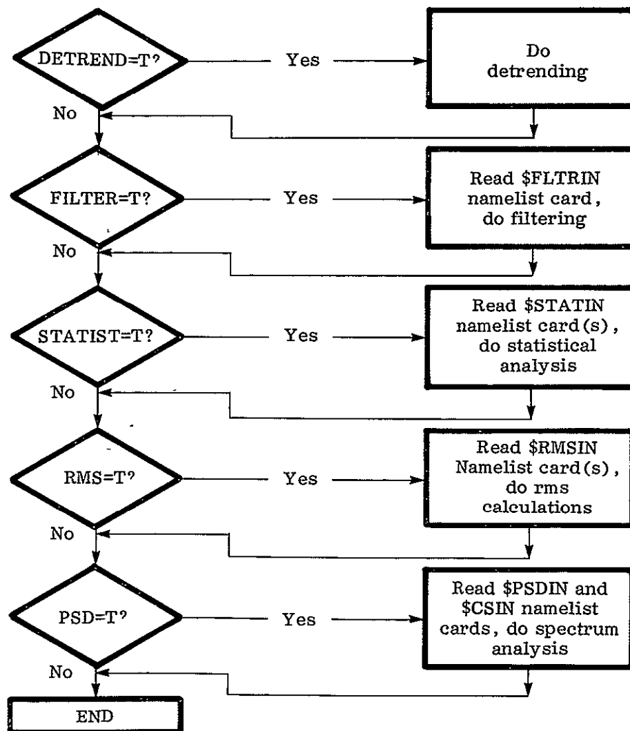
Figure 2. $SCARDIN namelist.
