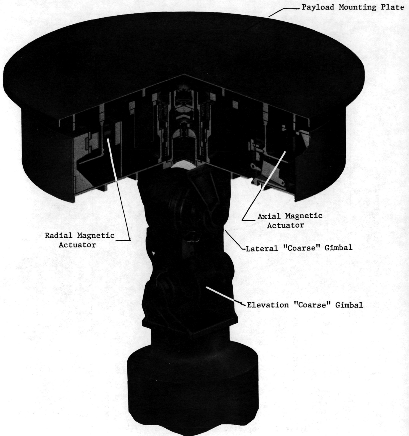
Figure 1. Annular Suspension and Pointing System (ASPS).
