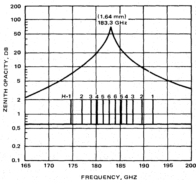
FIGURE 2. H 2 O SOUNDING CHANNELS H-1 TO H-6
